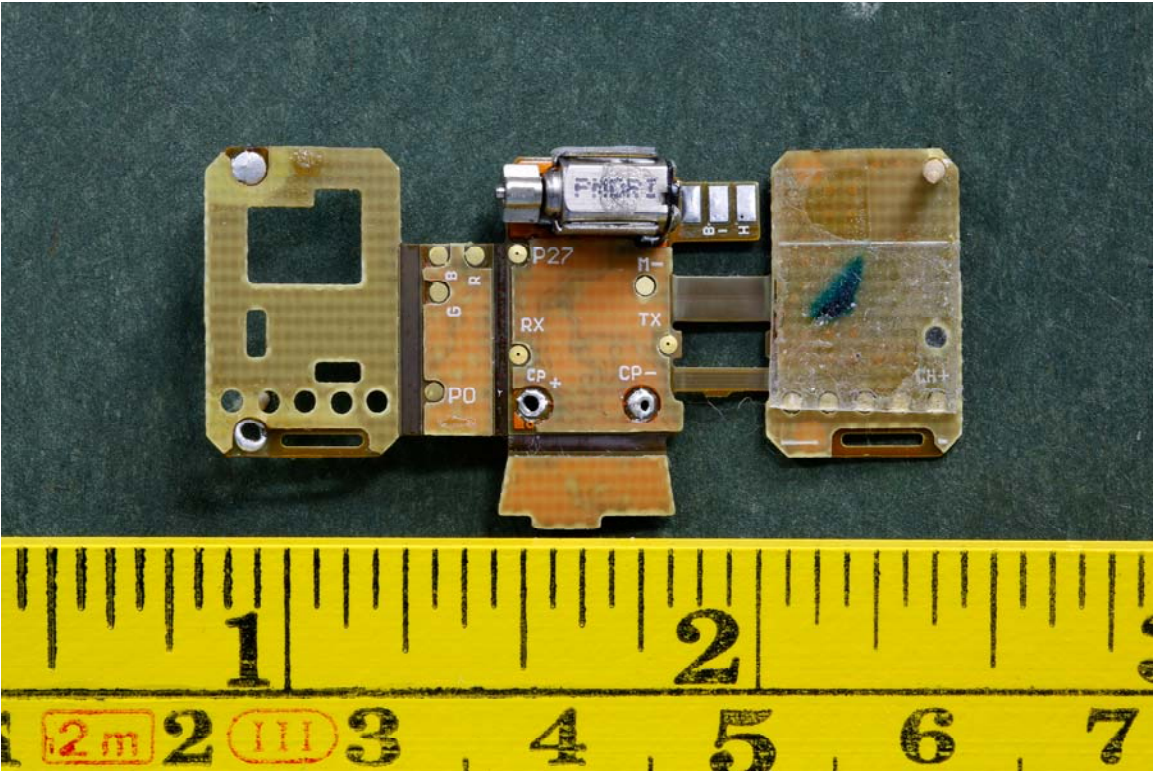
PCB Rear
