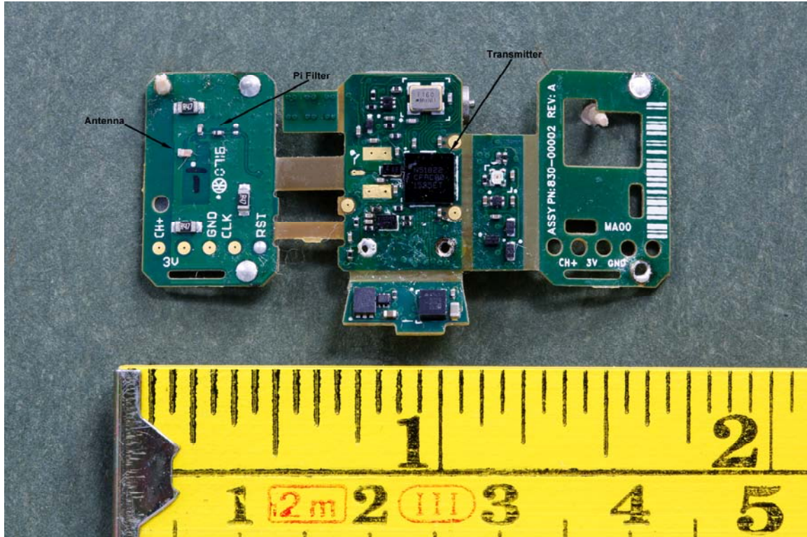
PCB Front
