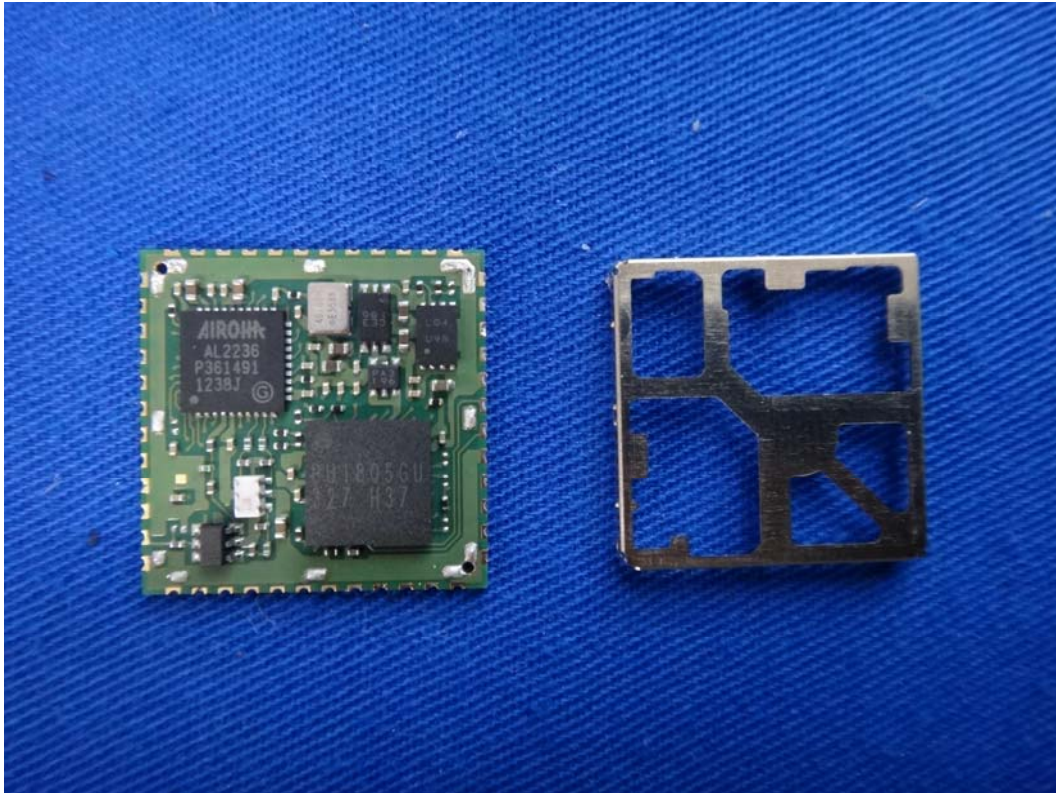
(7) EUT Photo
