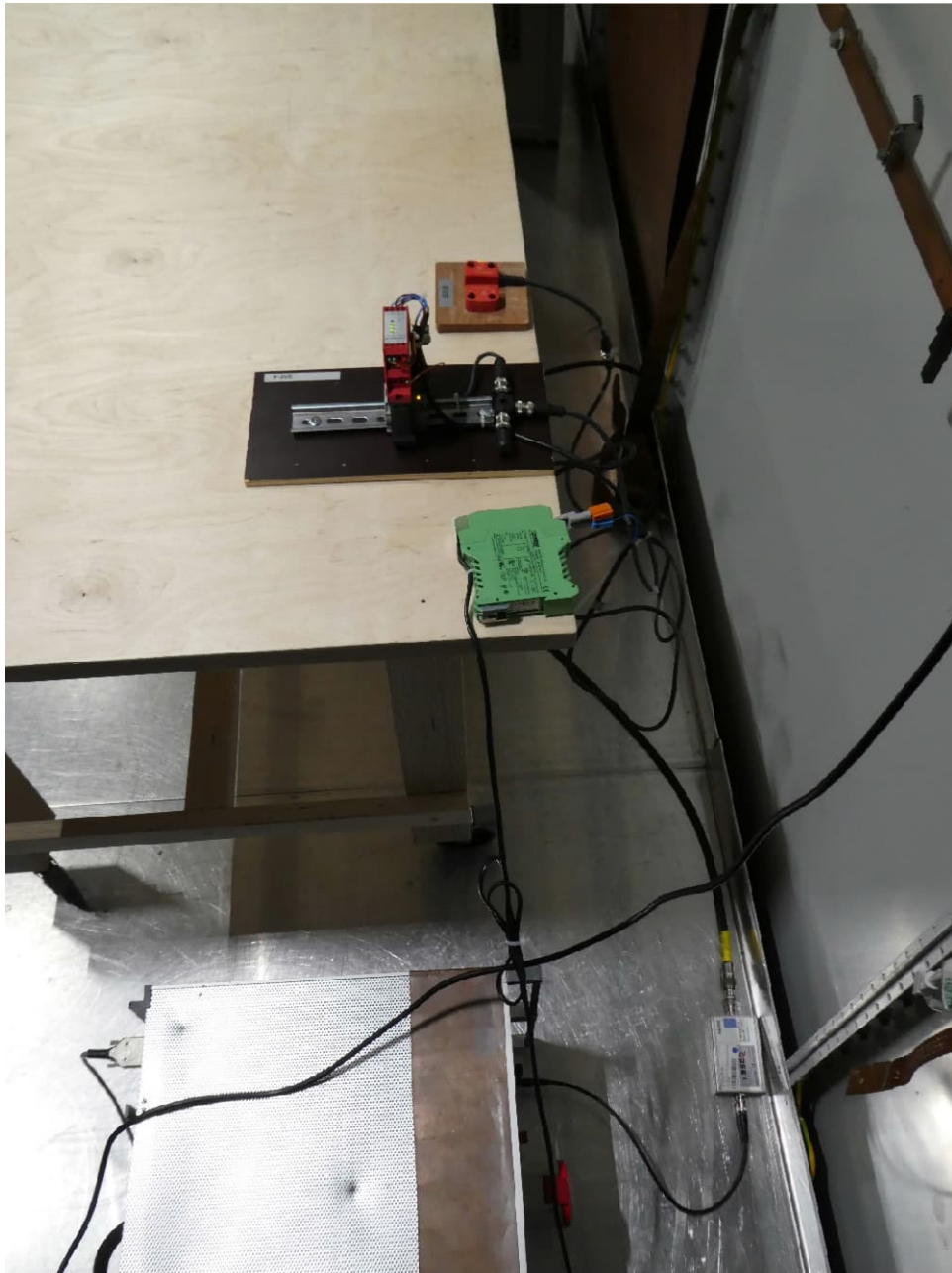
Test setup AC power line conducted emissions EUT 2
