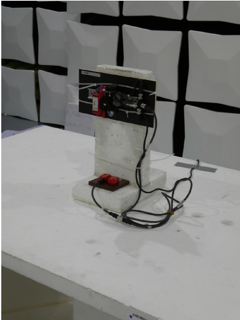
Test setup semi anechoic chamber EUT 2
