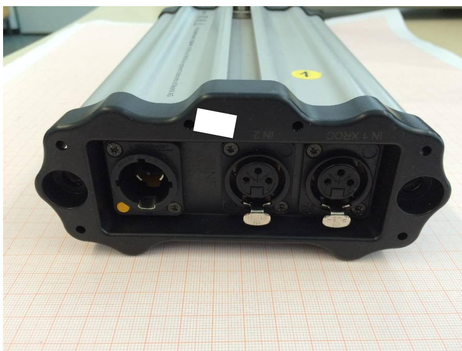
Photo 6 (bottom view):
