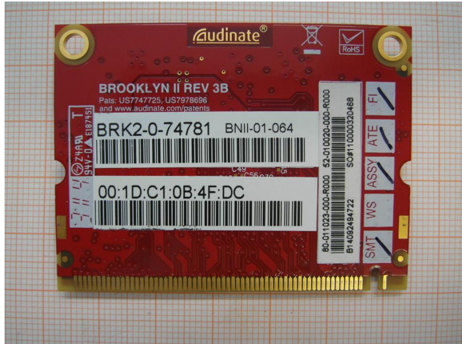
Photo 13 (Audio board with DSP – rear view):
