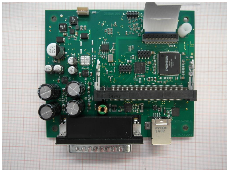
Photo 14 (interface board – top view):
