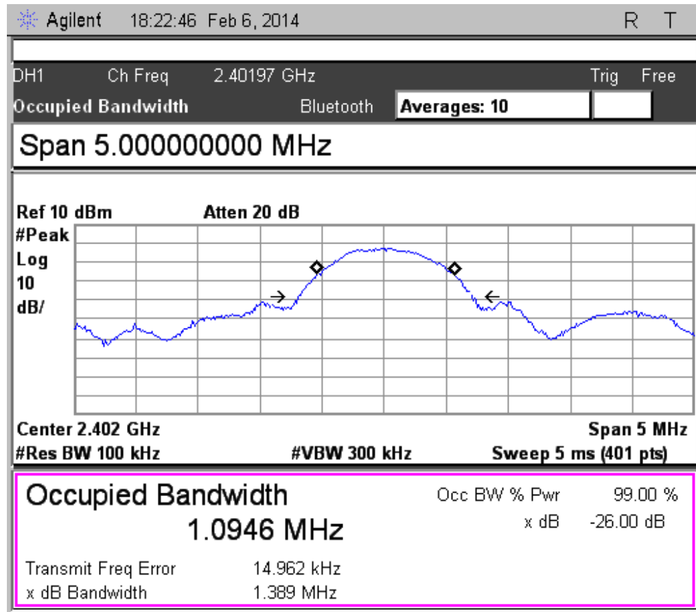
Figure 41: Occupied Bandwidth Measurement – Channel no 37
