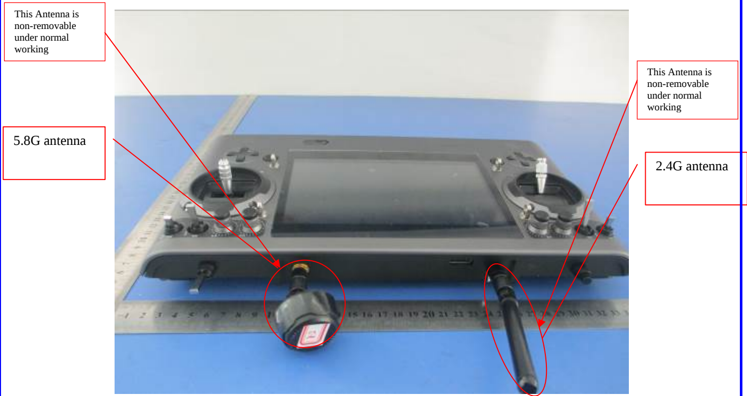
EUT - Top View
