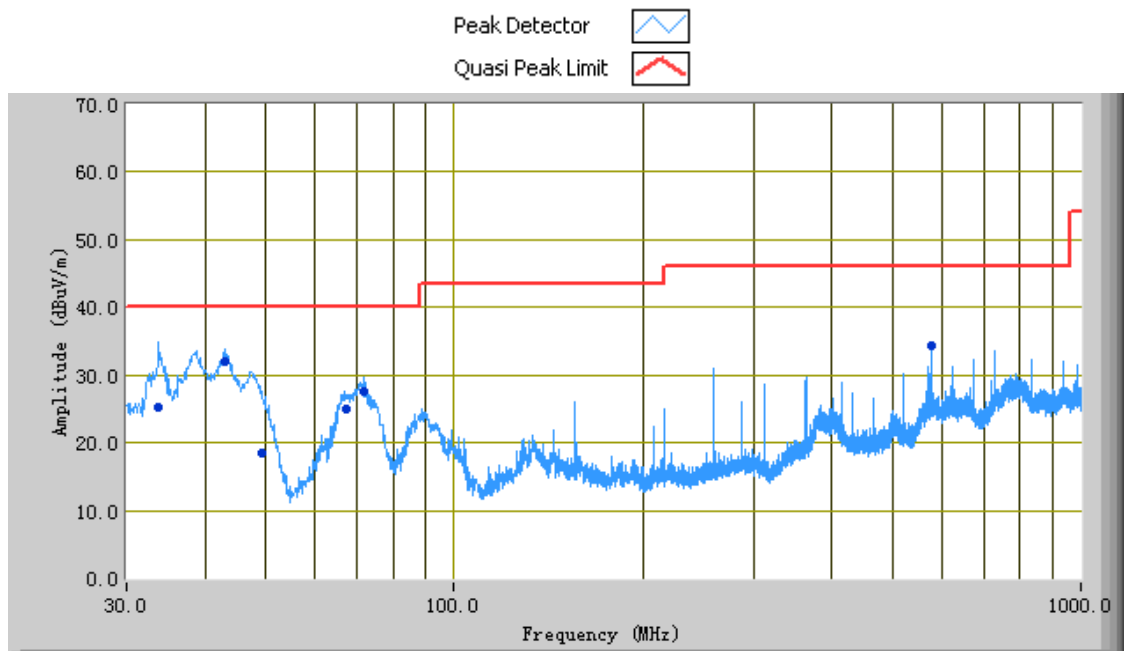
Vertical Polarity Plot @3m
