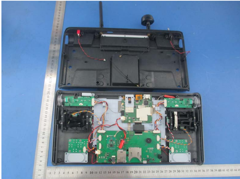
Cover Off – Front View 1
