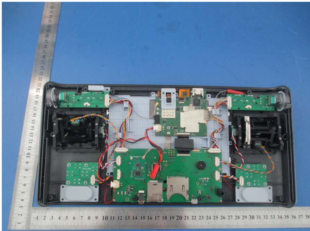
Cover Off – Front View 2
