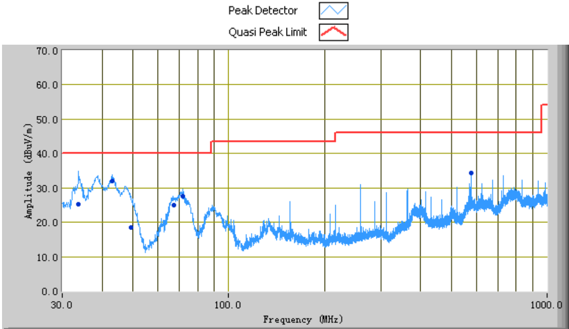
Horizontal Polarity Plot @3m
