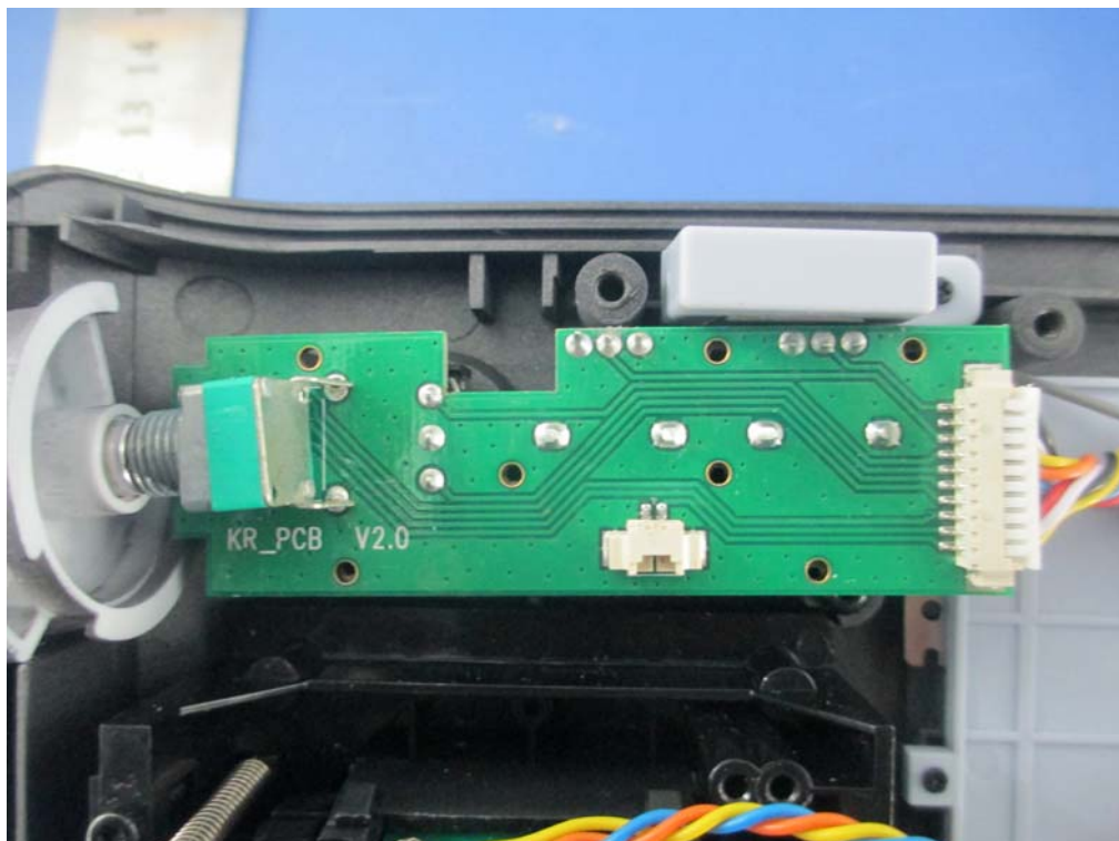
PCB 5 - Top View
