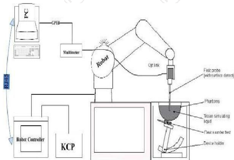
KUKA SAR Test Sysyem Configuration
