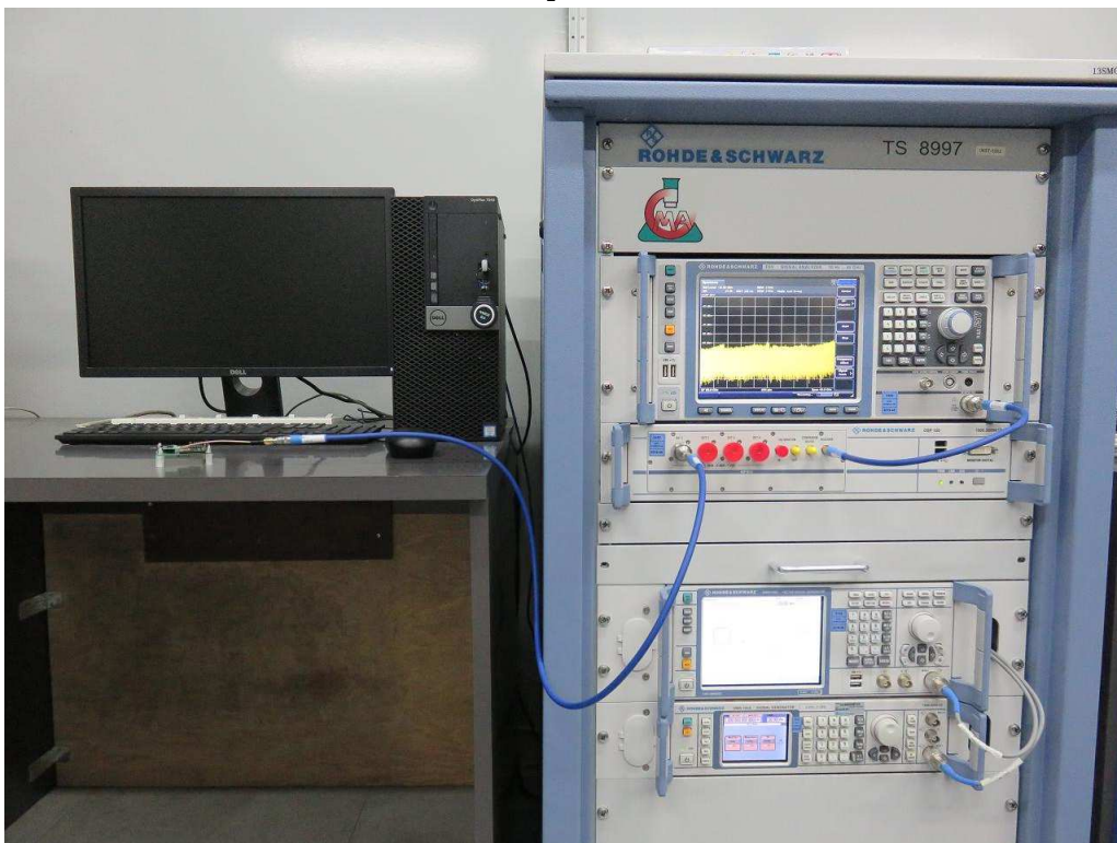
Conducted emission
