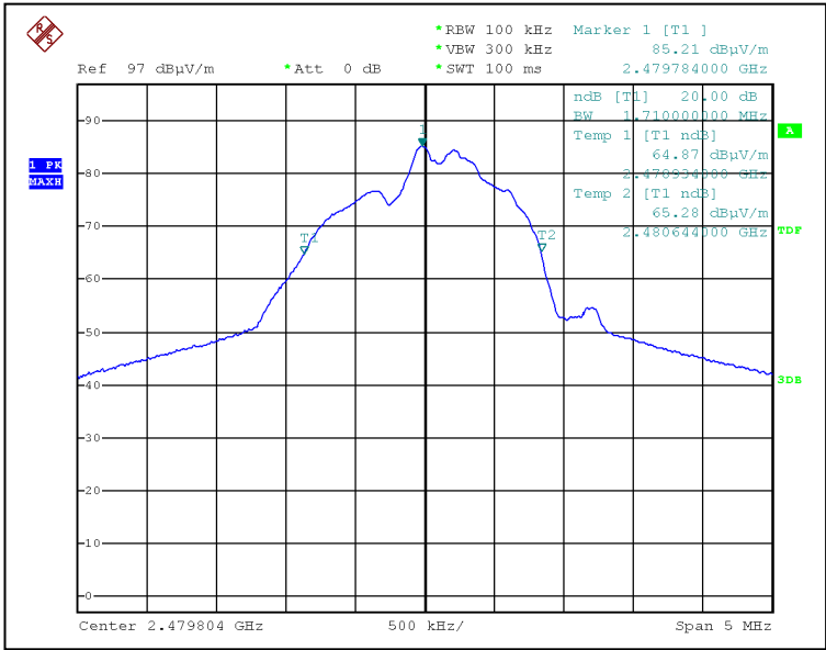
Bandwidth 3 (2480MHz)
