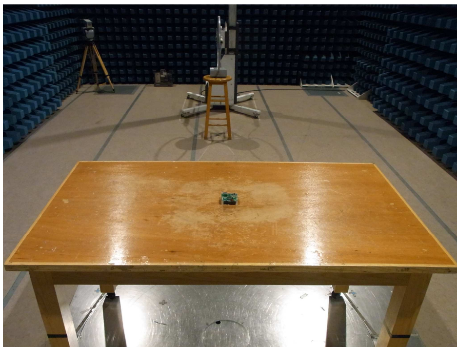
Rear view (30MHz – 1GHz)
