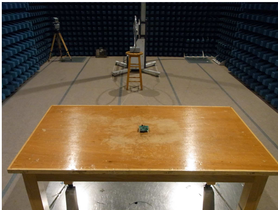
Front view (30MHz – 1GHz)
