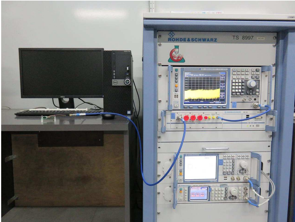
Conducted emission
