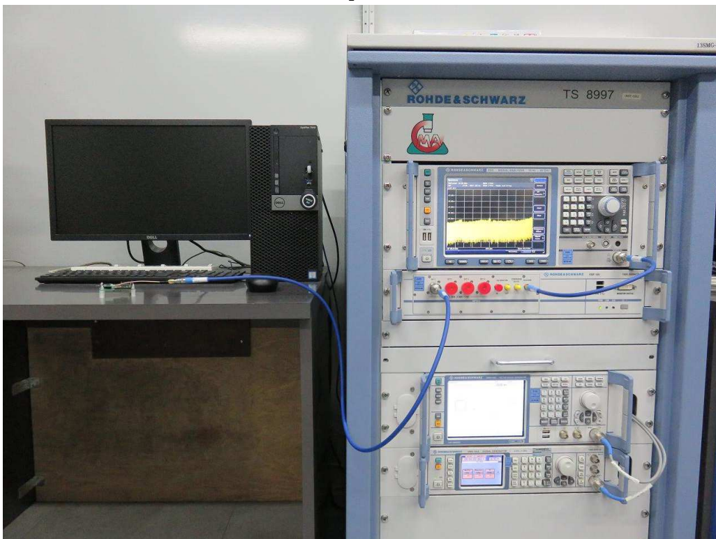
Conducted emission
