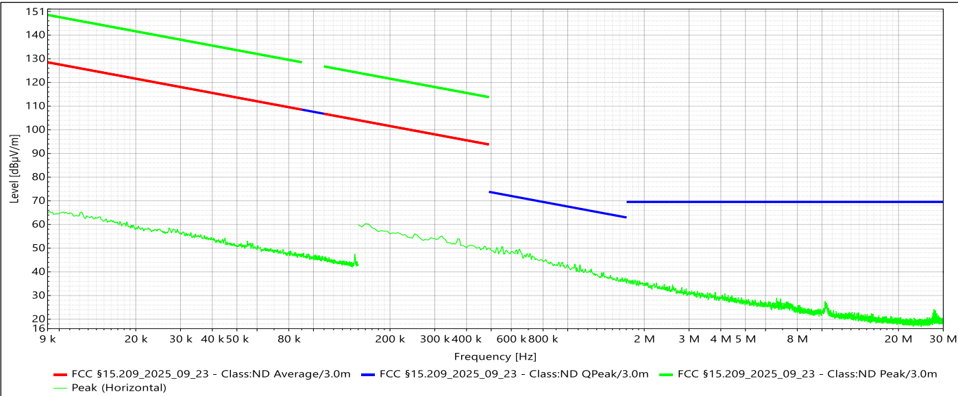
Figure 2.3.7-6 – Radiated Emissions Test Results
