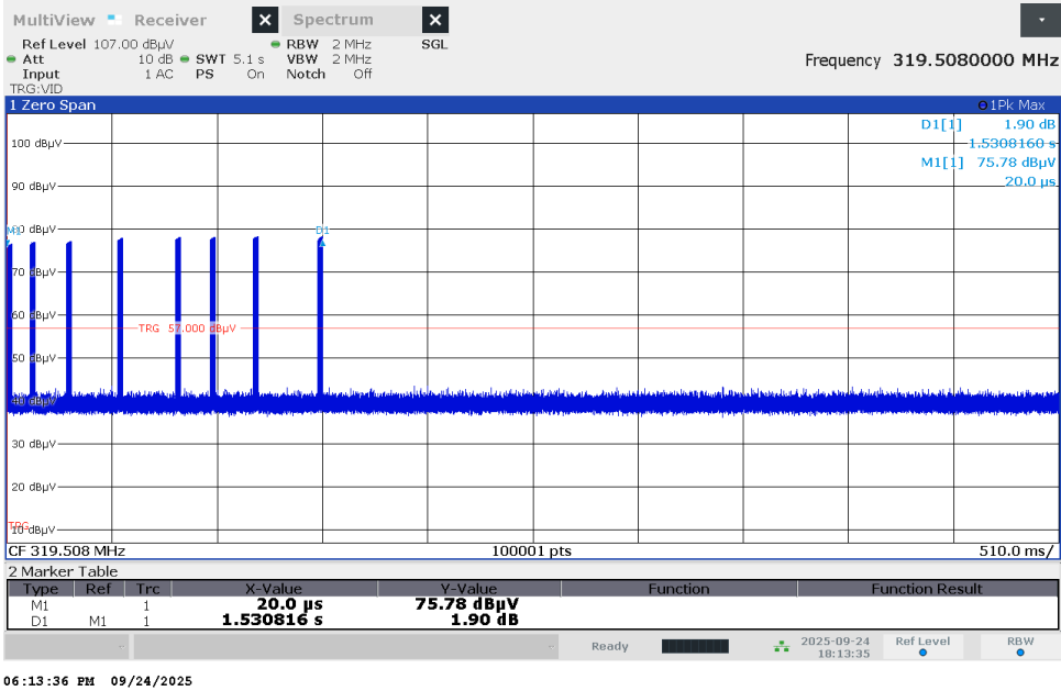
Figure 2.2.6-1 – Transmitter Deactivation Time Test Results
