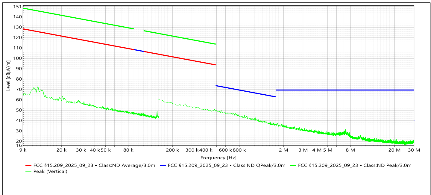
Figure 2.3.7-4 – Radiated Emissions Test Results
