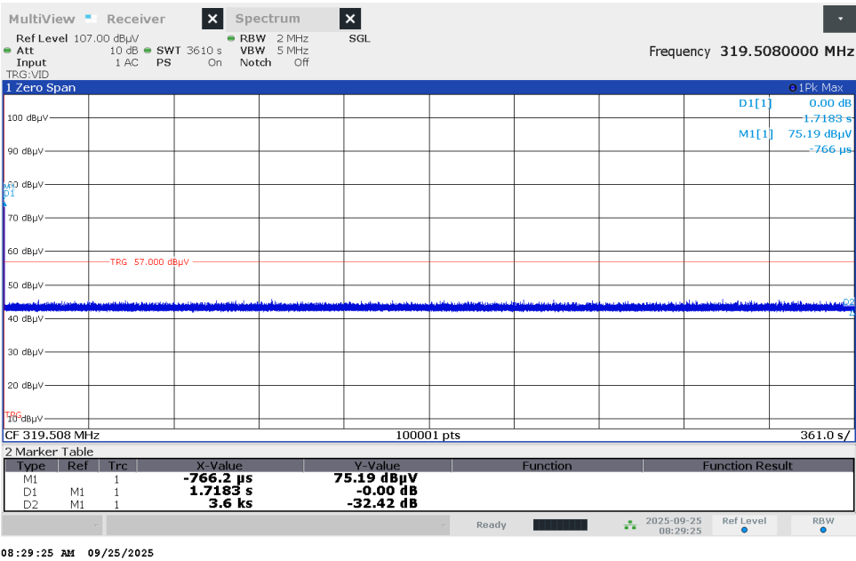
Figure 2.2.6-2 – Timing Measurement Test Results – Maximum Transmission Over One Hour
