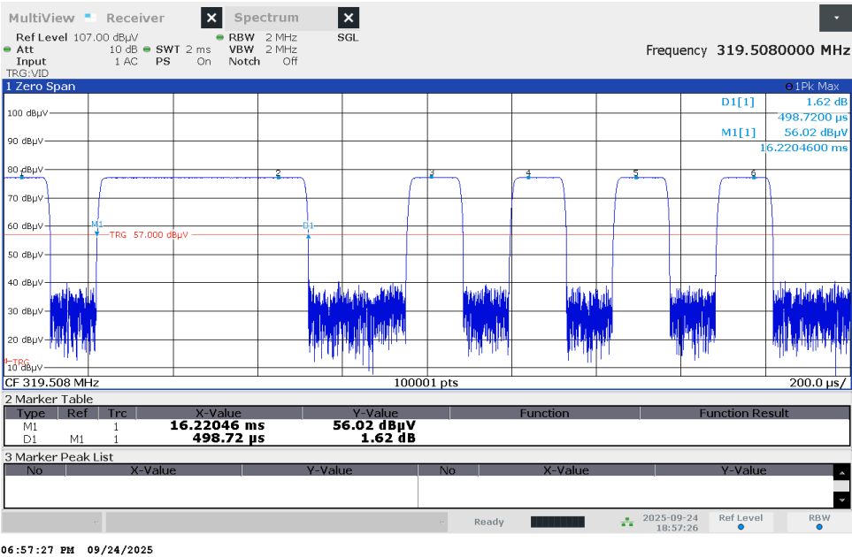
Figure 2.2.6-6 – Pulse Width Test Results
