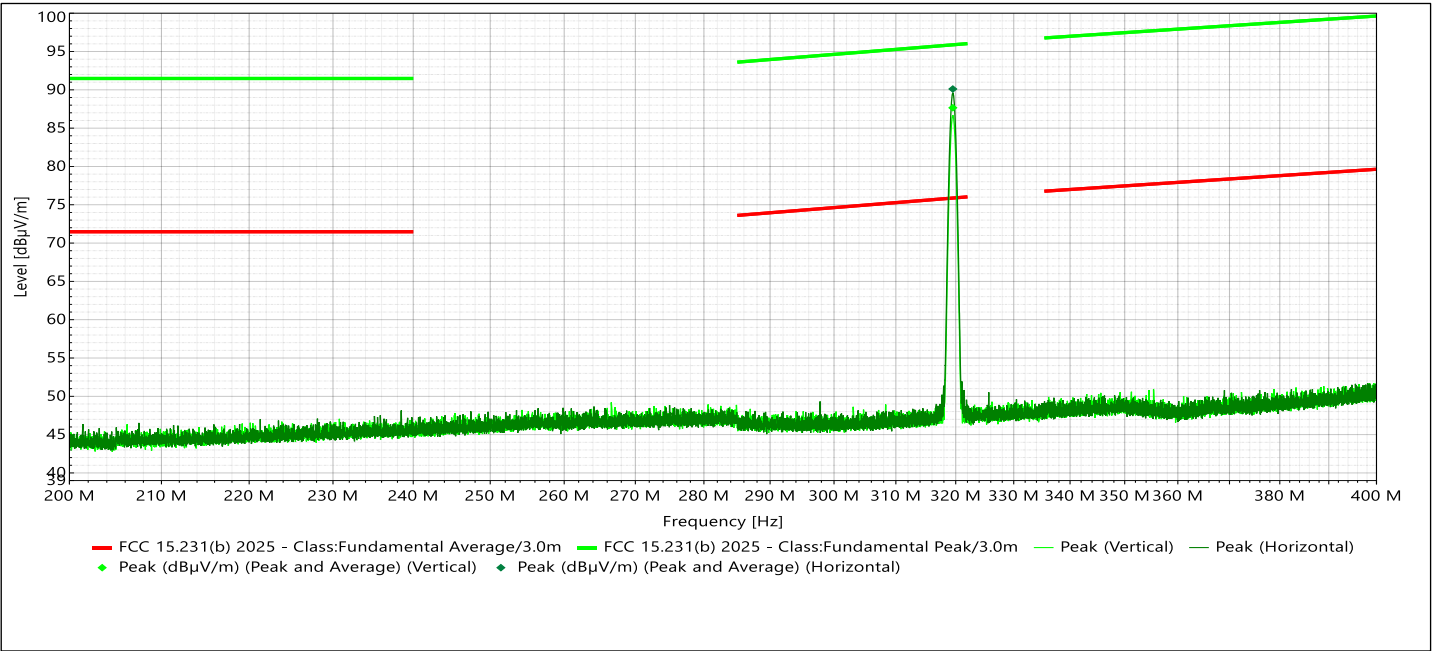
Figure 2.3.7-2 – Radiated Emissions Test Results
