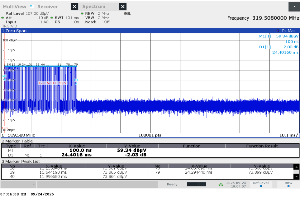
Figure 2.2.6-3 – Transmitter Duty Cycle – Number of Packets
