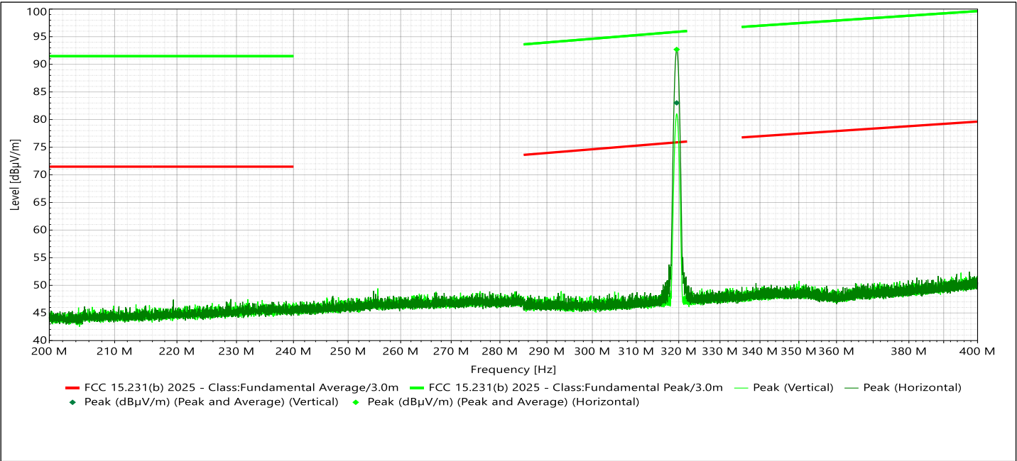
Figure 2.3.7-1 – Radiated Emissions Test Results
