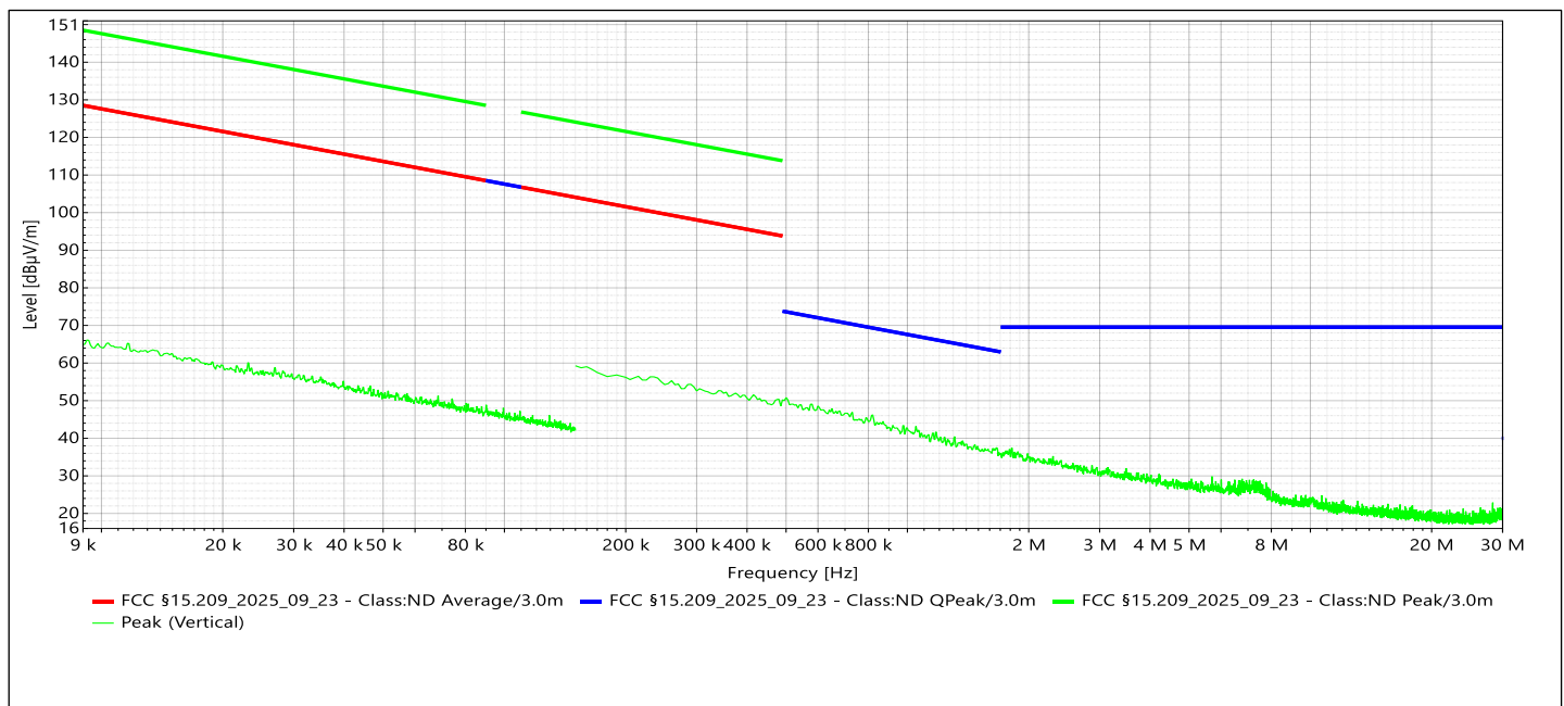
Figure 2.3.7-5 – Radiated Emissions Test Results
