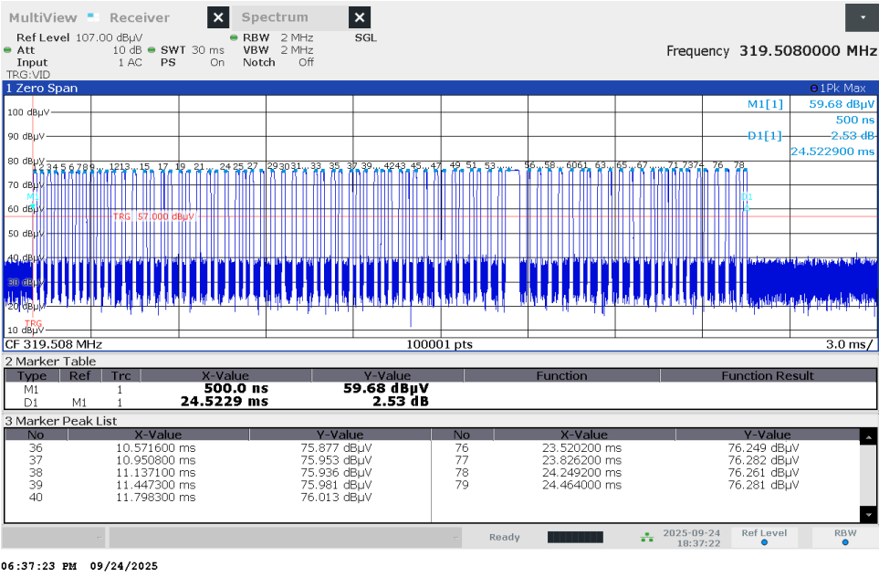
Figure 2.2.6-4 – Total Number of Pulses Test Results / Packet Length
