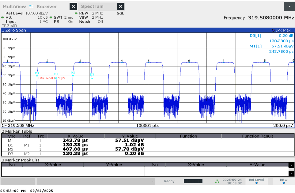
Figure 2.2.6-5 – Pulse Width Test Results
