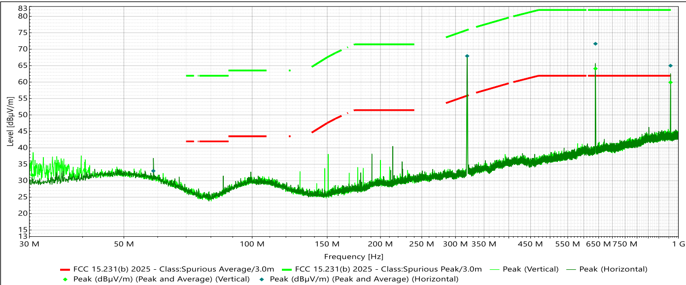
Figure 2.3.7-7 – Radiated Emissions Test Results
