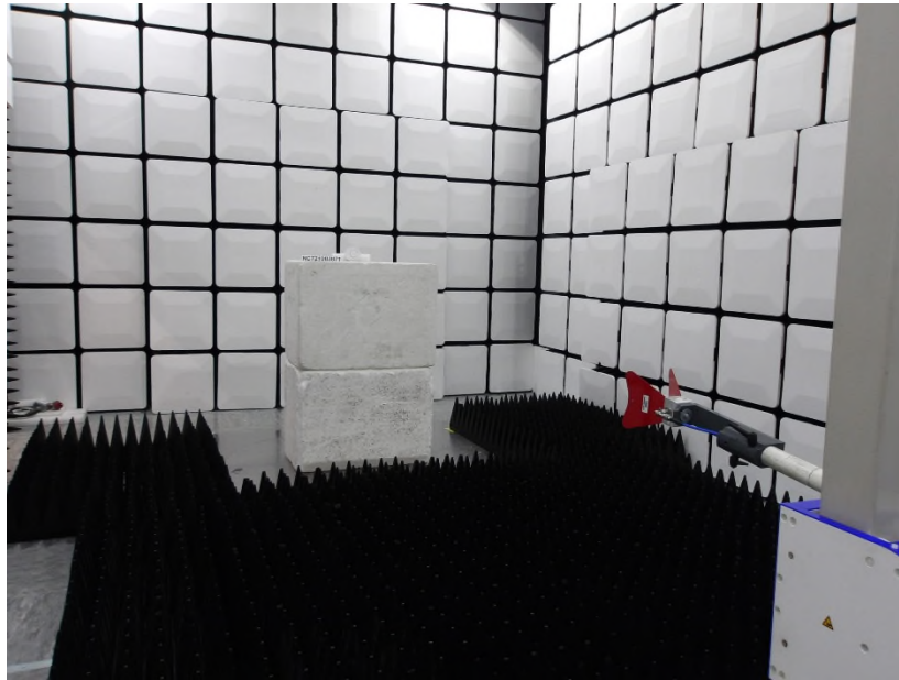
Photo 1.5-3 – Radiated Spurious Emission 1G-18G Test Setup Photo [Front View]
