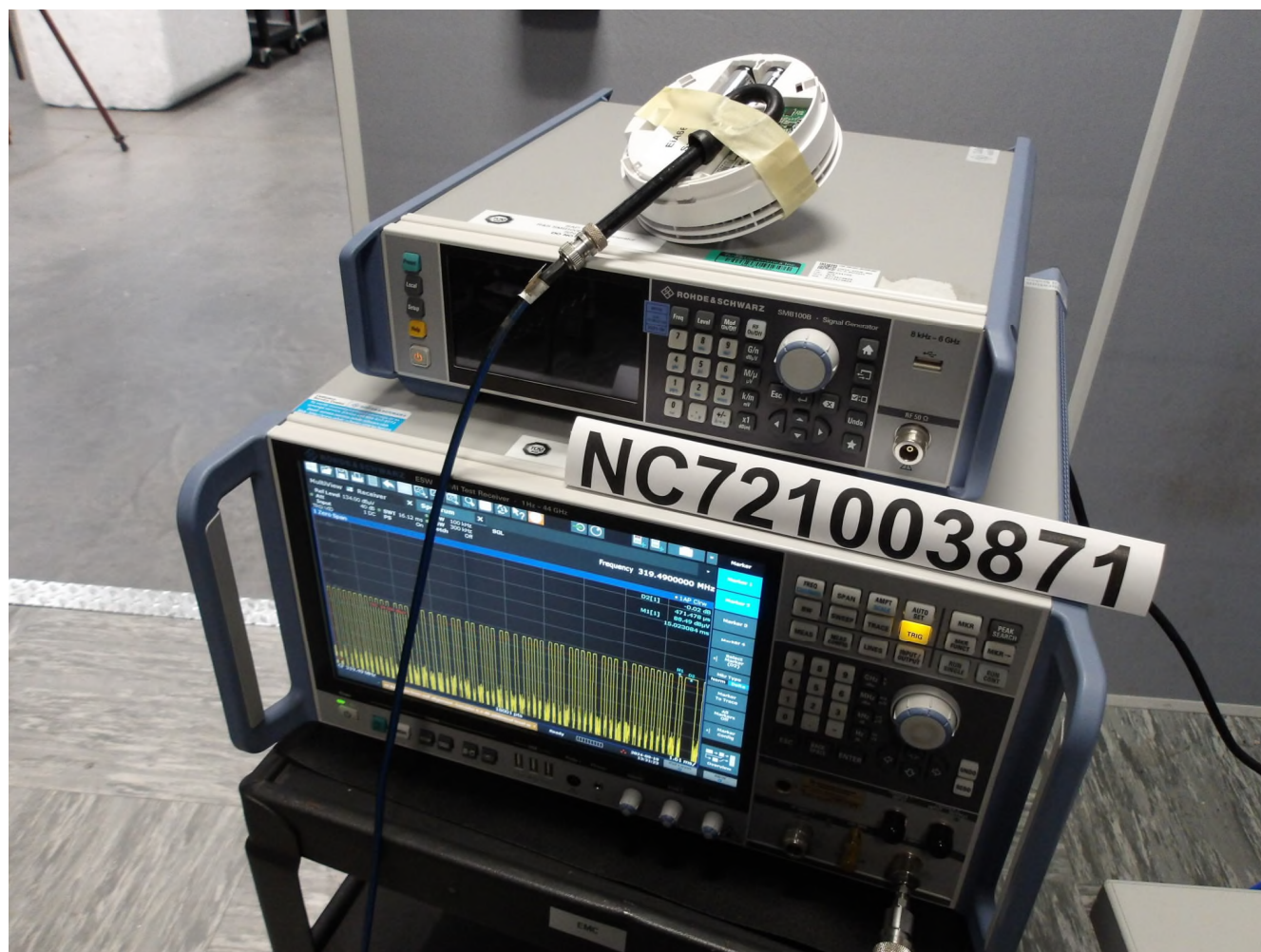
Photo 1.3-1 – Pulse Polling or Supervision Transmissions & Duty Cycle of Transmitter Test Setup Photo [Front View]
