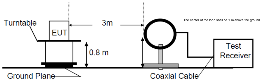
Diagram of Measurement Configuration for Radiation Test (Below 1GHz)
