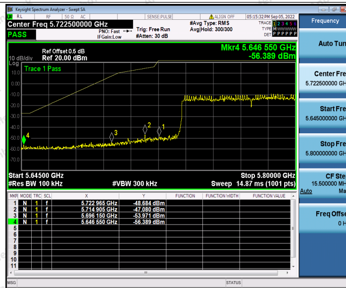
11AX80SISO_Ant1_High_5775
