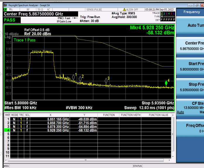
11AX20SISO_Ant2_High_5825
