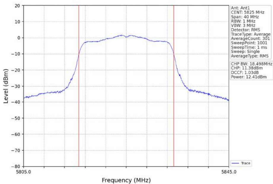
802.11ac(VHT20)_HCH_5825MHz_Ant1_NTNV
