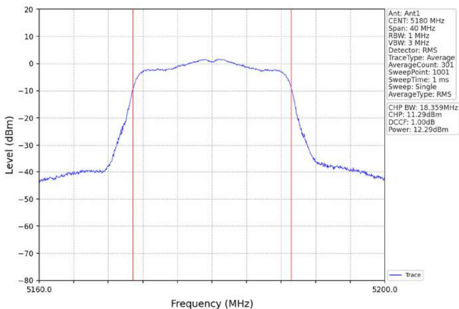
802.11ac(VHT20)_LCH_5180MHz_Ant1_NTNV
