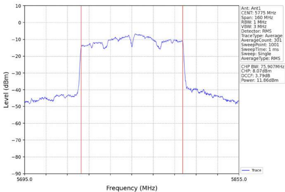
802.11ac(VHT80)_MCH_5775MHz_Ant1_NTNV
