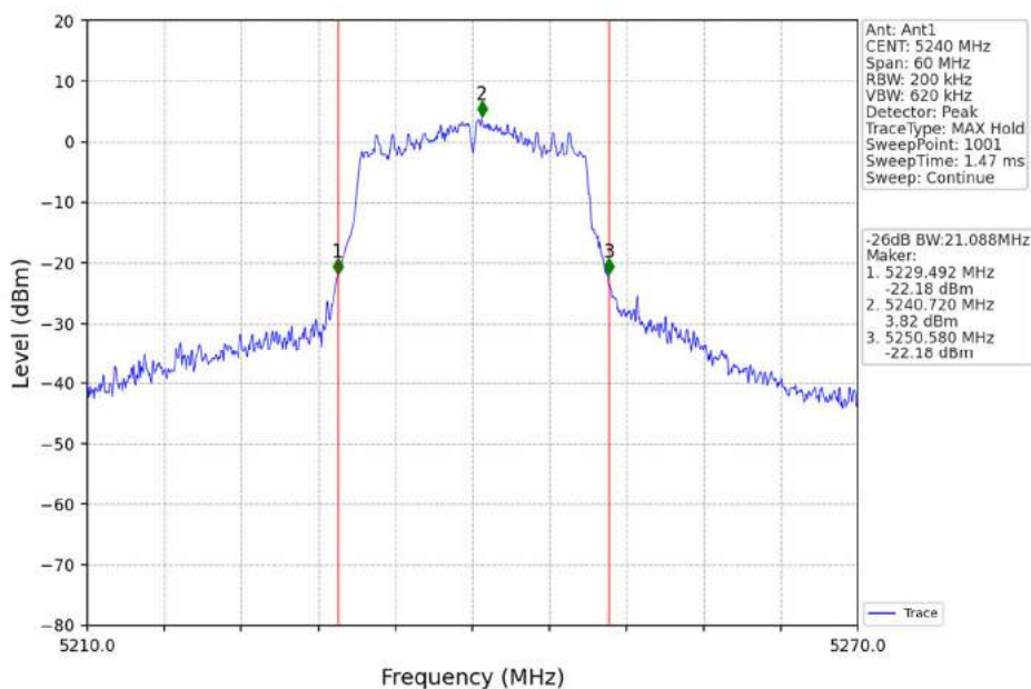
802.11ac(VHT20)_HCH_5240MHz_Ant1_NTNV
