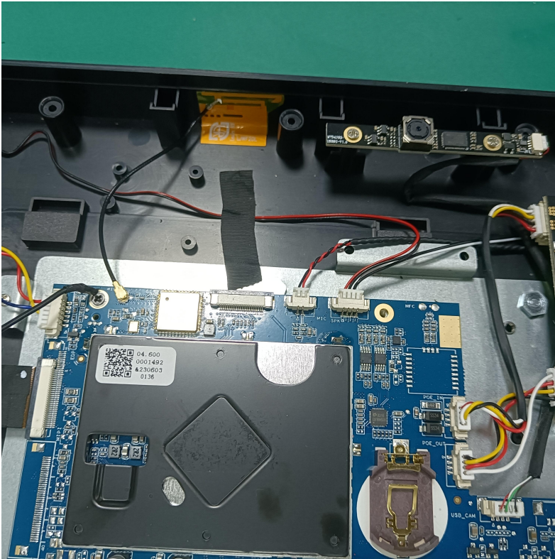
WIFI Antenna
