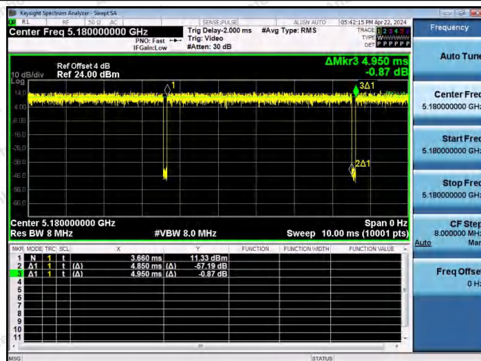
NTNV-11AX20MIMO-Ant1-5180
