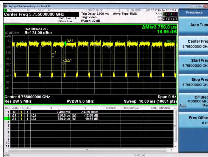
NTNV-11N40MIMO-Ant2-5755
