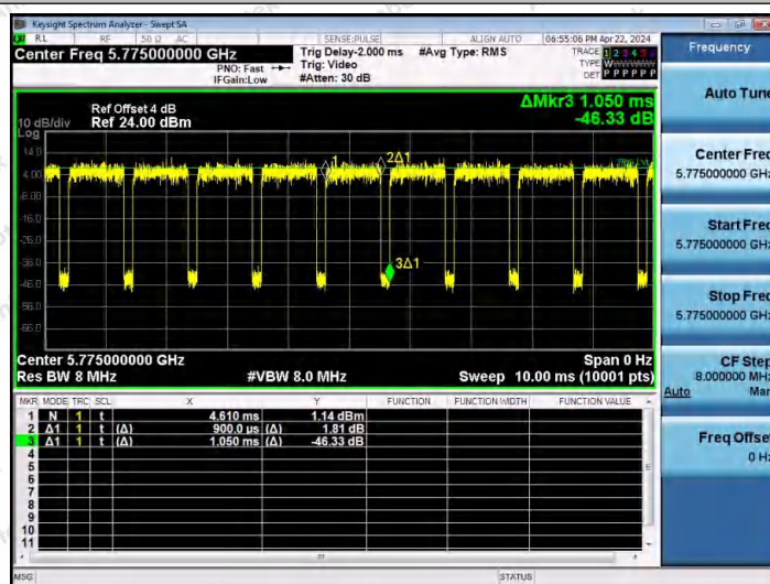
NTNV-11AC80MIMO-Ant2-5775
