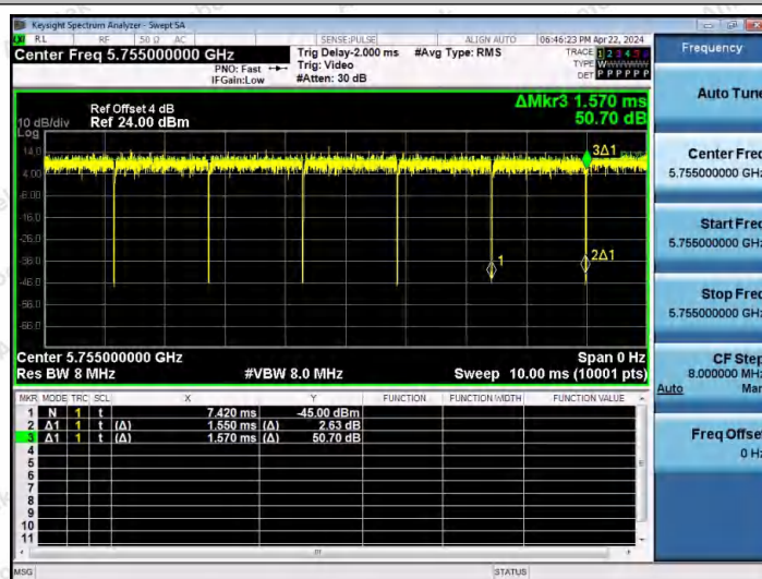
NTNV-11AC40MIMO-Ant1-5755
