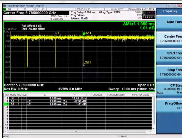
NTNV-11AC20MIMO-Ant1-5785
