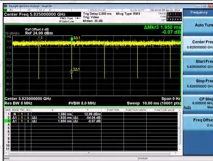
NTNV-11AC20MIMO-Ant2-5825
