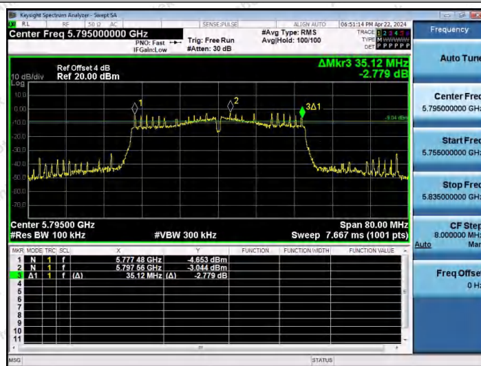
11AC40MIMO-Ant2-5795-PASS
