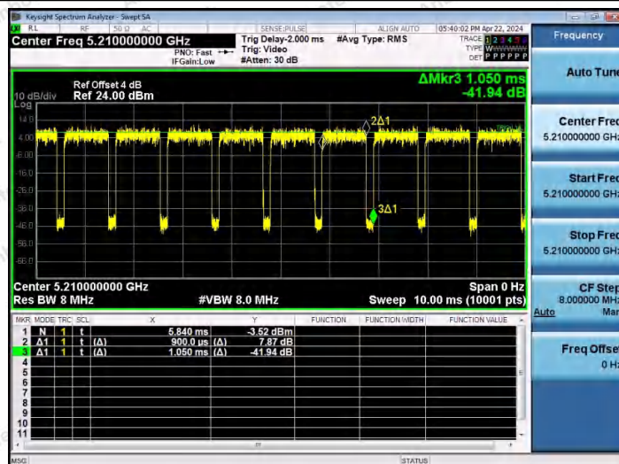
NTNV-11AC80MIMO-Ant2-5210
