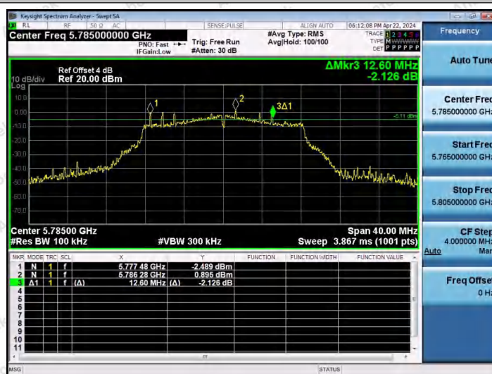
11A-Ant2-5785-PASS
