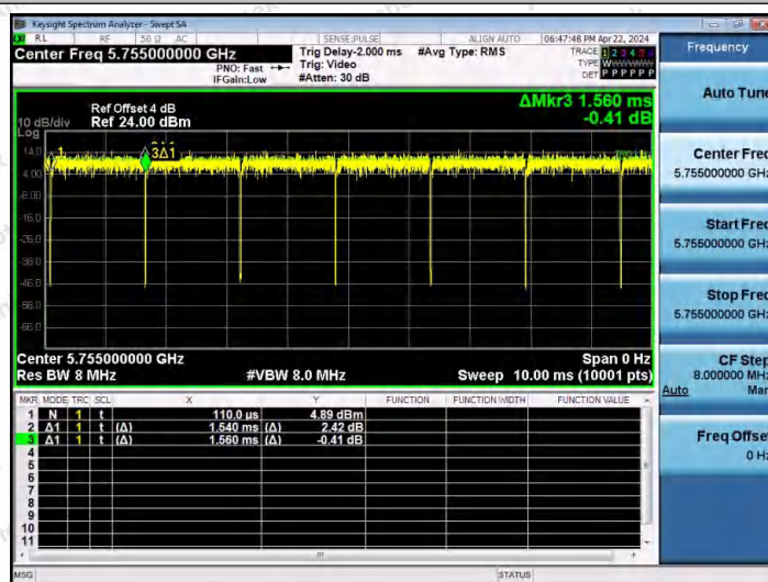
NTNV-11AC40MIMO-Ant2-5755
