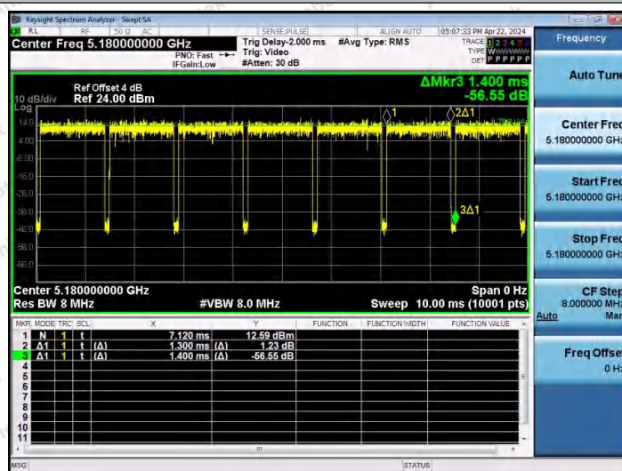
NTNV-11N20MIMO-Ant2-5180
