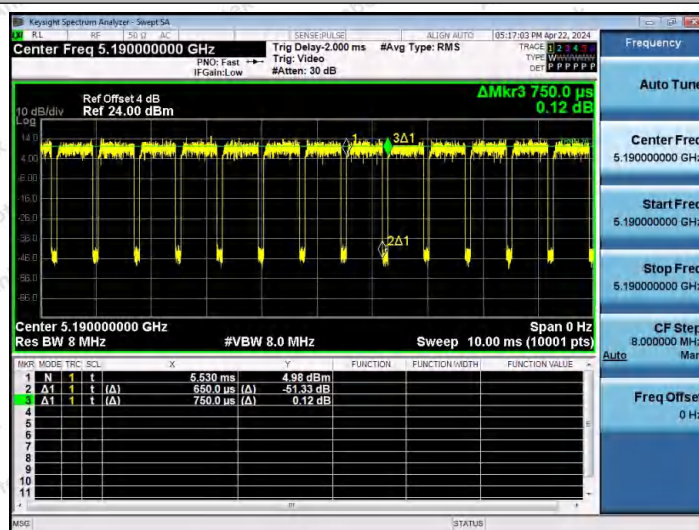
NTNV-11N40MIMO-Ant2-5190
