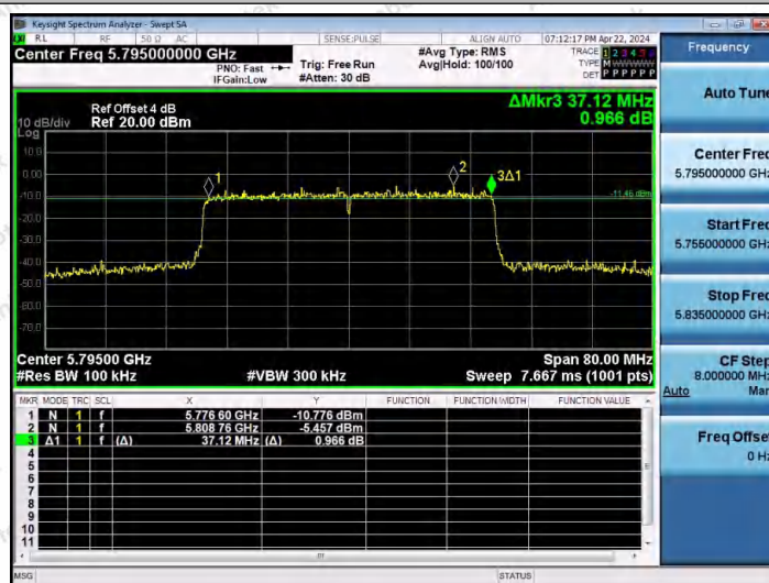
11AX40MIMO-Ant2-5795-PASS
