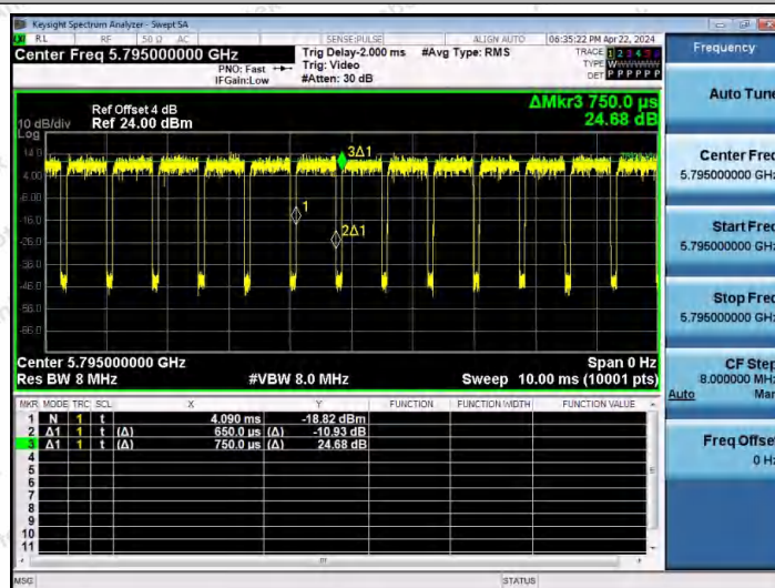
NTNV-11N40MIMO-Ant2-5795
