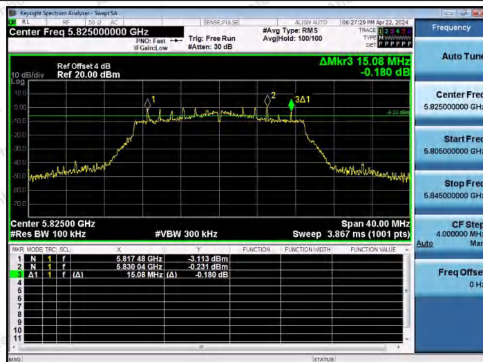
11N20MIMO-Ant2-5825-PASS
