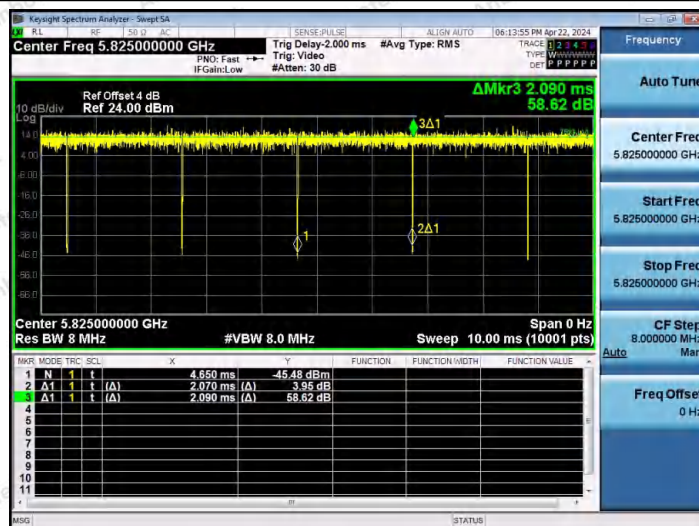
NTNV-11A-Ant2-5825
