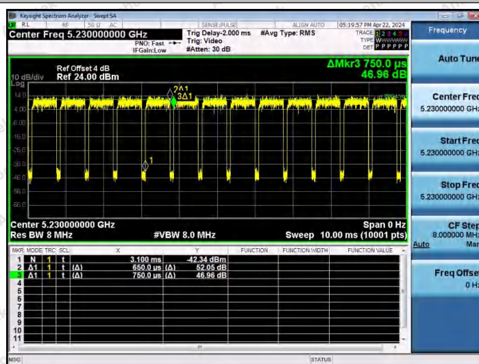
NTNV-11N40MIMO-Ant2-5230
