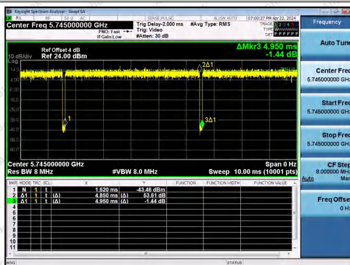
NTNV-11AX20MIMO-Ant2-5745
