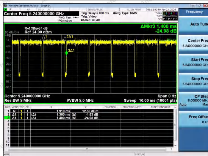
NTNV-11N20MIMO-Ant2-5240
