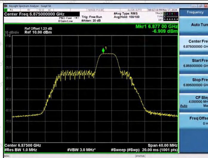
11AX20SISO-Ant1-6875-52Tone-RU39-PASS
