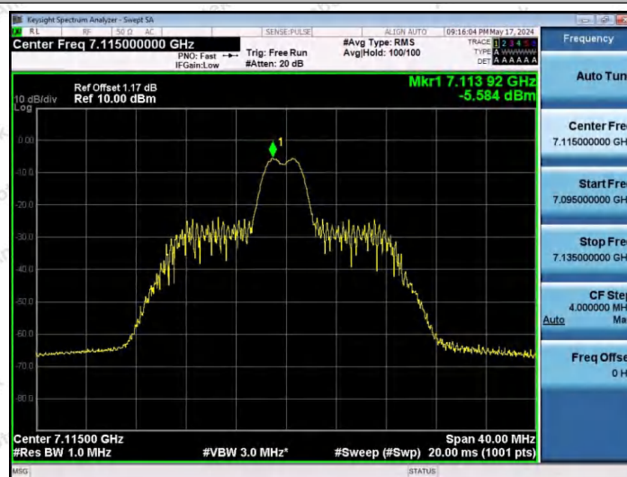
11AX20SISO-Ant1-7115-26Tone-RU4-PASS
