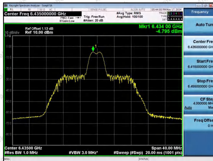
11AX20SISO-Ant1-6435-26Tone-RU4-PASS
