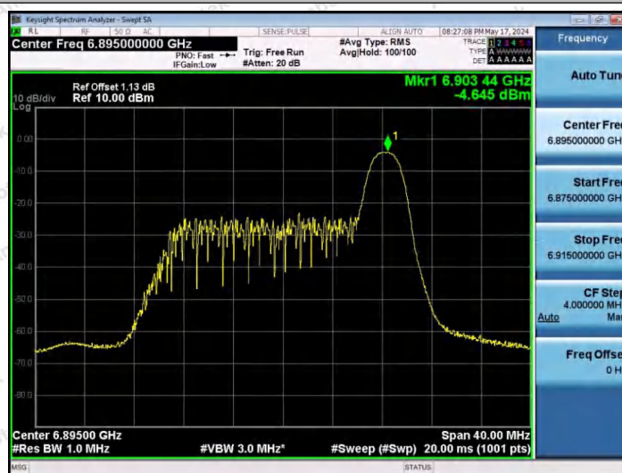
11AX20SISO-Ant1-6895-26Tone-RU8-PASS
