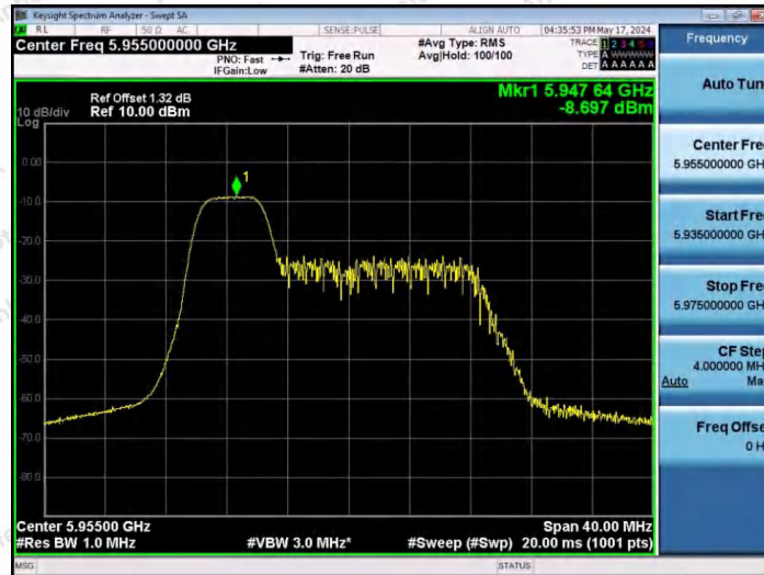
11AX20SISO-Ant1-5955-52Tone-RU37-PASS
