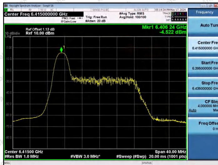
11AX20SISO-Ant1-6415-26Tone-RU0-PASS
