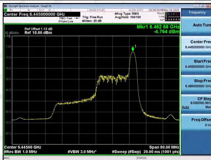
11AX40SISO-Ant1-6445-26Tone-RU17-PASS
