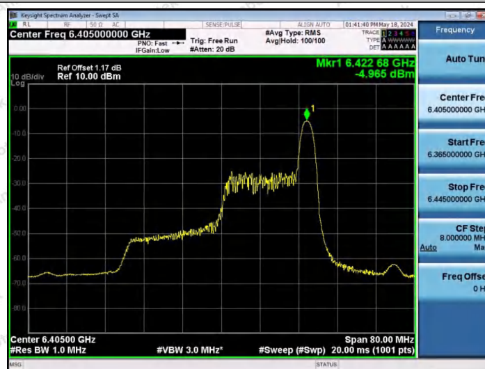
11AX40SISO-Ant1-6405-26Tone-RU17-PASS
