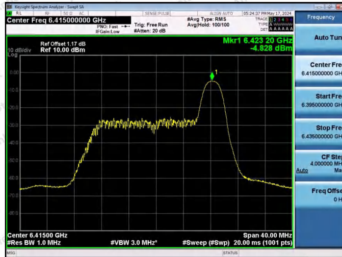
11AX20SISO-Ant1-6415-26Tone-RU8-PASS
