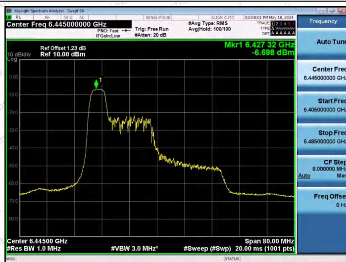
11AX40SISO-Ant1-6445-52Tone-RU37-PASS
