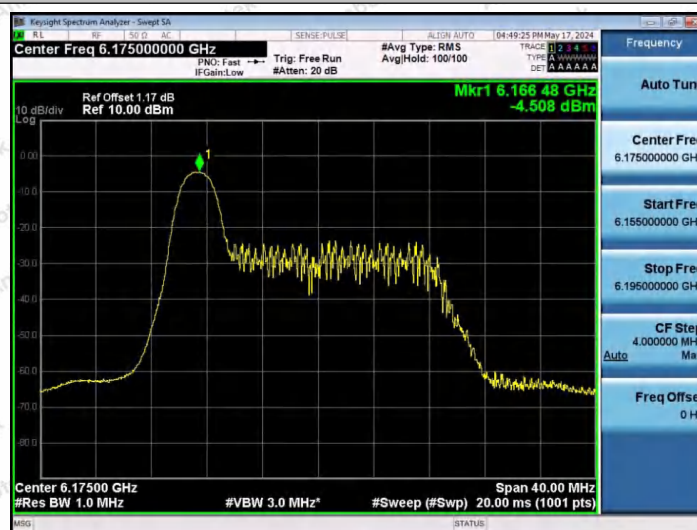
11AX20SISO-Ant1-6175-26Tone-RU0-PASS
