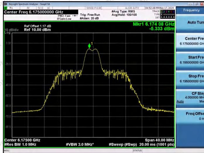
11AX20SISO-Ant1-6175-26Tone-RU4-PASS
