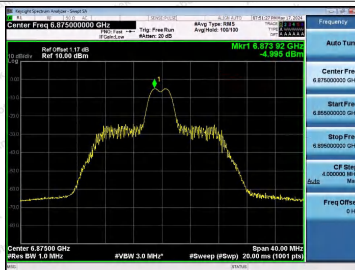
11AX20SISO-Ant1-6875-26Tone-RU4-PASS
