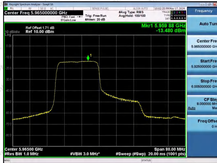
11AX40SISO-Ant1-5965-242Tone-RU61-PASS
