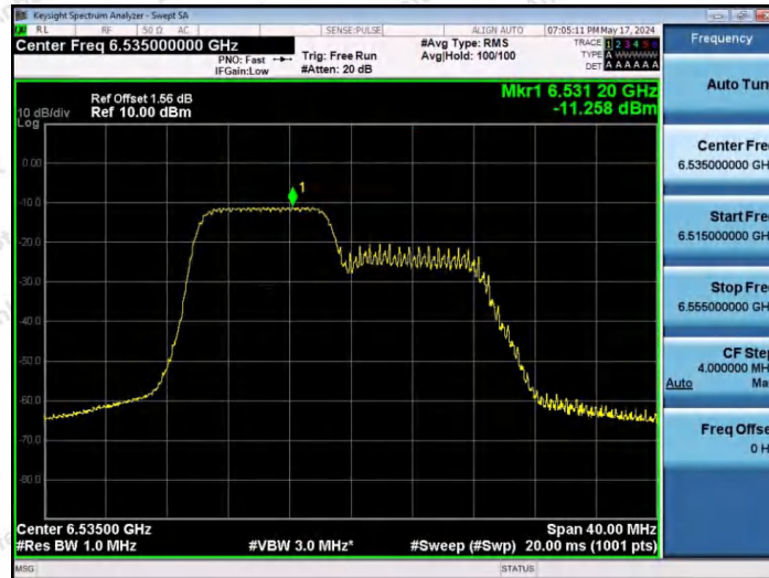
11AX20SISO-Ant1-6535-106Tone-RU53-PASS
