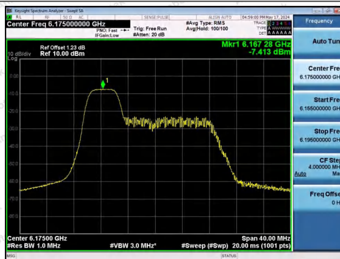
11AX20SISO-Ant1-6175-52Tone-RU37-PASS
