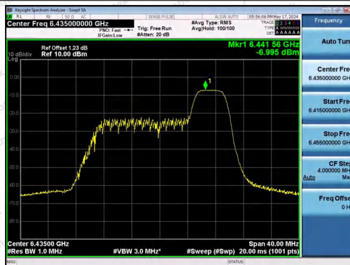
11AX20SISO-Ant1-6435-52Tone-RU40-PASS
