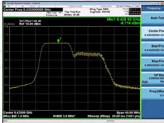
11AX20SISO-Ant1-6435-106Tone-RU53-PASS
