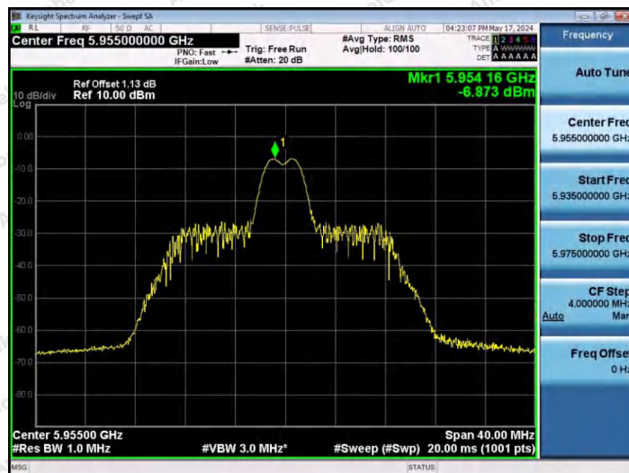
11AX20SISO-Ant1-5955-26Tone-RU4-PASS
