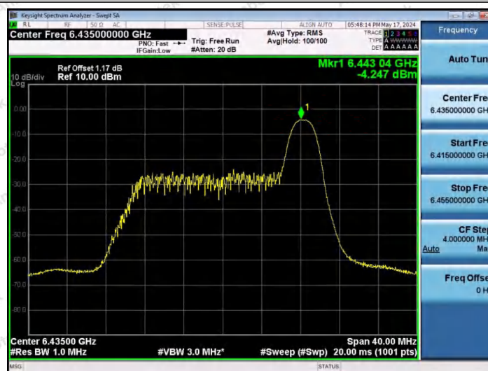
11AX20SISO-Ant1-6435-26Tone-RU8-PASS
