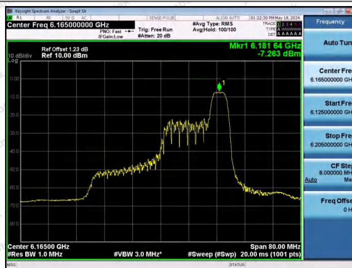
11AX40SISO-Ant1-6165-52Tone-RU44-PASS
