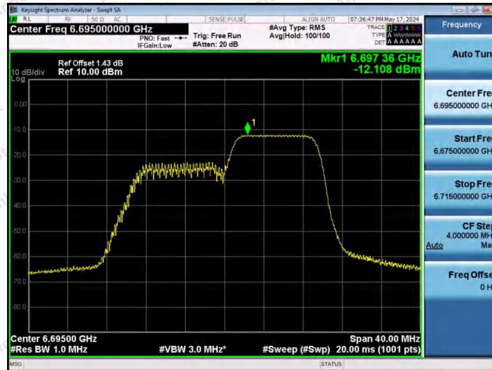
11AX20SISO-Ant1-6695-106Tone-RU54-PASS
