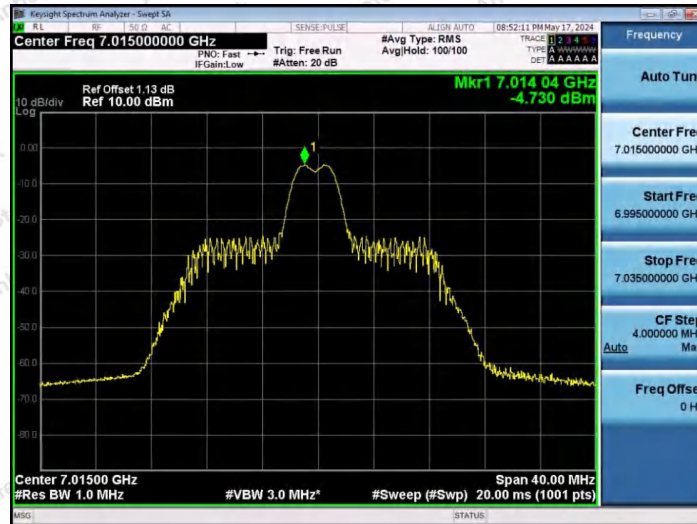
11AX20SISO-Ant1-7015-26Tone-RU4-PASS
