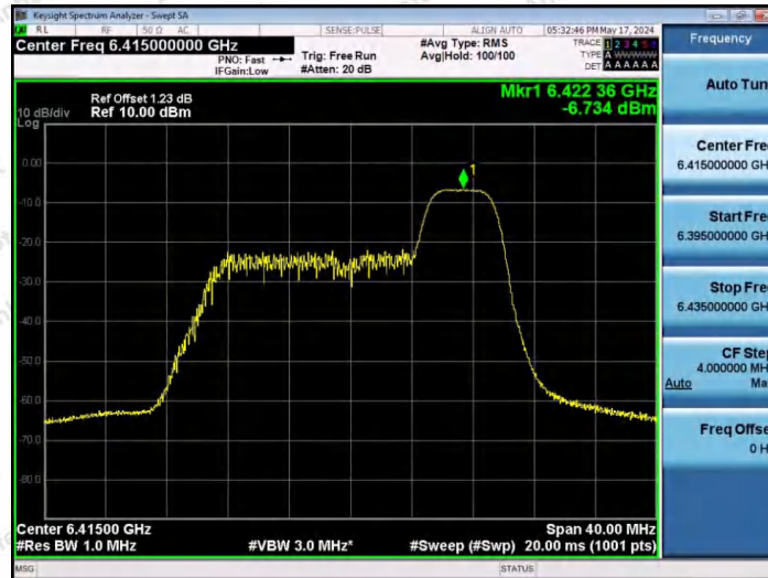
11AX20SISO-Ant1-6415-52Tone-RU40-PASS
