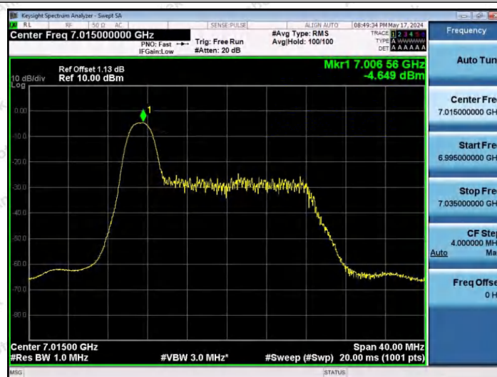
11AX20SISO-Ant1-7015-26Tone-RU0-PASS
