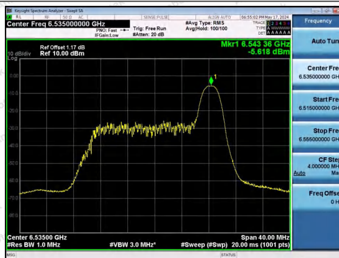
11AX20SISO-Ant1-6535-26Tone-RU8-PASS
