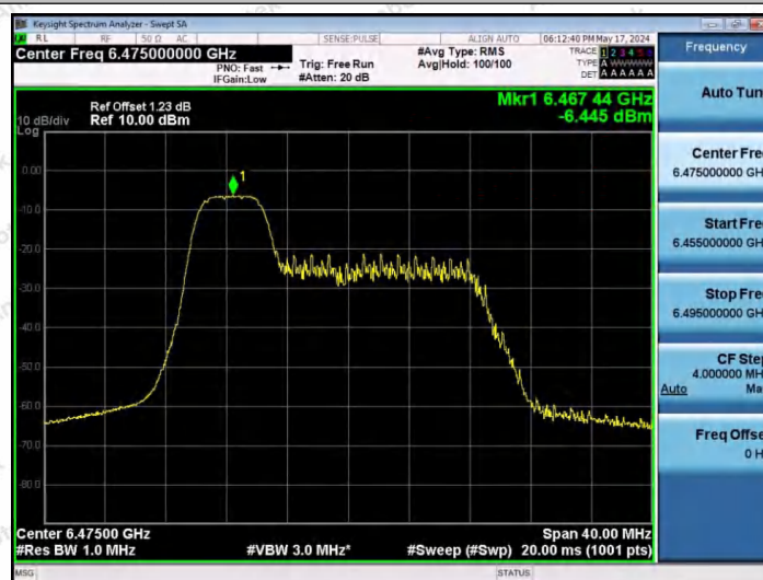
11AX20SISO-Ant1-6475-52Tone-RU37-PASS
