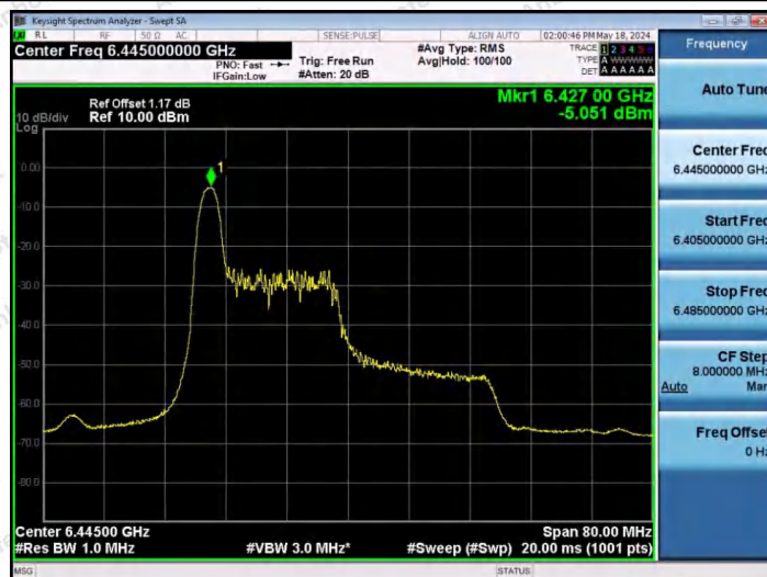
11AX40SISO-Ant1-6445-26Tone-RU0-PASS
