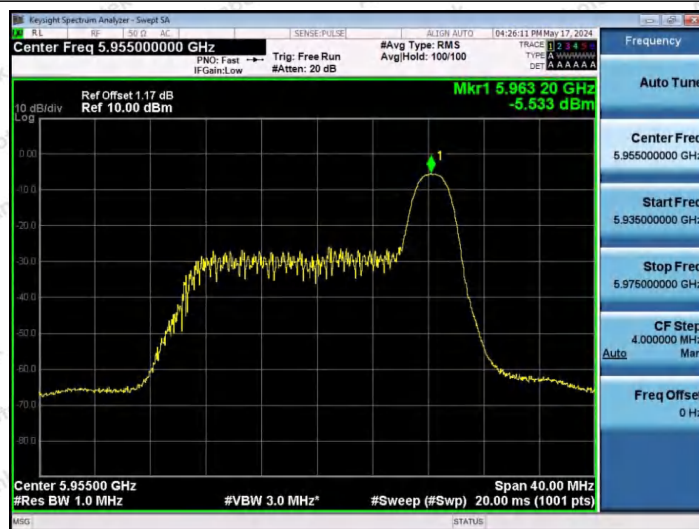
11AX20SISO-Ant1-5955-26Tone-RU8-PASS
