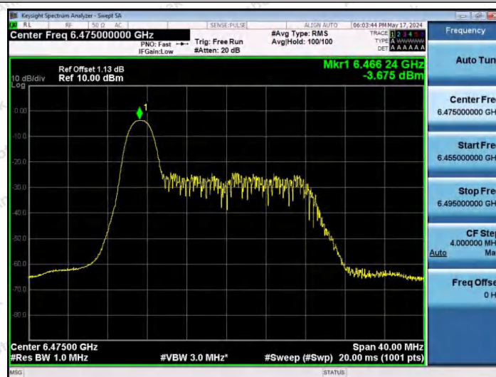
11AX20SISO-Ant1-6475-26Tone-RU0-PASS
