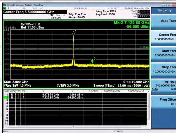
11AX40SISO-Ant1-6165-106Tone-RU56-3000~10000-PASS
