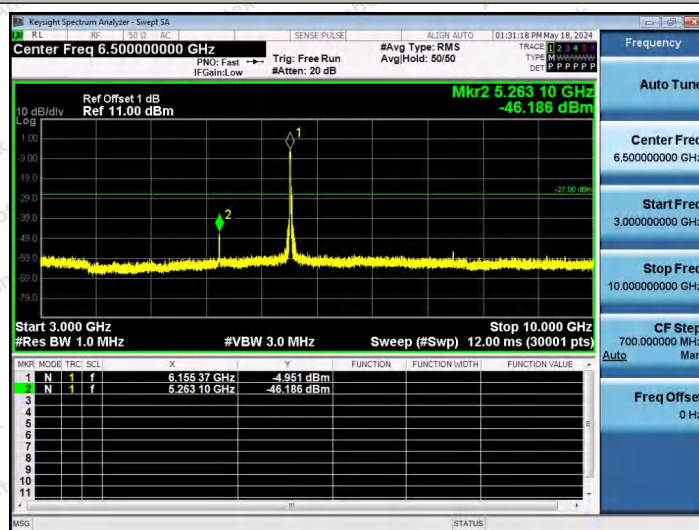
11AX40SISO-Ant1-6165-242Tone-RU61-3000~10000-PASS
