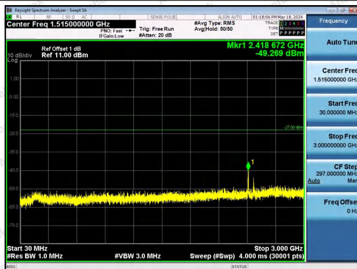
11AX40SISO-Ant1-6165-26Tone-RU17-30~3000-PASS
