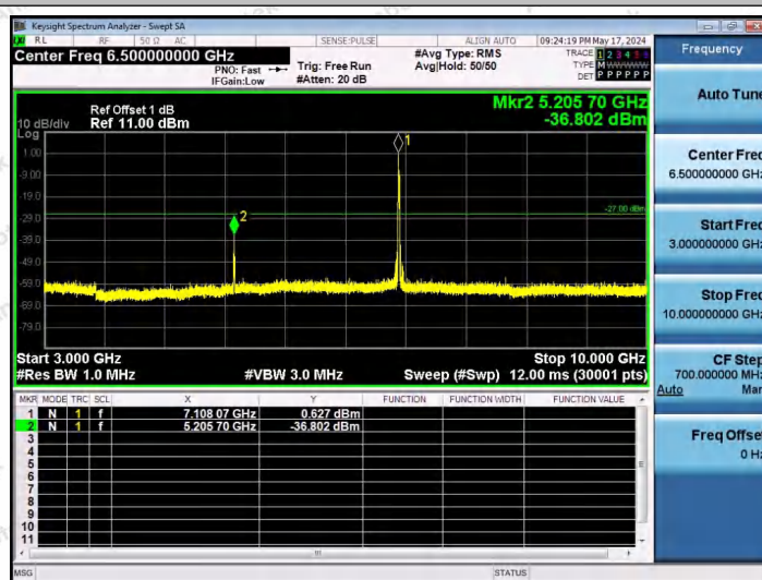
11AX20SISO-Ant1-7115-52Tone-RU37-3000~10000-PASS
