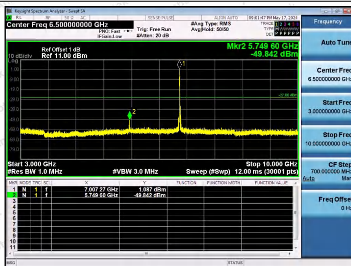
11AX20SISO-Ant1-7015-52Tone-RU37-3000~10000-PASS
