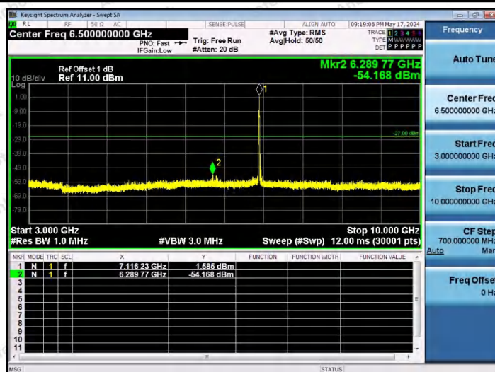
11AX20SISO-Ant1-7115-26Tone-RU4-3000~10000-PASS
