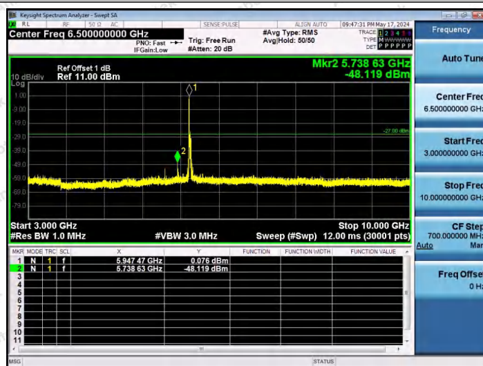
11AX40SISO-Ant1-5965-26Tone-RU0-3000~10000-PASS
