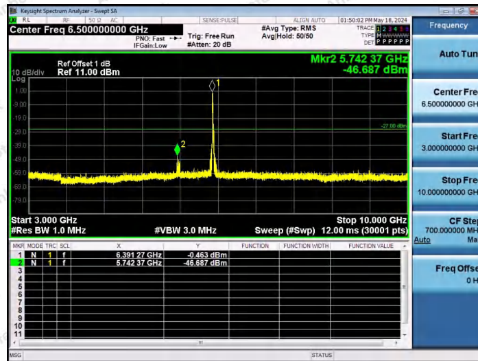
11AX40SISO-Ant1-6405-106Tone-RU53-3000~10000-PASS
