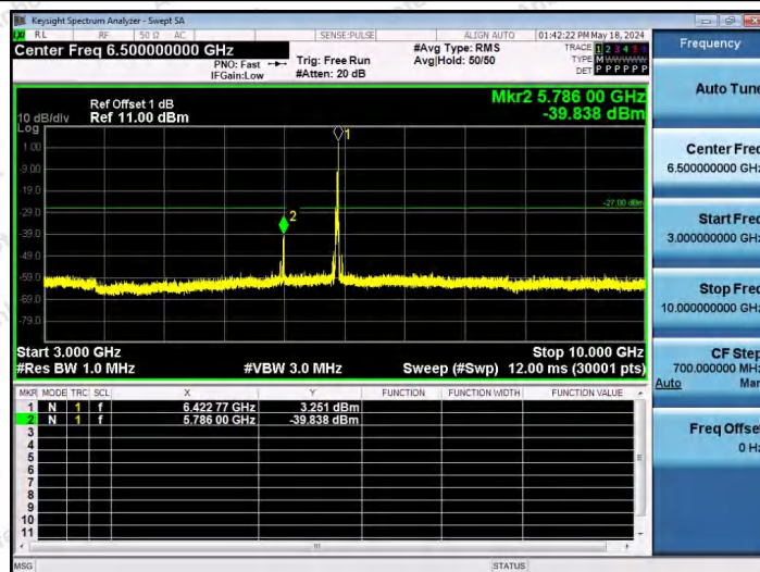
11AX40SISO-Ant1-6405-26Tone-RU17-3000~10000-PASS
