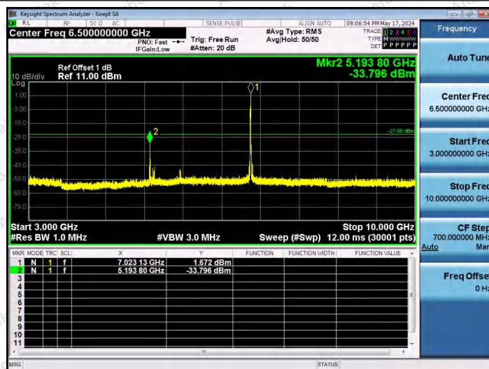
11AX20SISO-Ant1-7015-52Tone-RU40-3000~10000-PASS
