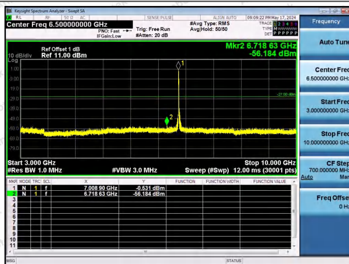
11AX20SISO-Ant1-7015-106Tone-RU53-3000~10000-PASS
