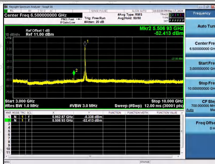
11AX40SISO-Ant1-5965-242Tone-RU61-3000~10000-PASS
