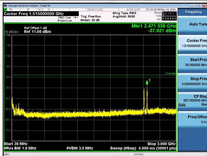
11AX40SISO-Ant1-6405-242Tone-RU61-30~3000-PASS
