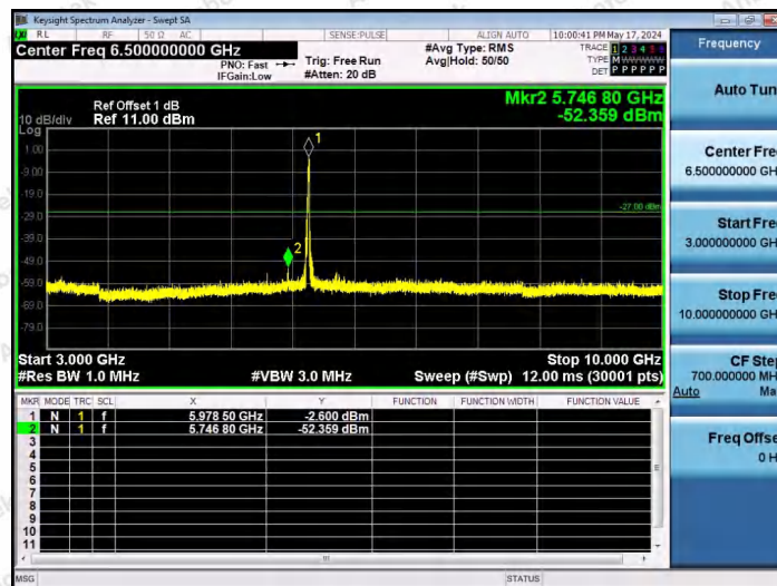
11AX40SISO-Ant1-5965-106Tone-RU56-3000~10000-PASS
