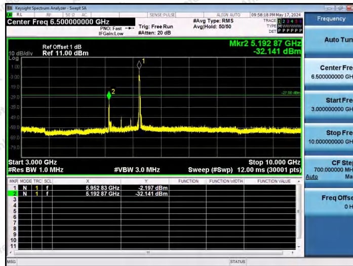
11AX40SISO-Ant1-5965-106Tone-RU53-3000~10000-PASS
