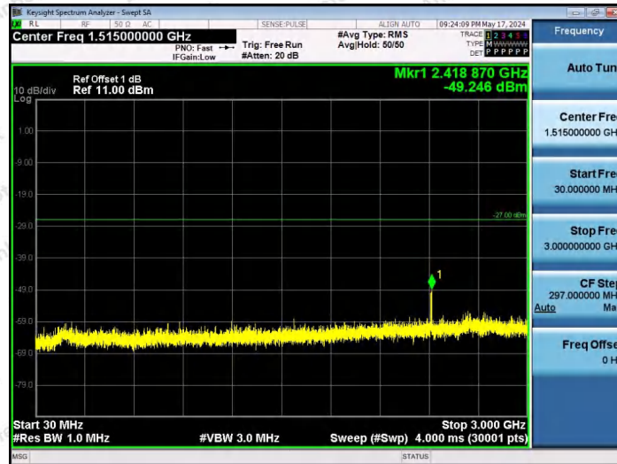
11AX20SISO-Ant1-7115-52Tone-RU37-30~3000-PASS
