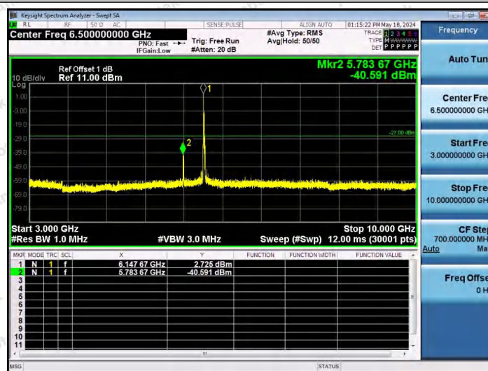
11AX40SISO-Ant1-6165-26Tone-RU0-3000~10000-PASS
