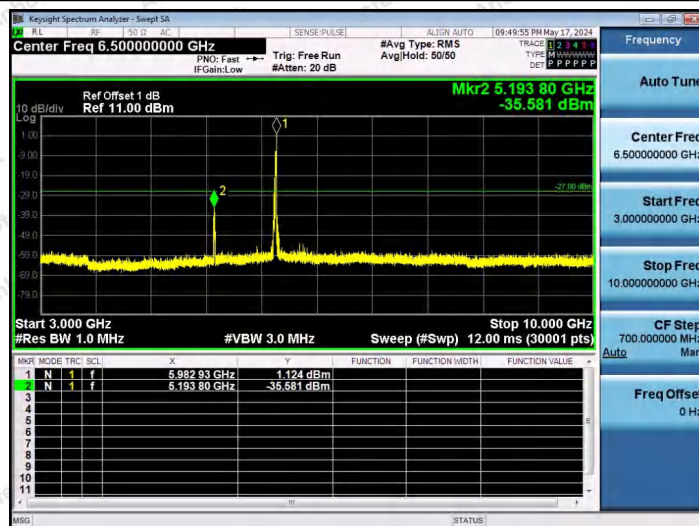
11AX40SISO-Ant1-5965-26Tone-RU17-3000~10000-PASS
