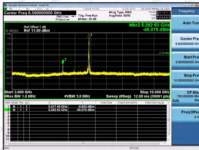
11AX40SISO-Ant1-6405-106Tone-RU56-3000~10000-PASS
