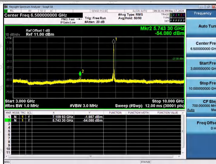
11AX20SISO-Ant1-7115-106Tone-RU53-3000~10000-PASS
