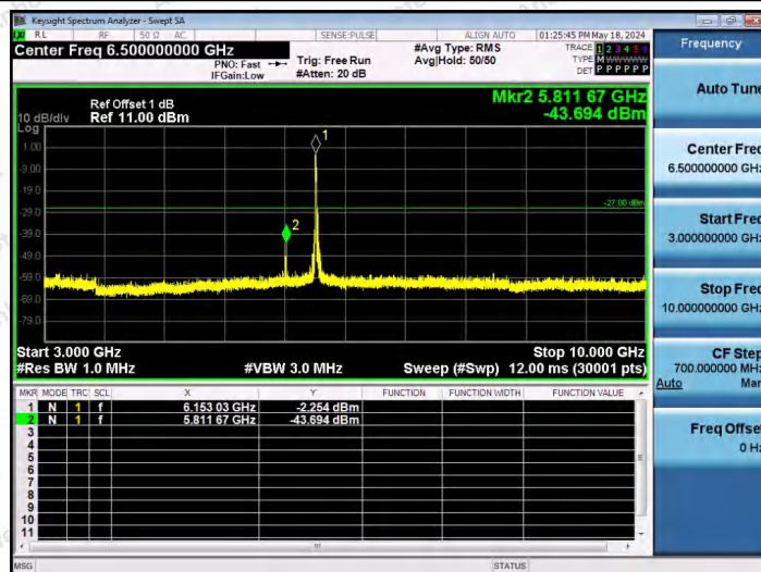
11AX40SISO-Ant1-6165-106Tone-RU53-3000~10000-PASS
