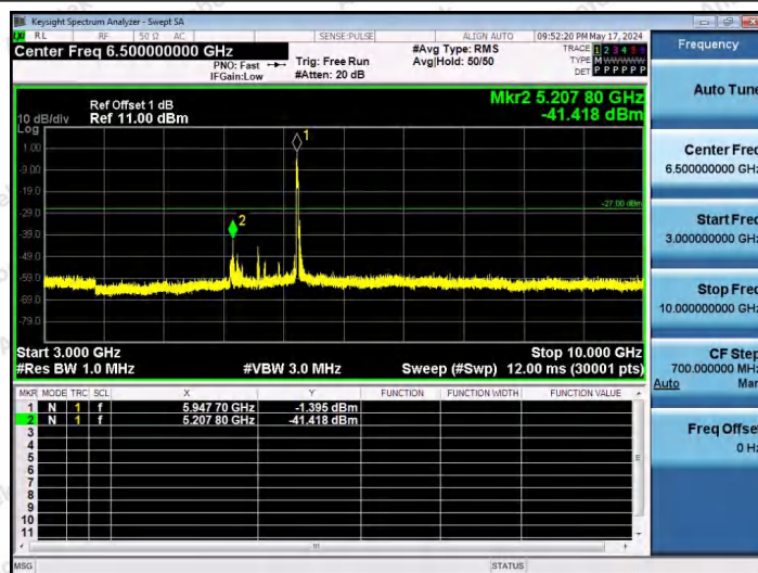
11AX40SISO-Ant1-5965-52Tone-RU37-3000~10000-PASS
