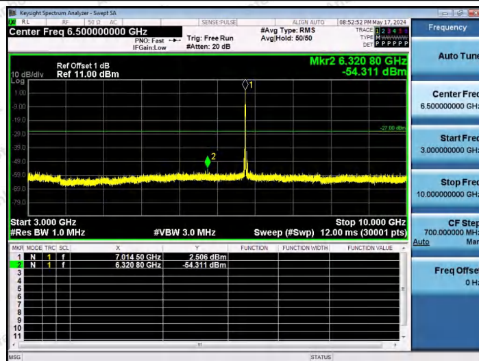
11AX20SISO-Ant1-7015-26Tone-RU4-3000~10000-PASS
