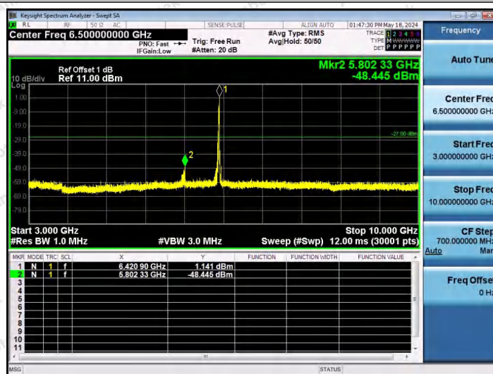
11AX40SISO-Ant1-6405-52Tone-RU44-3000~10000-PASS
