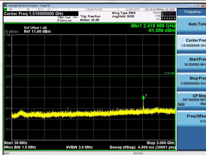
11AX40SISO-Ant1-6165-26Tone-RU0-30~3000-PASS
