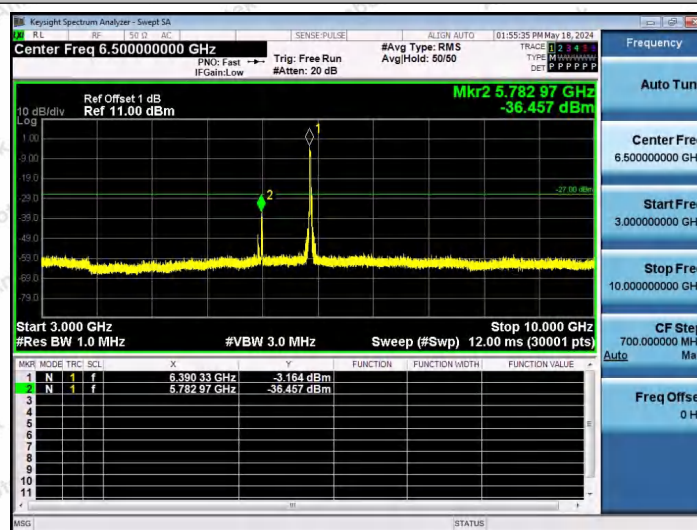
11AX40SISO-Ant1-6405-242Tone-RU61-3000~10000-PASS
