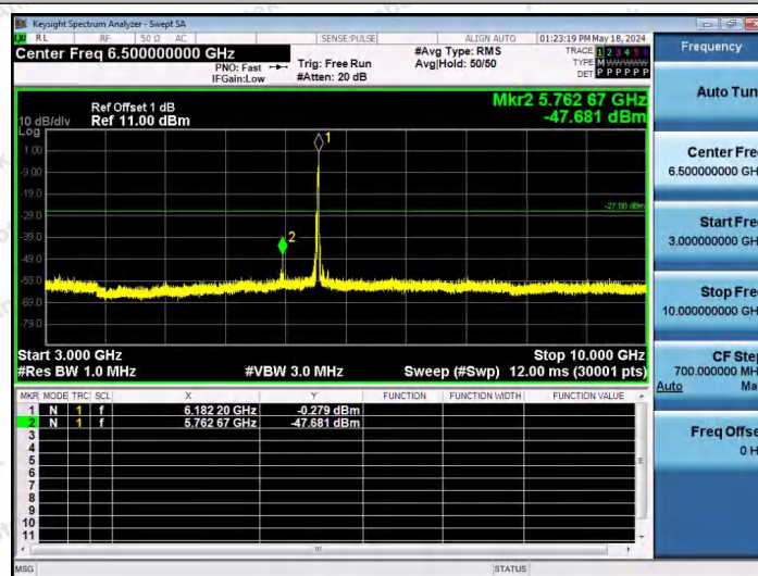
11AX40SISO-Ant1-6165-52Tone-RU44-3000~10000-PASS
