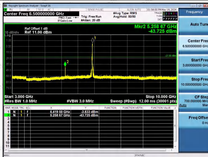
11AX40SISO-Ant1-6405-242Tone-RU62-3000~10000-PASS
