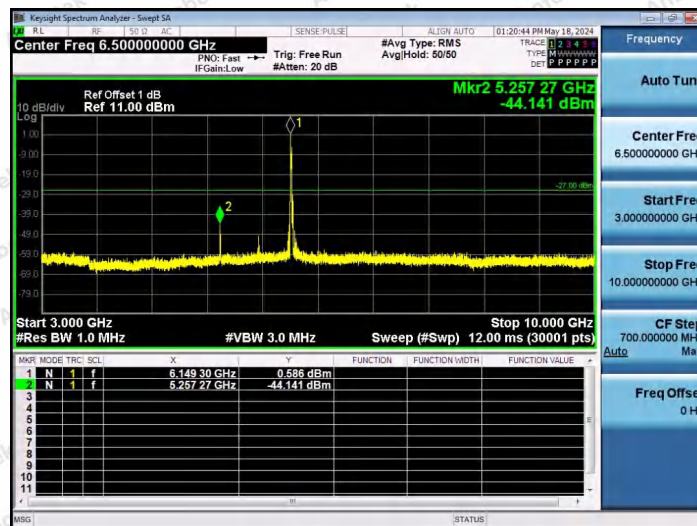
11AX40SISO-Ant1-6165-52Tone-RU37-3000~10000-PASS
