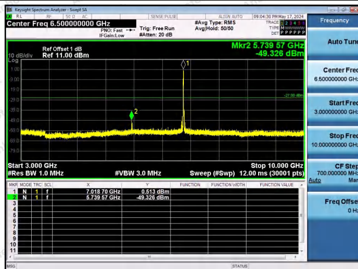
11AX20SISO-Ant1-7015-52Tone-RU39-3000~10000-PASS
