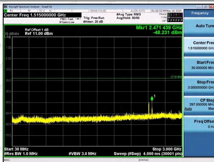
11AX40SISO-Ant1-6165-52Tone-RU37-30~3000-PASS
