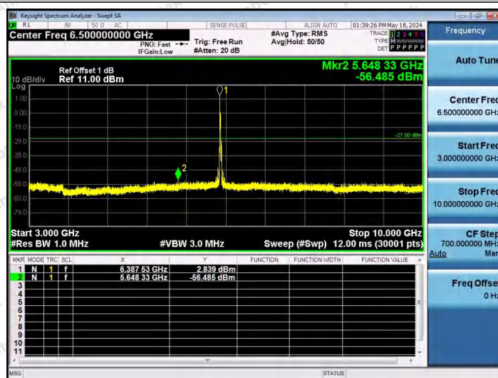
11AX40SISO-Ant1-6405-26Tone-RU0-3000~10000-PASS
