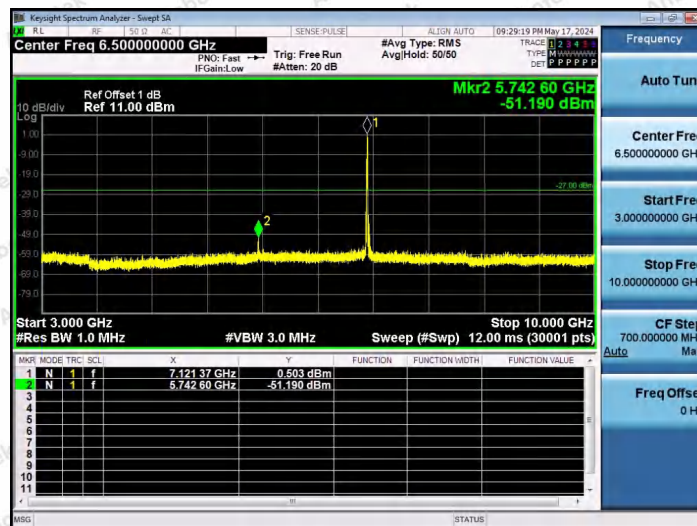
11AX20SISO-Ant1-7115-52Tone-RU40-3000~10000-PASS
