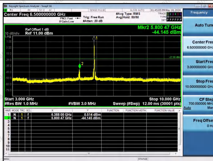
11AX40SISO-Ant1-6405-52Tone-RU37-3000~10000-PASS
