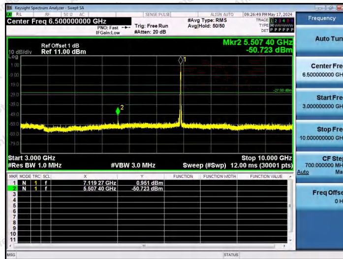
11AX20SISO-Ant1-7115-52Tone-RU39-3000~10000-PASS
