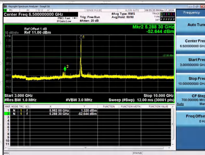
11AX40SISO-Ant1-5965-52Tone-RU44-3000~10000-PASS
