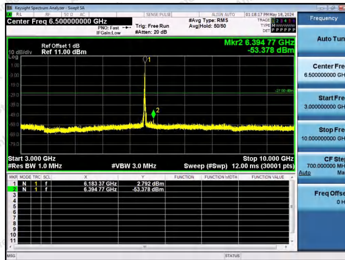
11AX40SISO-Ant1-6165-26Tone-RU17-3000~10000-PASS
