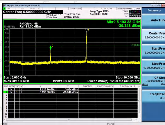
11AX20SISO-Ant1-7115-26Tone-RU8-3000~10000-PASS
