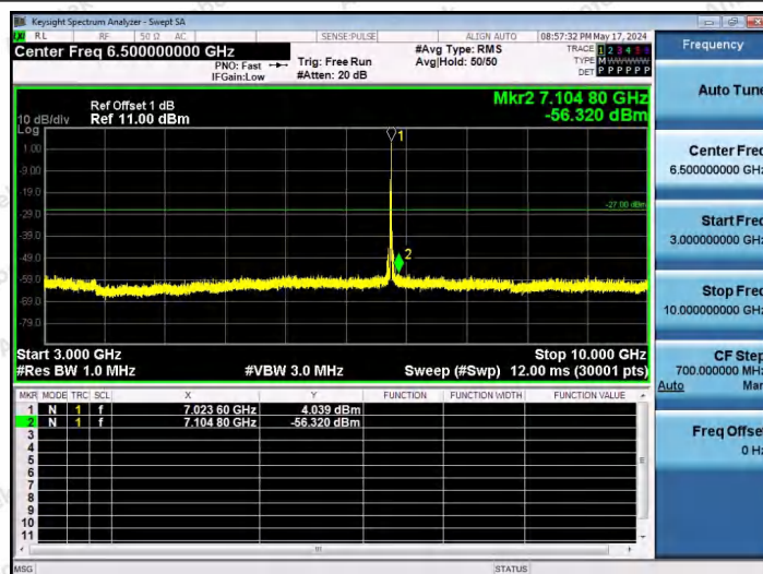
11AX20SISO-Ant1-7015-26Tone-RU8-3000~10000-PASS
