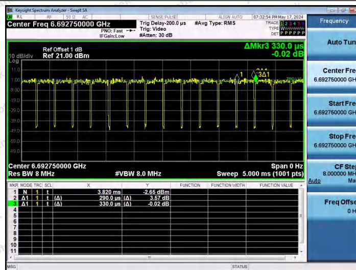
NTNV-11AX20SISO-Ant1-6695-106Tone-RU53
