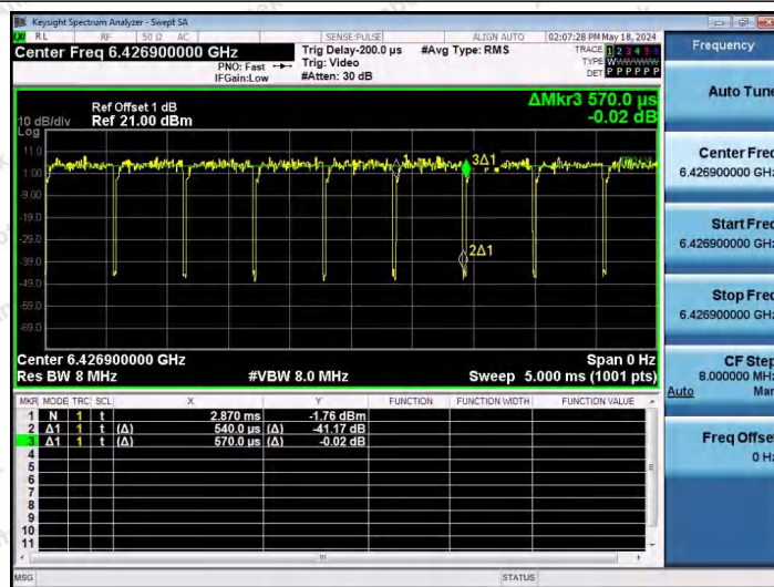
NTNV-11AX40SISO-Ant1-6445-52Tone-RU37
