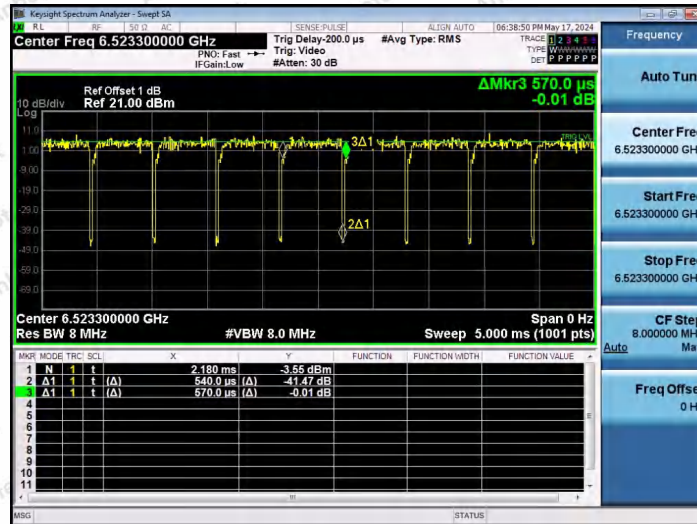
NTNV-11AX20SISO-Ant1-6515-52Tone-RU40
