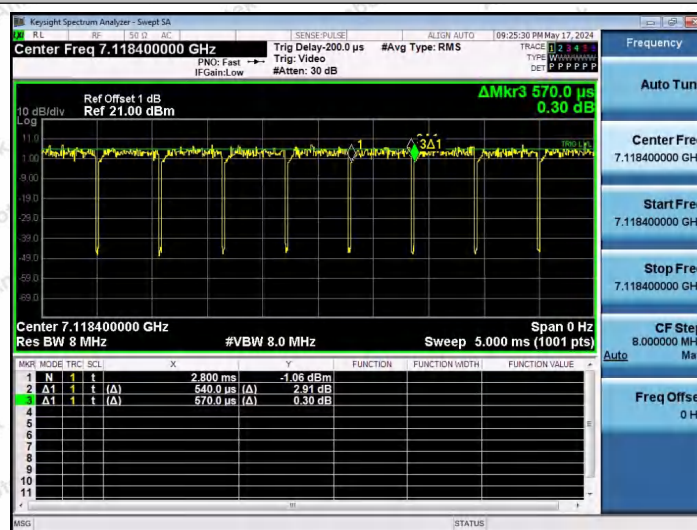
NTNV-11AX20SISO-Ant1-7115-52Tone-RU39
