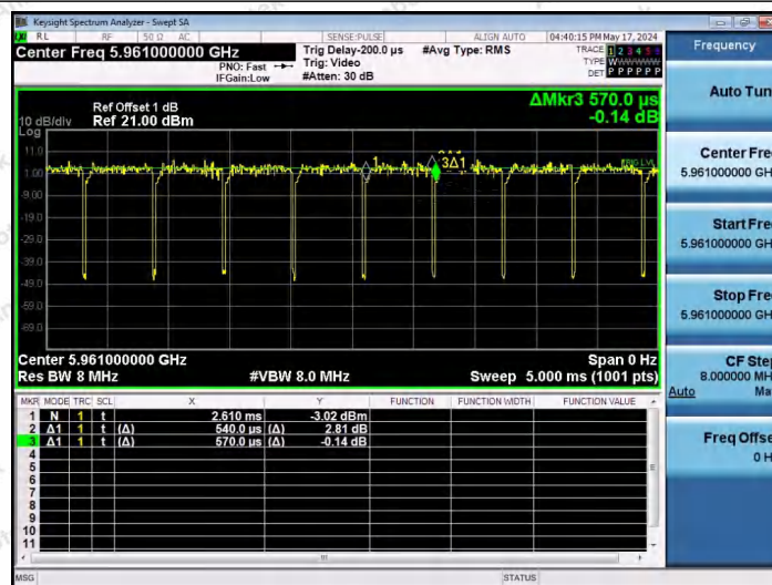
NTNV-11AX20SISO-Ant1-5955-52Tone-RU40
