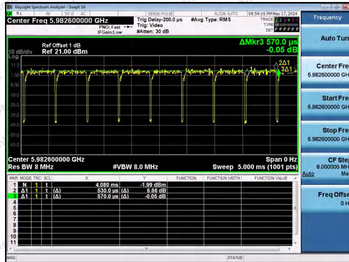
NTNV-11AX40SISO-Ant1-5965-52Tone-RU44
