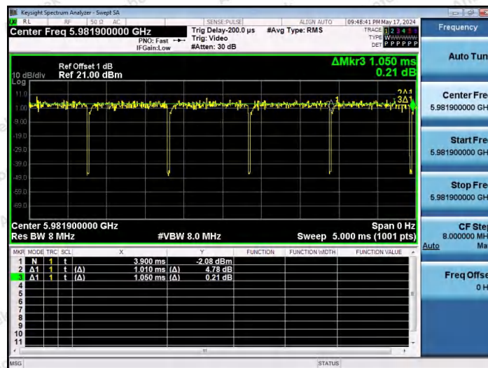
NTNV-11AX40SISO-Ant1-5965-26Tone-RU17
