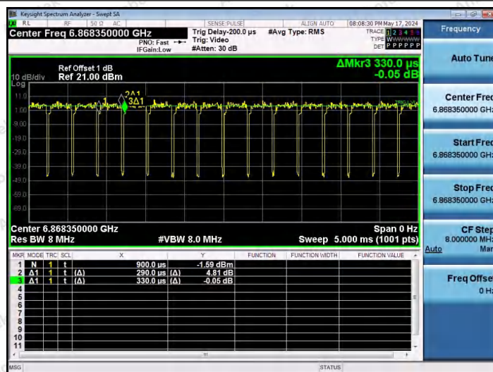
NTNV-11AX20SISO-Ant1-6875-106Tone-RU53
