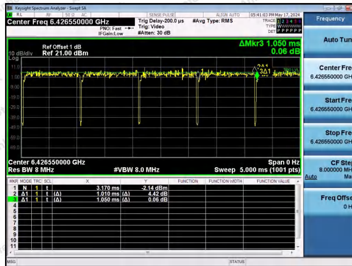
NTNV-11AX20SISO-Ant1-6435-26Tone-RU0
