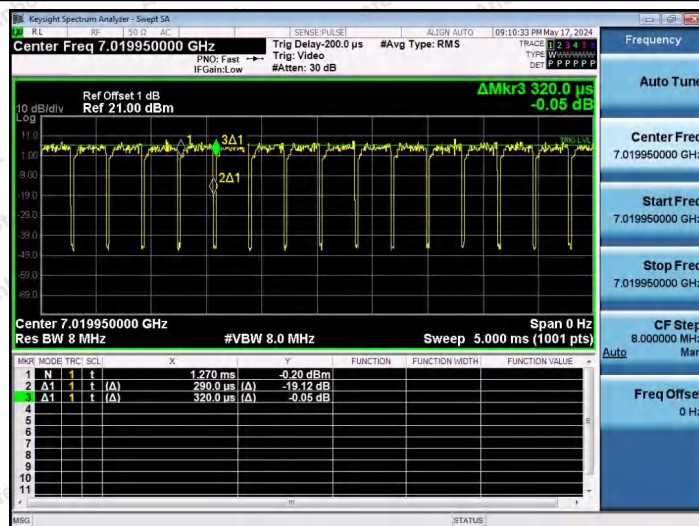
NTNV-11AX20SISO-Ant1-7015-106Tone-RU54
