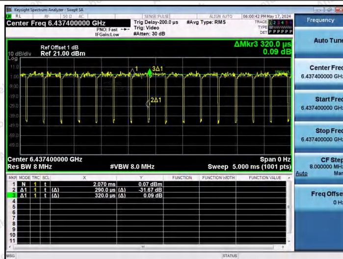
NTNV-11AX20SISO-Ant1-6435-106Tone-RU54
