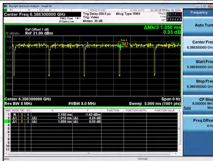
NTNV-11AX40SISO-Ant1-6405-26Tone-RU0
