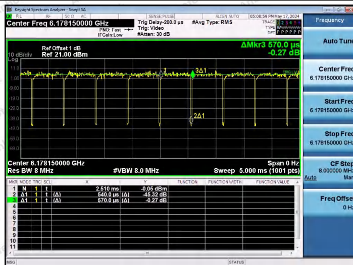
NTNV-11AX20SISO-Ant1-6175-52Tone-RU39
