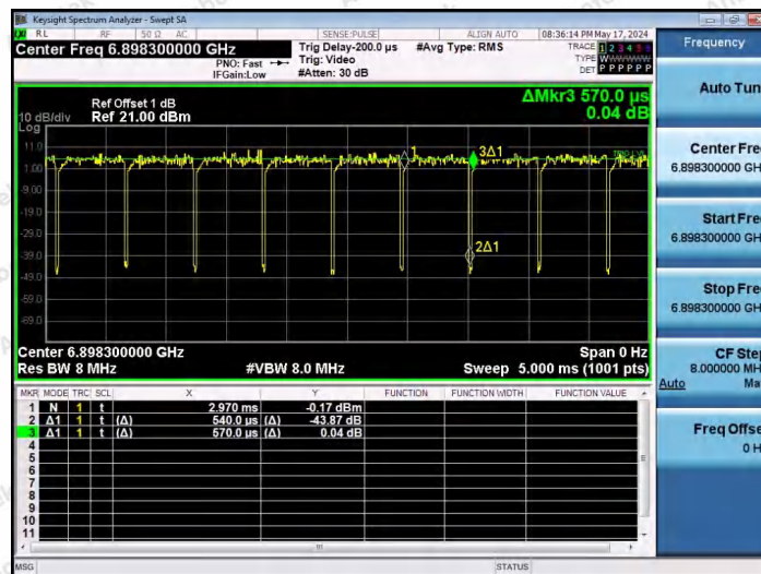
NTNV-11AX20SISO-Ant1-6895-52Tone-RU39
