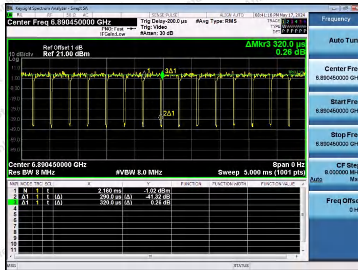
NTNV-11AX20SISO-Ant1-6895-106Tone-RU53
