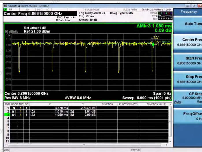
NTNV-11AX20SISO-Ant1-6875-26Tone-RU0
