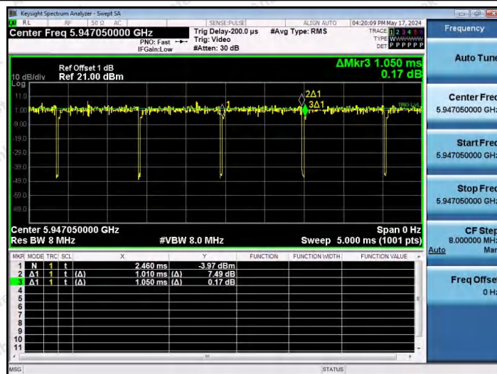
NTNV-11AX20SISO-Ant1-5955-26Tone-RU0
