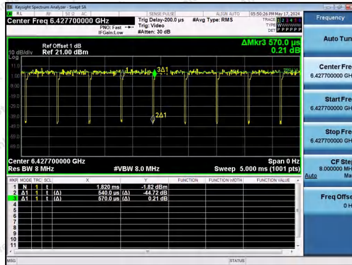
NTNV-11AX20SISO-Ant1-6435-52Tone-RU37
