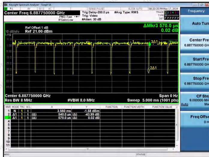
NTNV-11AX20SISO-Ant1-6895-52Tone-RU37
