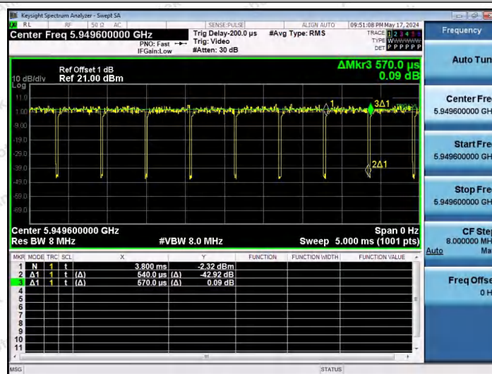
NTNV-11AX40SISO-Ant1-5965-52Tone-RU37
