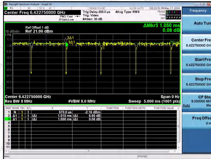
NTNV-11AX20SISO-Ant1-6415-26Tone-RU8
