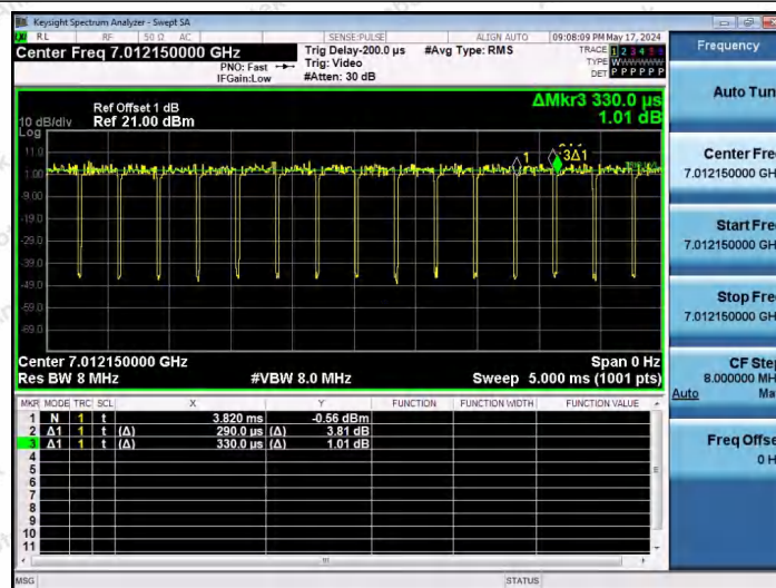
NTNV-11AX20SISO-Ant1-7015-106Tone-RU53
