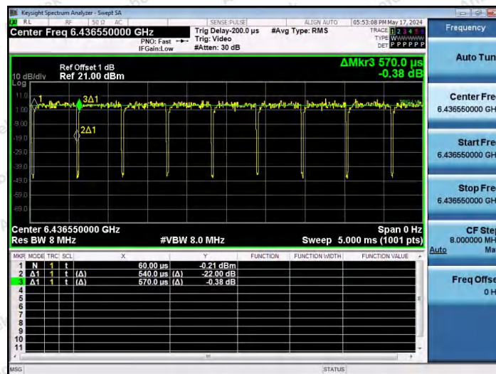
NTNV-11AX20SISO-Ant1-6435-52Tone-RU39
