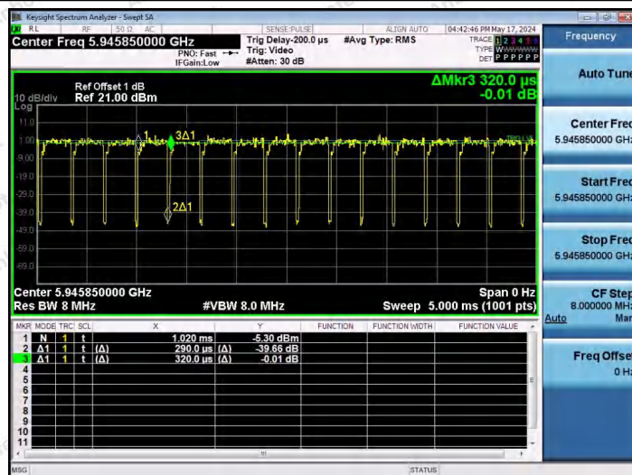
NTNV-11AX20SISO-Ant1-5955-106Tone-RU53
