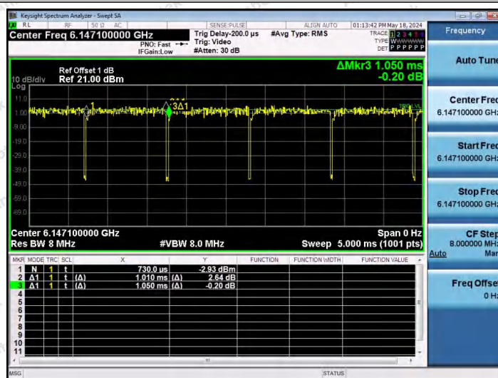
NTNV-11AX40SISO-Ant1-6165-26Tone-RU0
