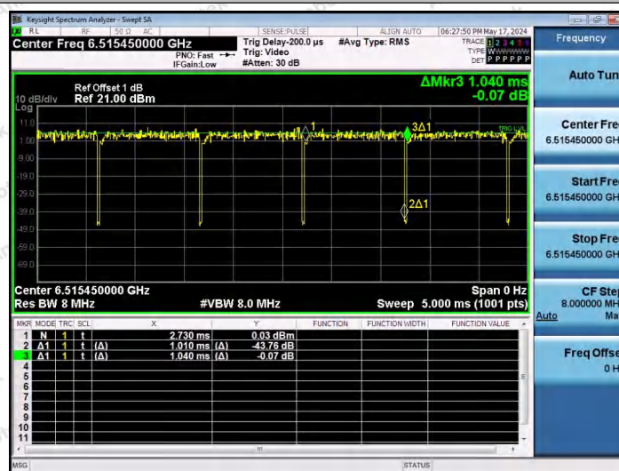
NTNV-11AX20SISO-Ant1-6515-26Tone-RU4
