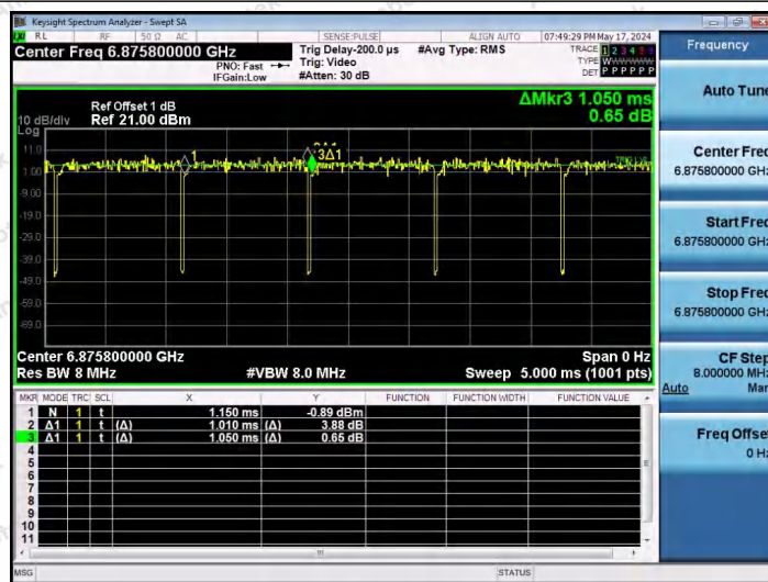
NTNV-11AX20SISO-Ant1-6875-26Tone-RU4
