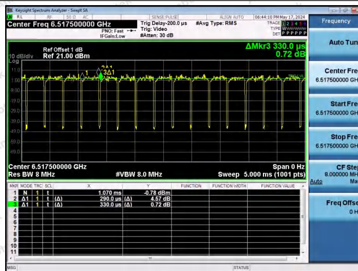
NTNV-11AX20SISO-Ant1-6515-106Tone-RU54
