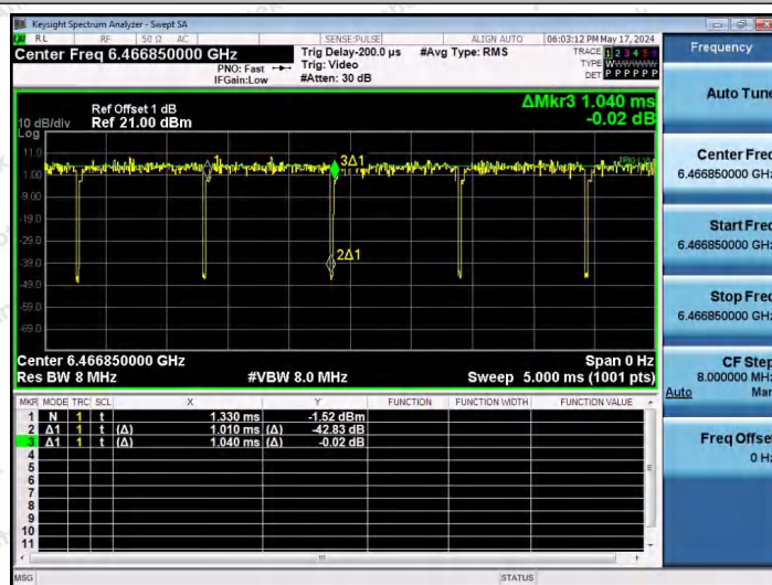
NTNV-11AX20SISO-Ant1-6475-26Tone-RU0
