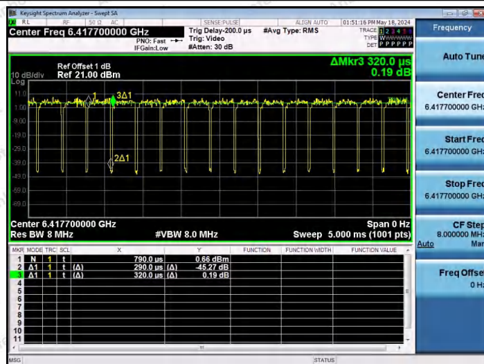
NTNV-11AX40SISO-Ant1-6405-106Tone-RU56
