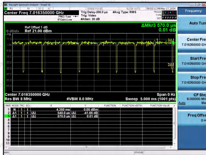
NTNV-11AX20SISO-Ant1-7015-52Tone-RU39
