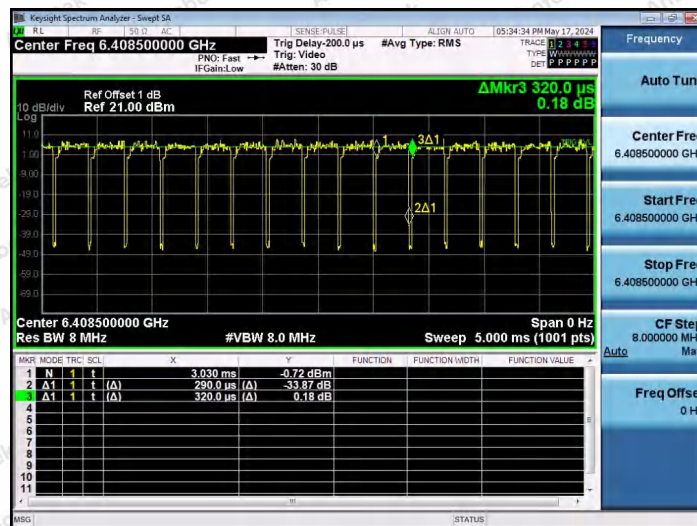
NTNV-11AX20SISO-Ant1-6415-106Tone-RU53
