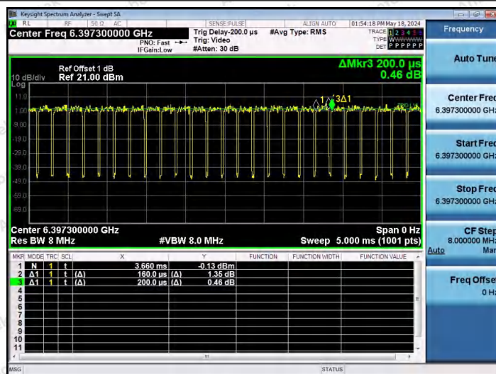
NTNV-11AX40SISO-Ant1-6405-242Tone-RU61
