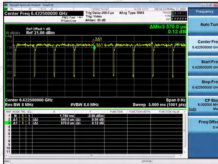
NTNV-11AX20SISO-Ant1-6415-52Tone-RU40
