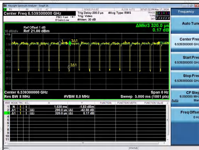
NTNV-11AX20SISO-Ant1-6535-106Tone-RU54
