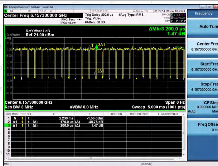
NTNV-11AX40SISO-Ant1-6165-242Tone-RU61
