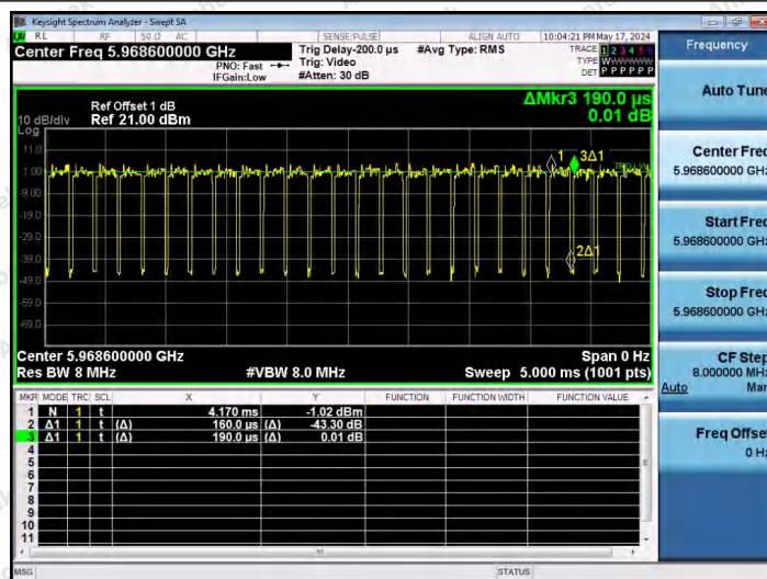
NTNV-11AX40SISO-Ant1-5965-242Tone-RU62
