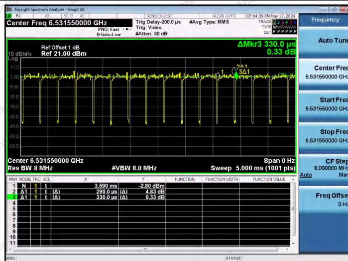
NTNV-11AX20SISO-Ant1-6535-106Tone-RU53
