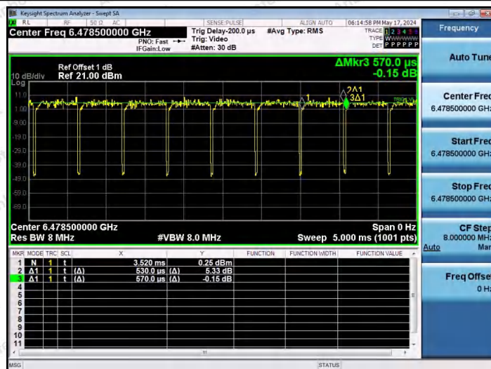
NTNV-11AX20SISO-Ant1-6475-52Tone-RU39
