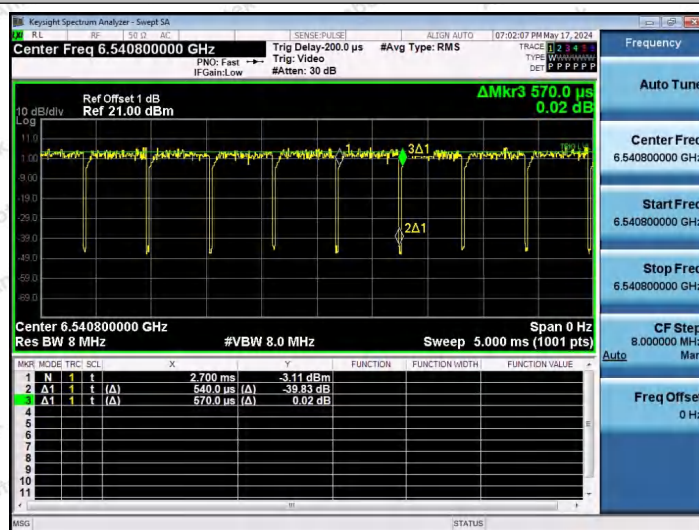
NTNV-11AX20SISO-Ant1-6535-52Tone-RU40
