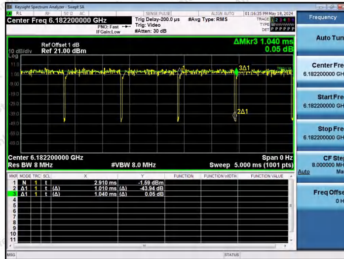
NTNV-11AX40SISO-Ant1-6165-26Tone-RU17
