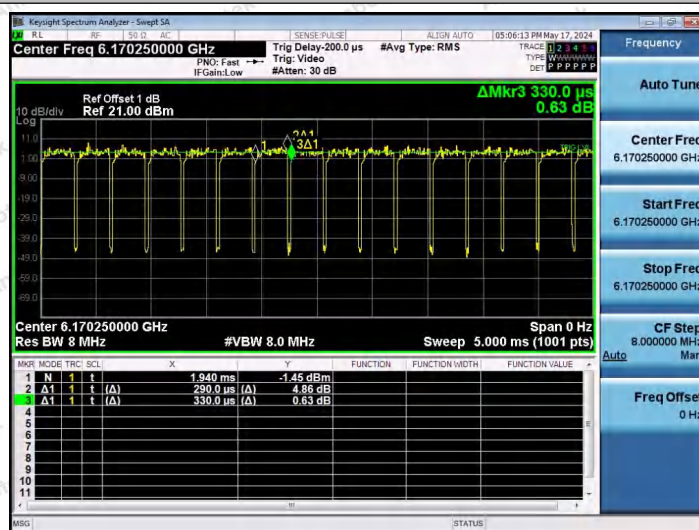
NTNV-11AX20SISO-Ant1-6175-106Tone-RU53
