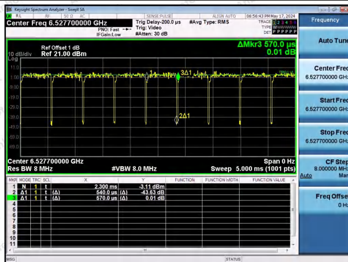
NTNV-11AX20SISO-Ant1-6535-52Tone-RU37
