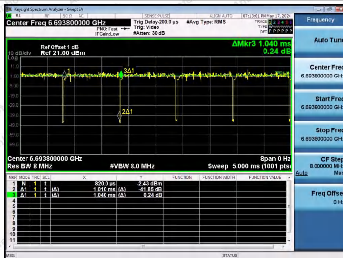
NTNV-11AX20SISO-Ant1-6695-26Tone-RU4
