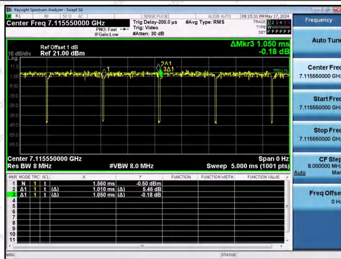
NTNV-11AX20SISO-Ant1-7115-26Tone-RU4
