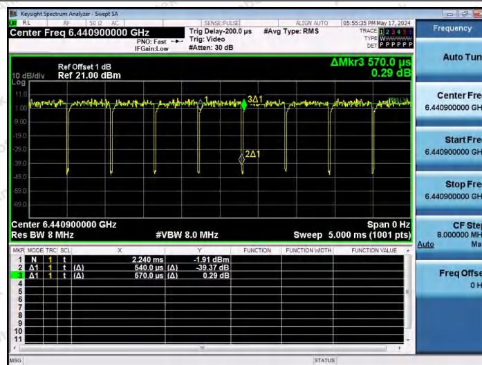
NTNV-11AX20SISO-Ant1-6435-52Tone-RU40
