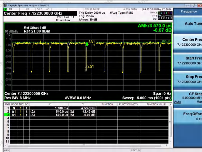
NTNV-11AX20SISO-Ant1-7115-52Tone-RU40
