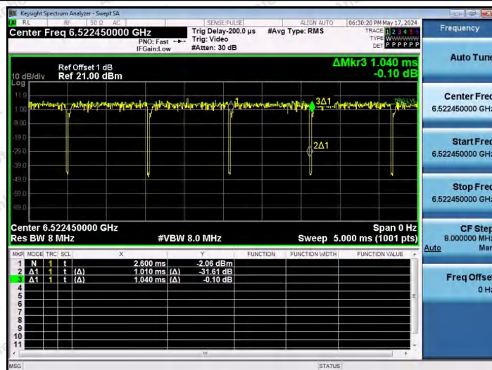
NTNV-11AX20SISO-Ant1-6515-26Tone-RU8
