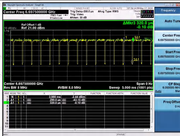
NTNV-11AX20SISO-Ant1-6695-106Tone-RU54
