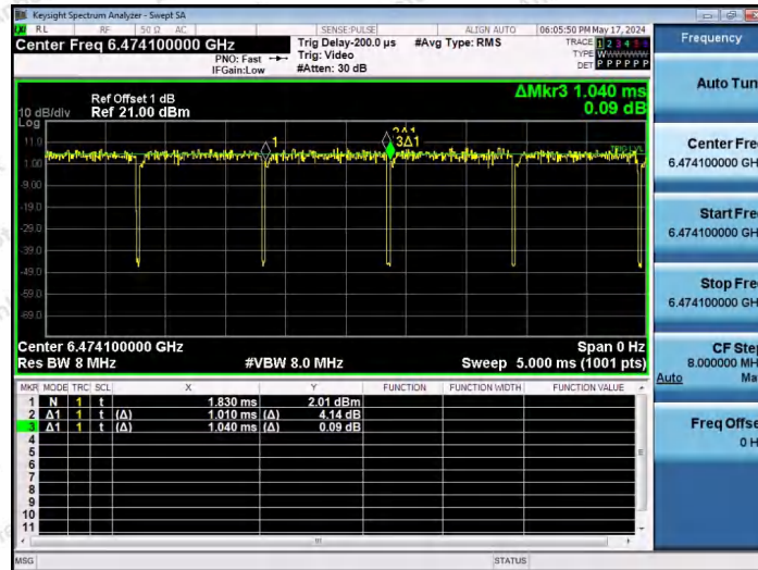
NTNV-11AX20SISO-Ant1-6475-26Tone-RU4
