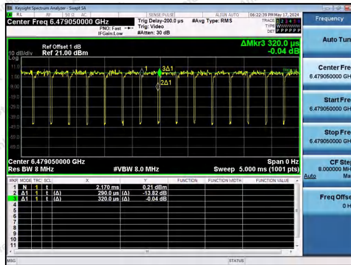
NTNV-11AX20SISO-Ant1-6475-106Tone-RU54
