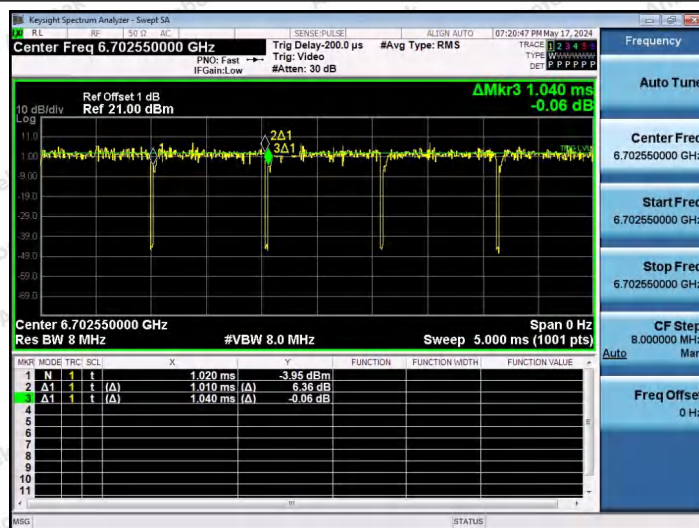
NTNV-11AX20SISO-Ant1-6695-26Tone-RU8
