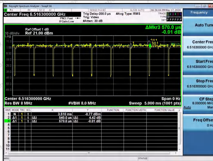
NTNV-11AX20SISO-Ant1-6515-52Tone-RU39
