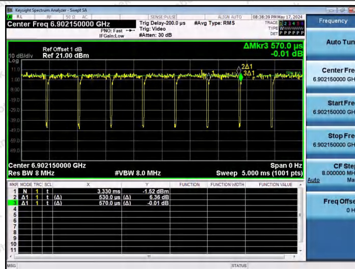
NTNV-11AX20SISO-Ant1-6895-52Tone-RU40
