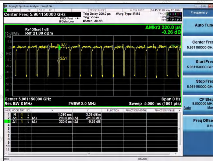
NTNV-11AX20SISO-Ant1-5955-106Tone-RU54
