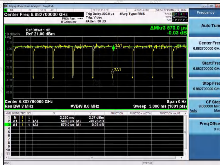
NTNV-11AX20SISO-Ant1-6875-52Tone-RU40
