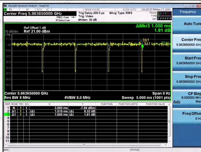
NTNV-11AX20SISO-Ant1-5955-26Tone-RU8
