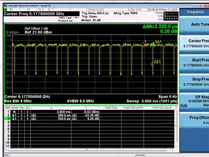
NTNV-11AX20SISO-Ant1-6175-106Tone-RU54
