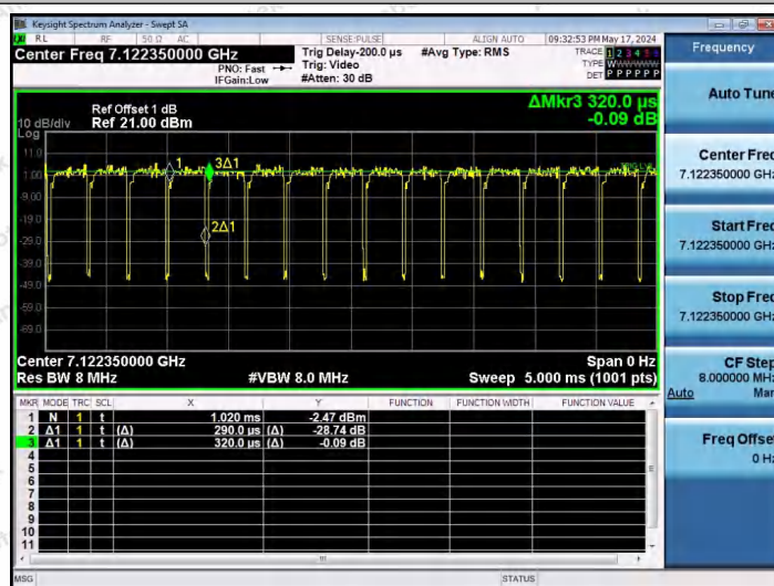
NTNV-11AX20SISO-Ant1-7115-106Tone-RU54
