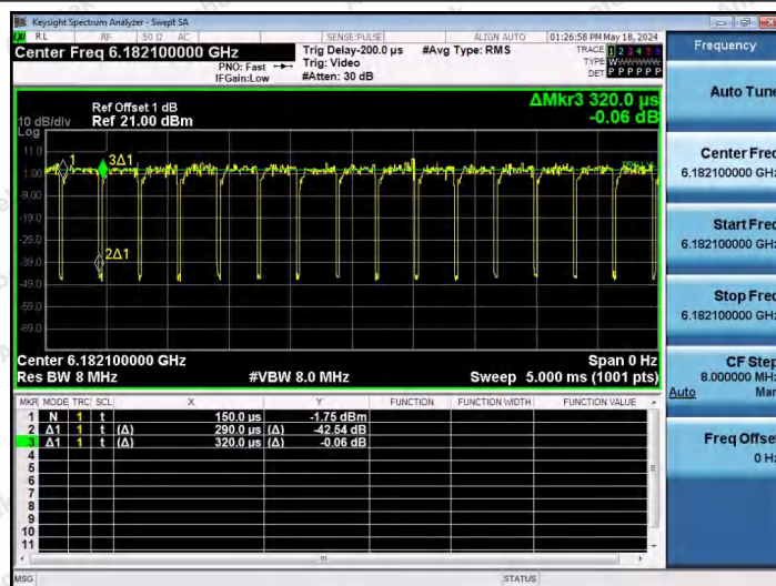
NTNV-11AX40SISO-Ant1-6165-106Tone-RU56
