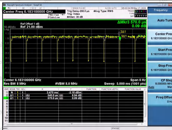
NTNV-11AX20SISO-Ant1-6175-52Tone-RU40
