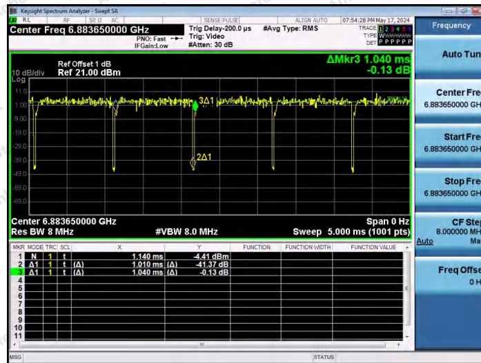
NTNV-11AX20SISO-Ant1-6875-26Tone-RU8
