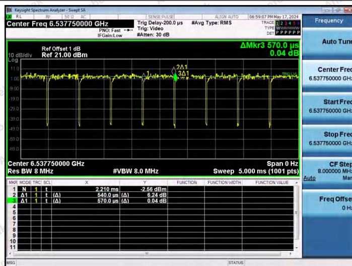
NTNV-11AX20SISO-Ant1-6535-52Tone-RU39
