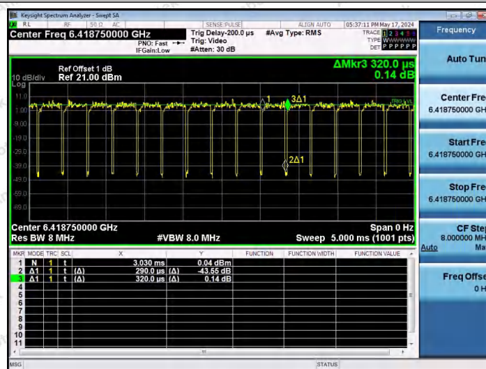
NTNV-11AX20SISO-Ant1-6415-106Tone-RU54
