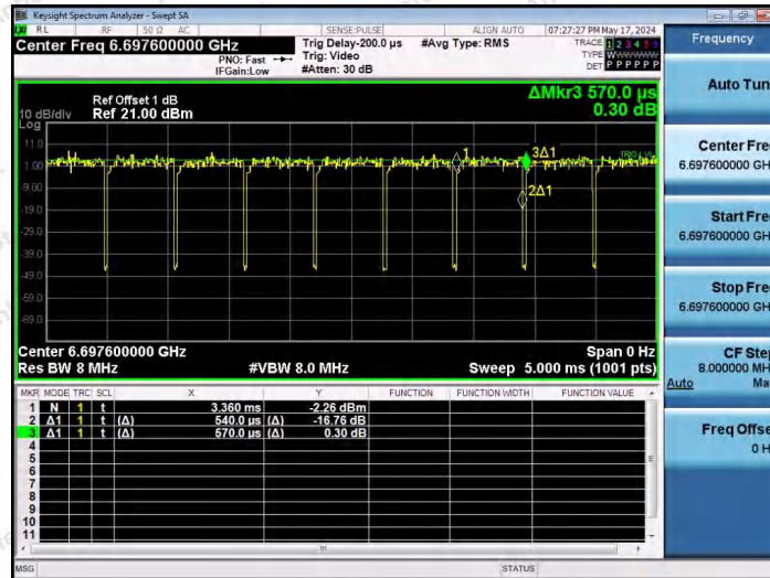
NTNV-11AX20SISO-Ant1-6695-52Tone-RU39
