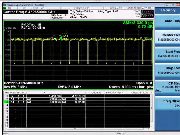
NTNV-11AX20SISO-Ant1-6435-106Tone-RU53
