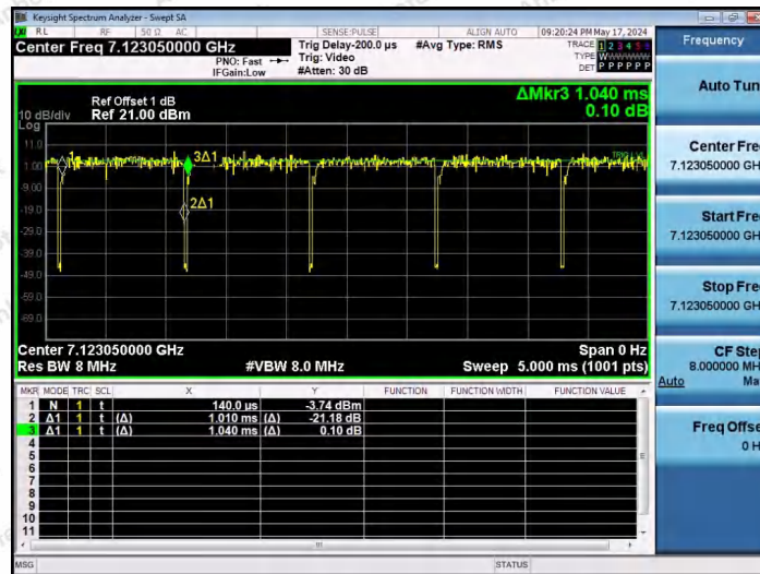
NTNV-11AX20SISO-Ant1-7115-26Tone-RU8
