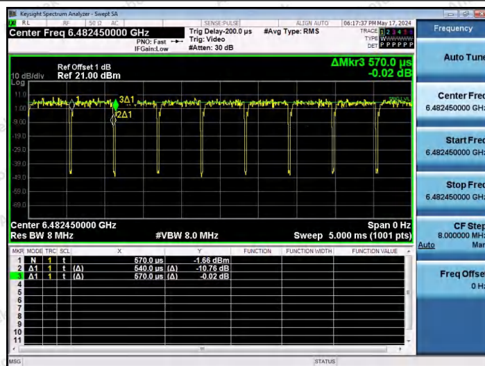
NTNV-11AX20SISO-Ant1-6475-52Tone-RU40
