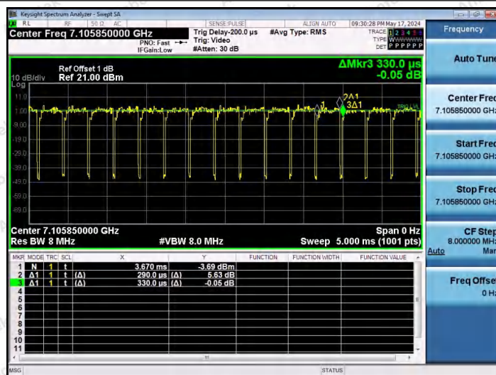
NTNV-11AX20SISO-Ant1-7115-106Tone-RU53
