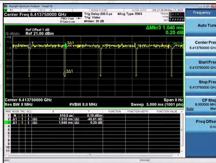
NTNV-11AX20SISO-Ant1-6415-26Tone-RU4
