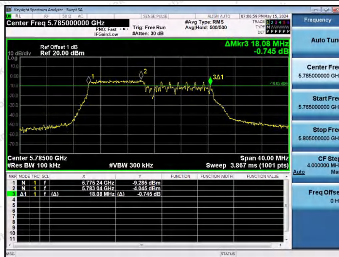
11AX20SISO-Ant1-5785-106Tone-RU53-PASS
