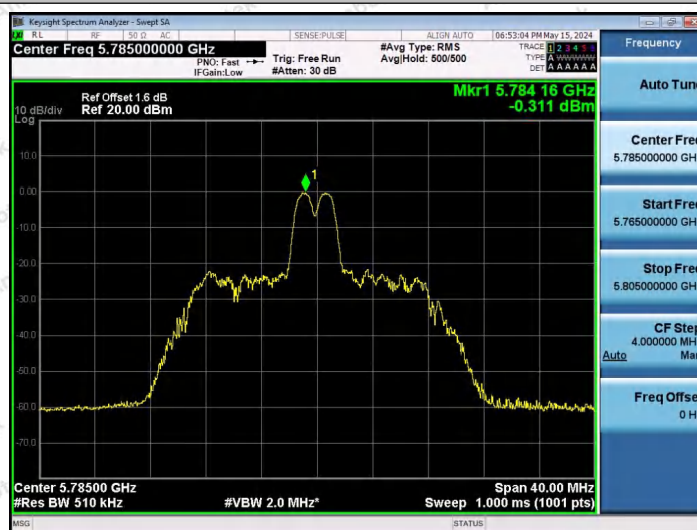
11AX20SISO-Ant1-5785-26Tone-RU4-PASS
