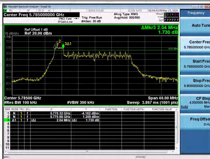
11AX20SISO-Ant1-5785-26Tone-RU0-PASS
