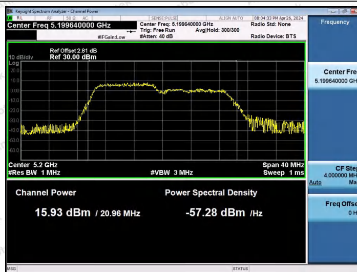
11AX20SISO-Ant1-5200-106Tone-RU53-PASS
