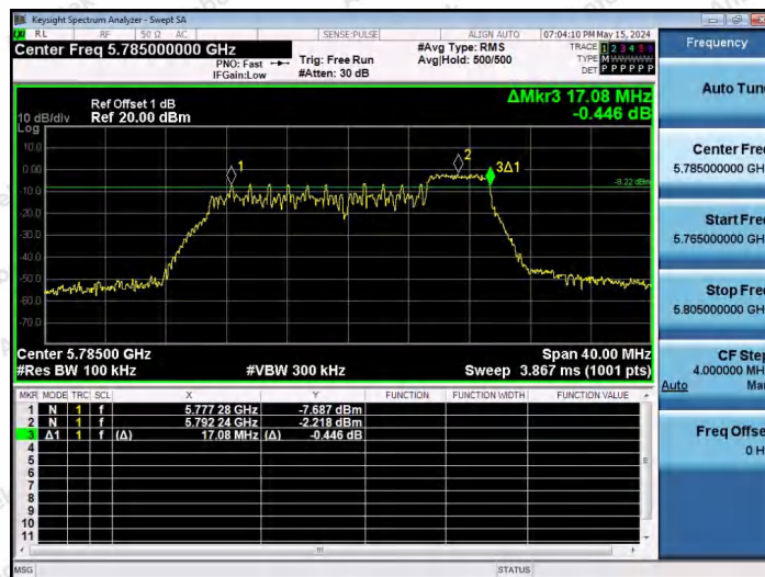
11AX20SISO-Ant1-5785-52Tone-RU40-PASS
