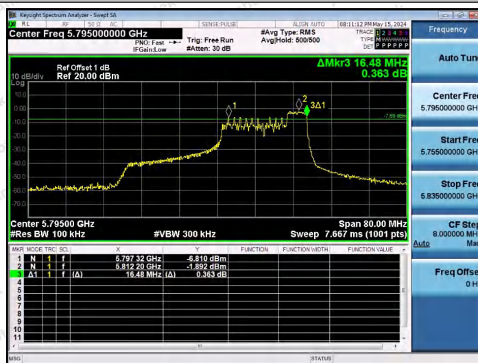
11AX40SISO-Ant1-5795-52Tone-RU44-PASS
