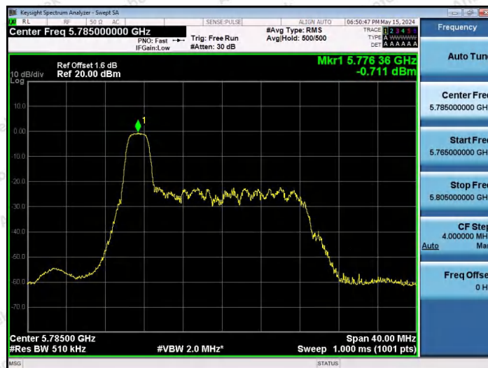
11AX20SISO-Ant1-5785-26Tone-RU0-PASS
