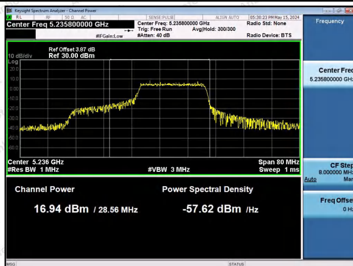
11AX40SISO-Ant1-5230-242Tone-RU62-PASS
