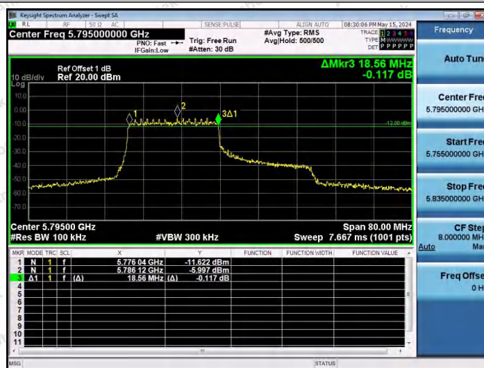
11AX40SISO-Ant1-5795-242Tone-RU61-PASS
