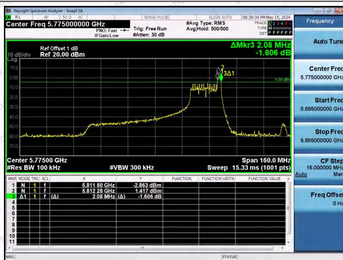
11AX80SISO-Ant1-5775-26Tone-RU36-PASS
