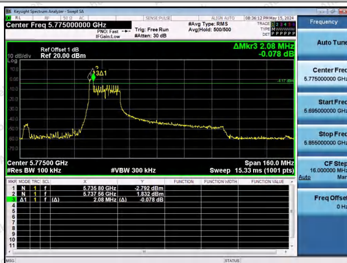
11AX80SISO-Ant1-5775-26Tone-RU0-PASS
