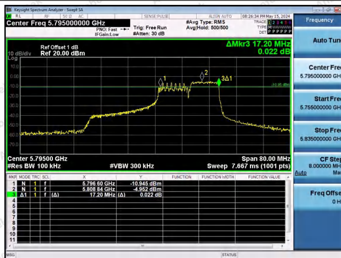
11AX40SISO-Ant1-5795-106Tone-RU56-PASS
