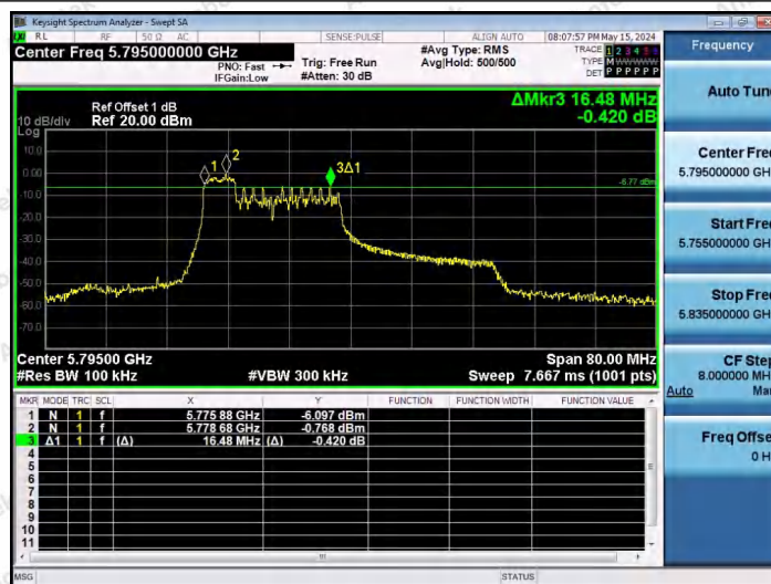
11AX40SISO-Ant1-5795-52Tone-RU37-PASS
