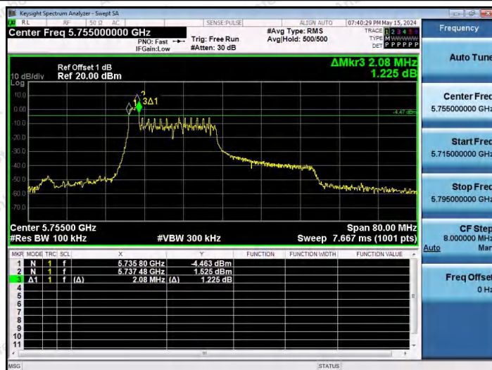
11AX40SISO-Ant1-5755-26Tone-RU0-PASS
