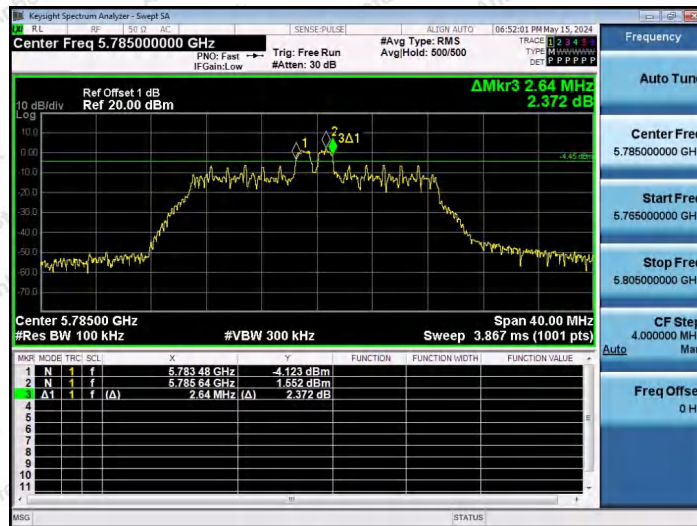
11AX20SISO-Ant1-5785-26Tone-RU4-PASS
