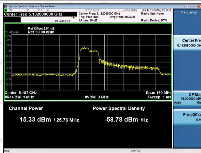
11AX80SISO-Ant1-5210-106Tone-RU53-PASS
