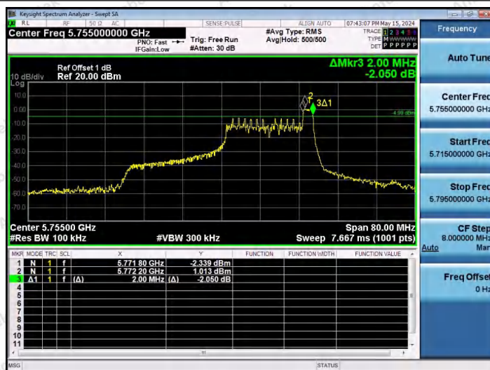
11AX40SISO-Ant1-5755-26Tone-RU17-PASS
