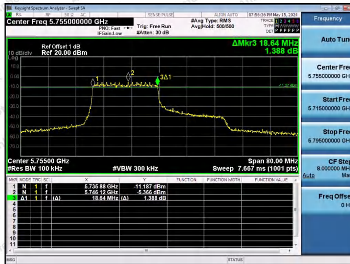
11AX40SISO-Ant1-5755-242Tone-RU61-PASS
