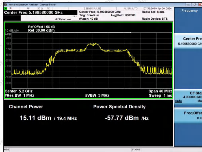
11AX20SISO-Ant1-5200-26Tone-RU4-PASS
