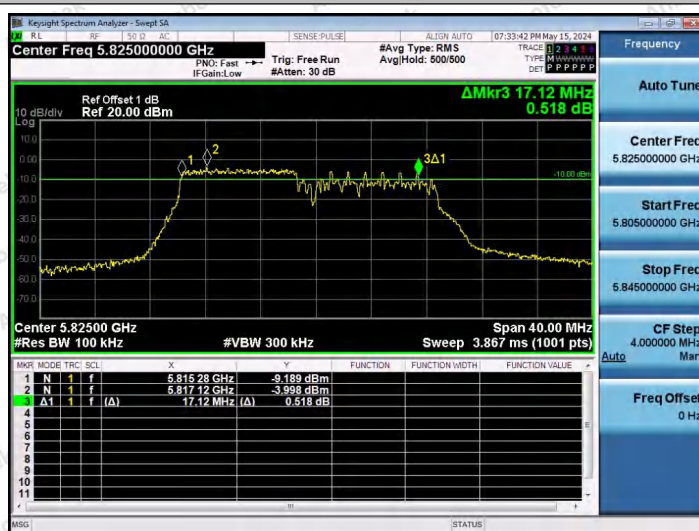
11AX20SISO-Ant1-5825-106Tone-RU53-PASS
