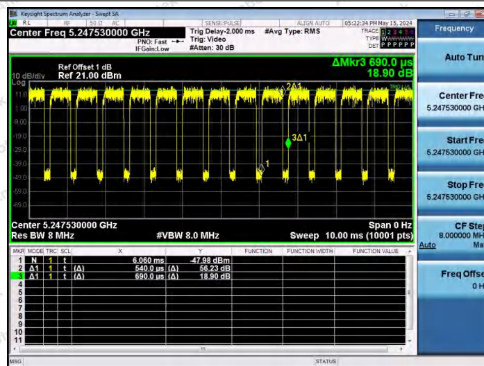
NTNV-11AX40SISO-Ant1-5230-52Tone-RU44
