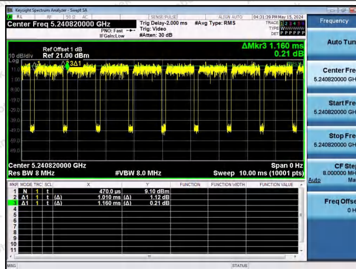
NTNV-11AX20SISO-Ant1-5240-26Tone-RU4
