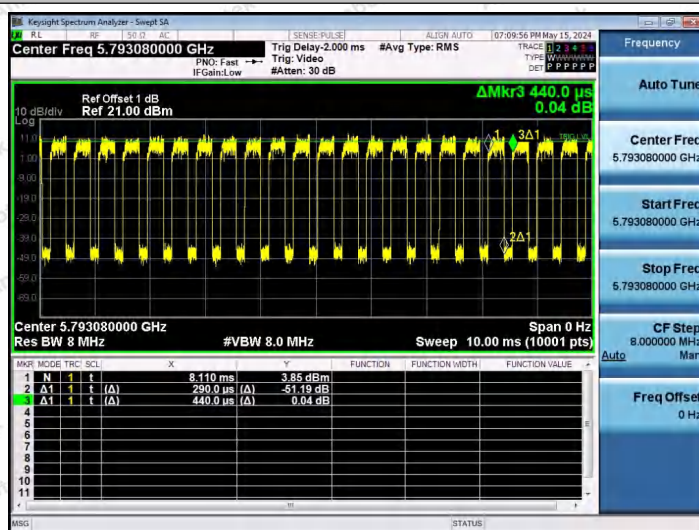
NTNV-11AX20SISO-Ant1-5785-106Tone-RU54
