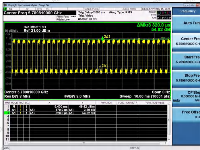
NTNV-11AX40SISO-Ant1-5795-242Tone-RU61
