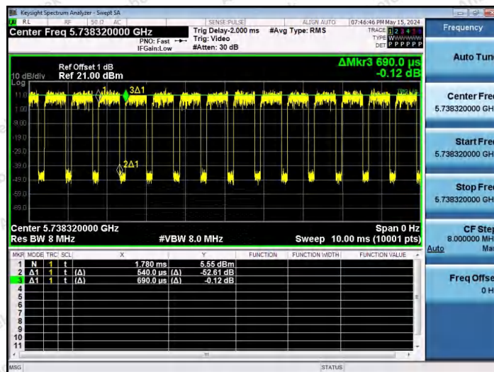
NTNV-11AX40SISO-Ant1-5755-52Tone-RU37
