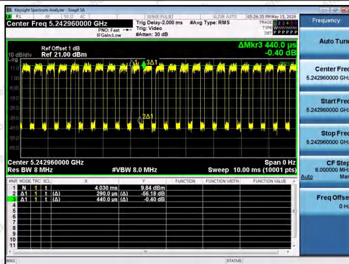
NTNV-11AX40SISO-Ant1-5230-106Tone-RU56
