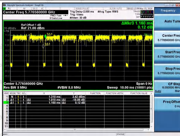
NTNV-11AX40SISO-Ant1-5795-26Tone-RU0
