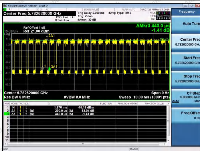
NTNV-11AX20SISO-Ant1-5785-106Tone-RU53
