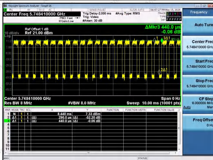
NTNV-11AX20SISO-Ant1-5745-106Tone-RU54
