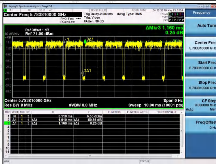
NTNV-11AX20SISO-Ant1-5785-26Tone-RU4
