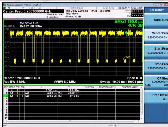
NTNV-11AX20SISO-Ant1-5200-52Tone-RU40
