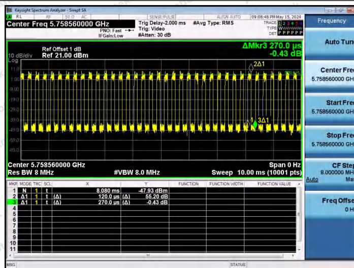
NTNV-11AX80SISO-Ant1-5775-484Tone-RU65
