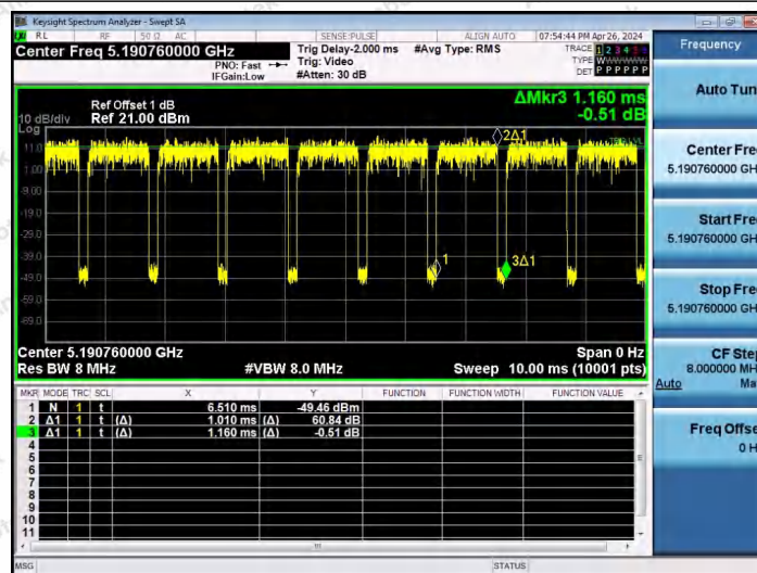
NTNV-11AX20SISO-Ant1-5200-26Tone-RU0
