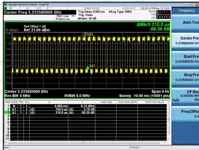
NTNV-11AX40SISO-Ant1-5230-242Tone-RU62
