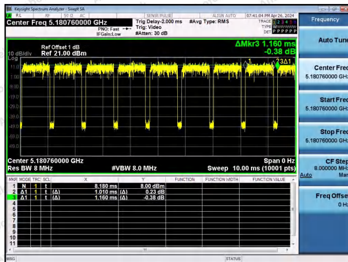
NTNV-11AX20SISO-Ant1-5180-26Tone-RU4
