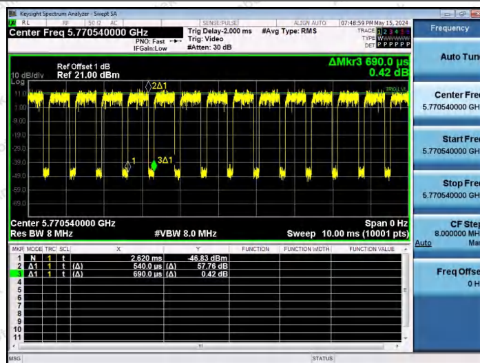
NTNV-11AX40SISO-Ant1-5755-52Tone-RU44
