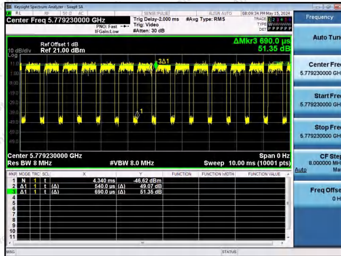
NTNV-11AX40SISO-Ant1-5795-52Tone-RU37
