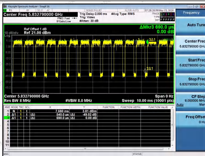
NTNV-11AX20SISO-Ant1-5825-52Tone-RU40
