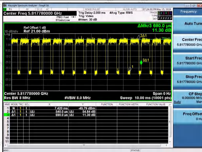
NTNV-11AX20SISO-Ant1-5825-52Tone-RU37
