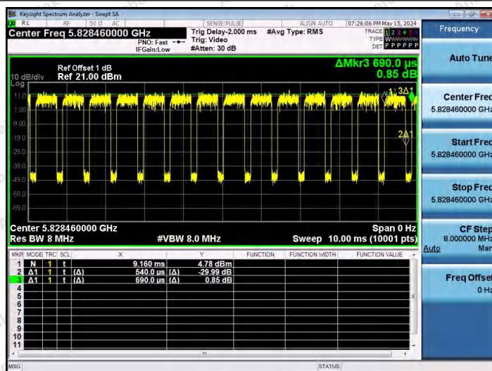
NTNV-11AX20SISO-Ant1-5825-52Tone-RU39
