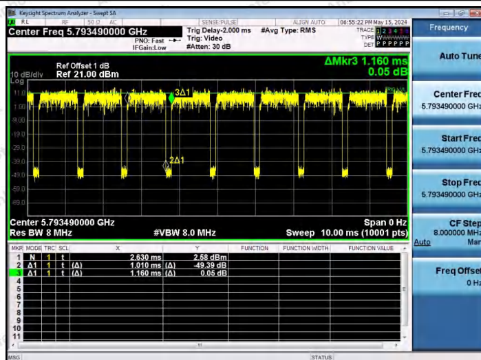
NTNV-11AX20SISO-Ant1-5785-26Tone-RU8
