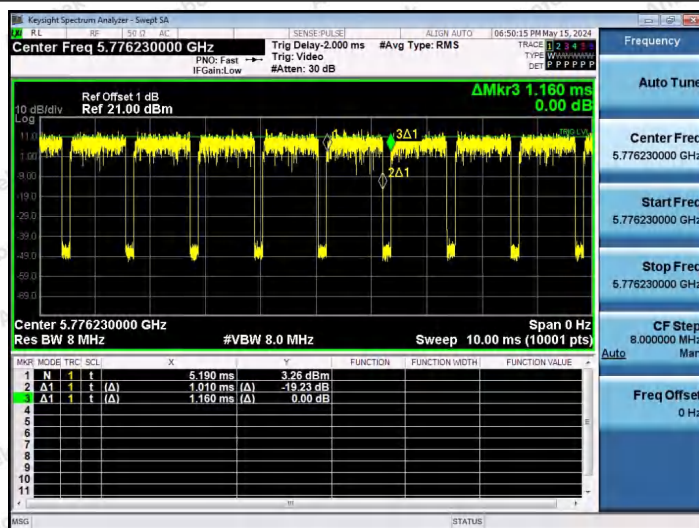
NTNV-11AX20SISO-Ant1-5785-26Tone-RU0
