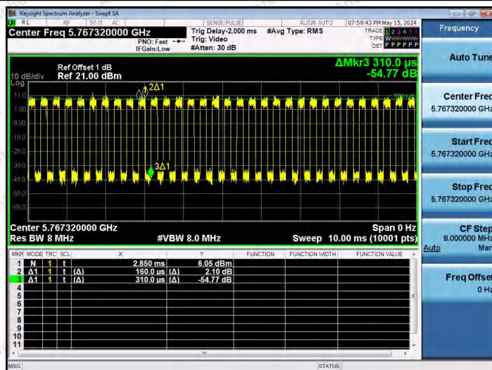
NTNV-11AX40SISO-Ant1-5755-242Tone-RU62
