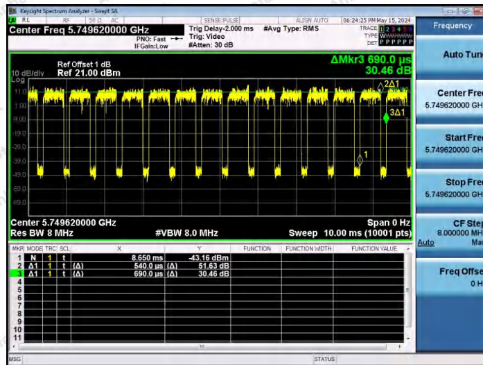
NTNV-11AX20SISO-Ant1-5745-52Tone-RU39
