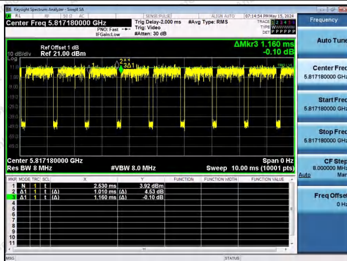
NTNV-11AX20SISO-Ant1-5825-26Tone-RU0
