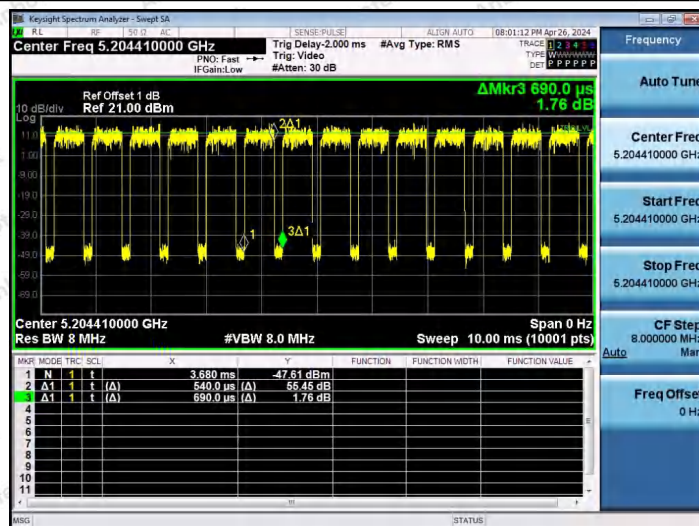
NTNV-11AX20SISO-Ant1-5200-52Tone-RU39
