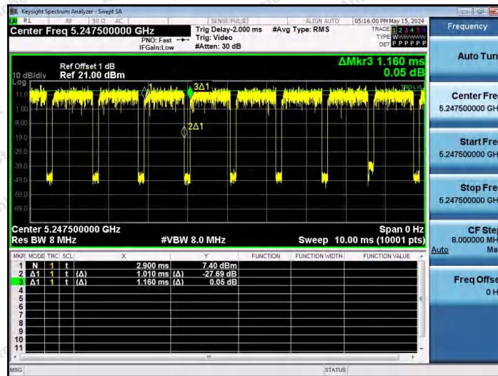
NTNV-11AX40SISO-Ant1-5230-26Tone-RU17
