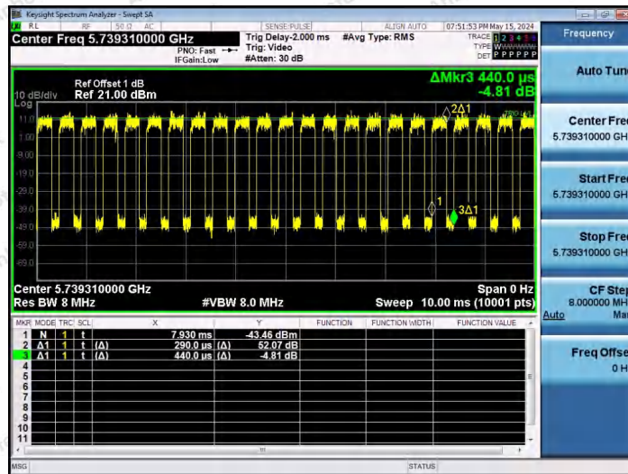
NTNV-11AX40SISO-Ant1-5755-106Tone-RU53
