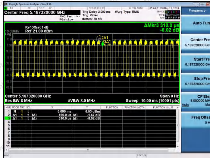
NTNV-11AX40SISO-Ant1-5190-242Tone-RU61
