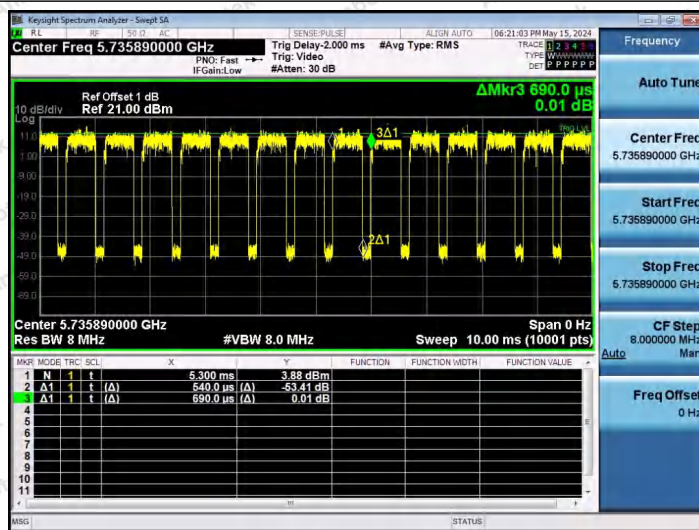
NTNV-11AX20SISO-Ant1-5745-52Tone-RU37
