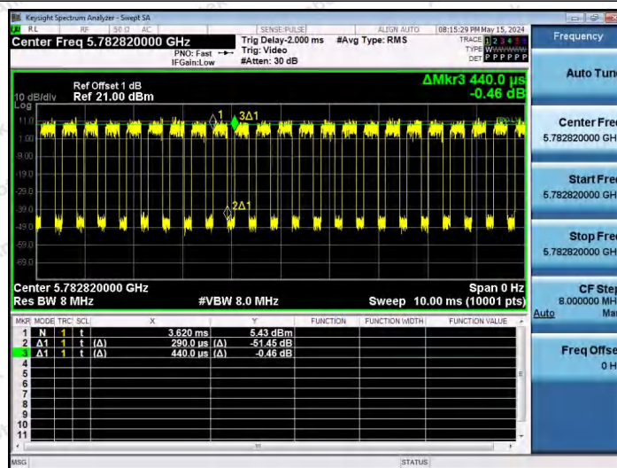
NTNV-11AX40SISO-Ant1-5795-106Tone-RU53
