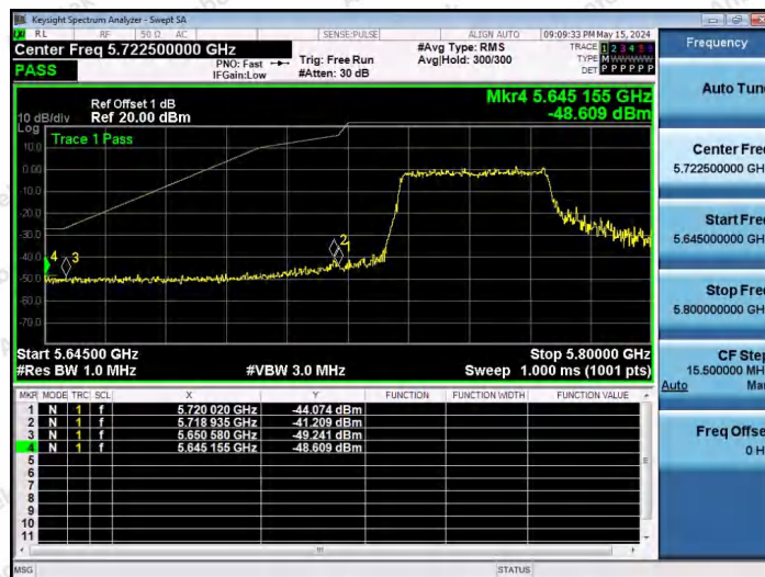
11AX80SISO-Ant1-5775-484Tone-RU65-PASS
