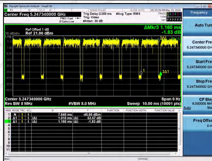
NTNV-11AX80SISO-Ant1-5210-26Tone-RU36
