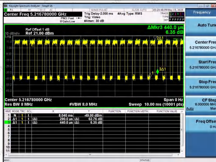
NTNV-11AX40SISO-Ant1-5230-106Tone-RU53
