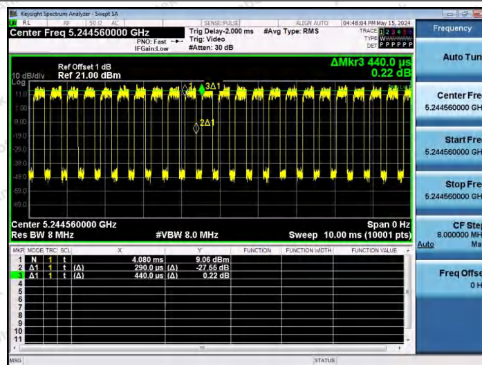
NTNV-11AX20SISO-Ant1-5240-106Tone-RU54
