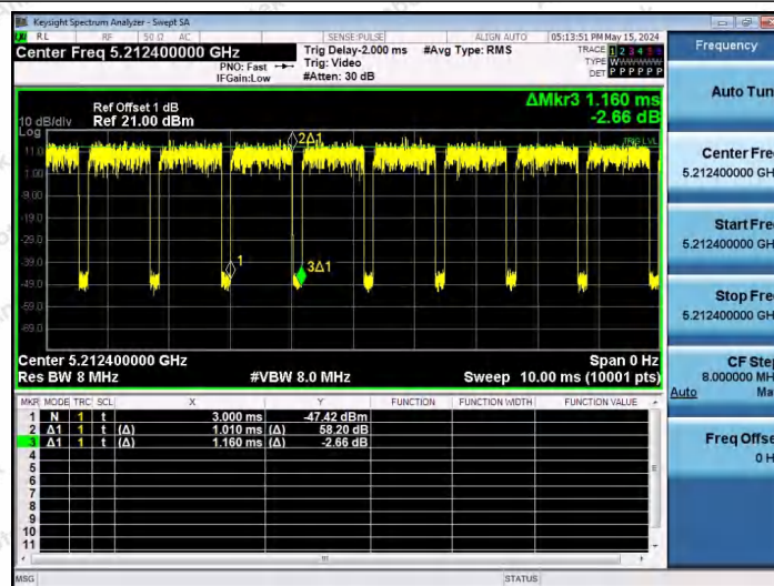
NTNV-11AX40SISO-Ant1-5230-26Tone-RU0
