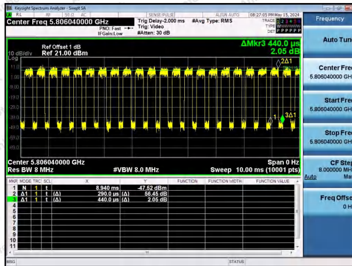
NTNV-11AX40SISO-Ant1-5795-106Tone-RU56
