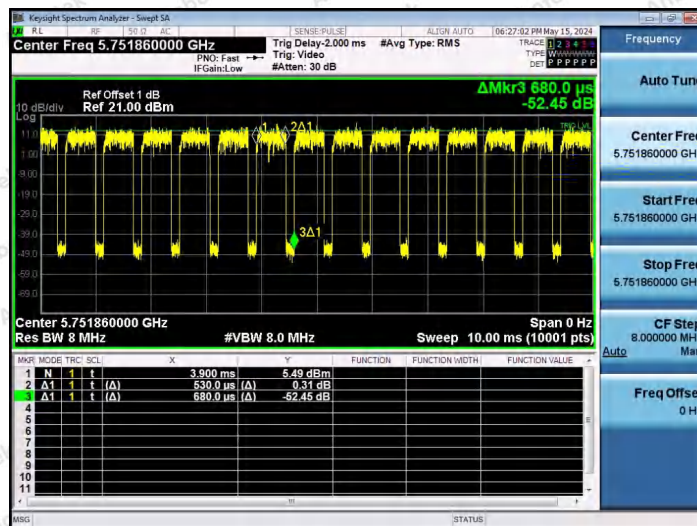
NTNV-11AX20SISO-Ant1-5745-52Tone-RU40
