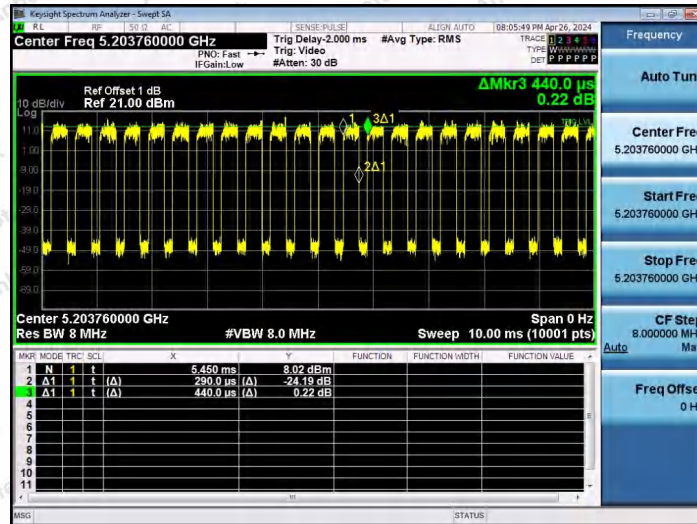
NTNV-11AX20SISO-Ant1-5200-106Tone-RU54
