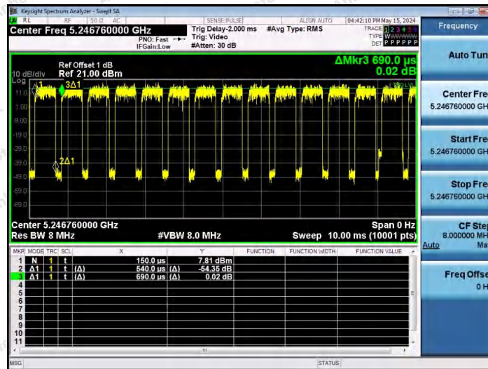
NTNV-11AX20SISO-Ant1-5240-52Tone-RU40
