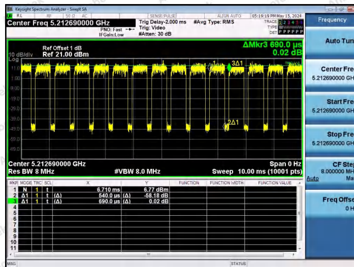
NTNV-11AX40SISO-Ant1-5230-52Tone-RU37
