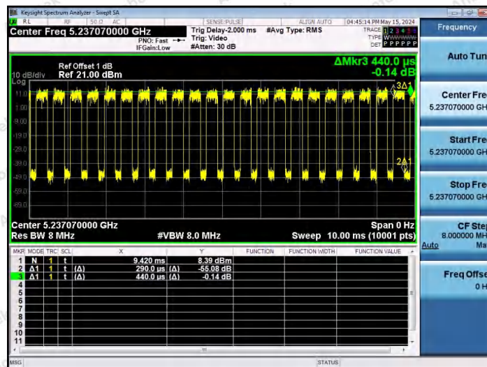
NTNV-11AX20SISO-Ant1-5240-106Tone-RU53
