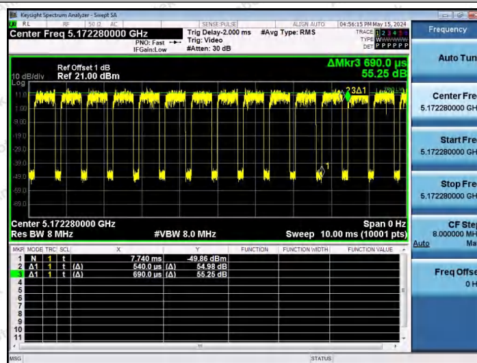
NTNV-11AX40SISO-Ant1-5190-52Tone-RU37
