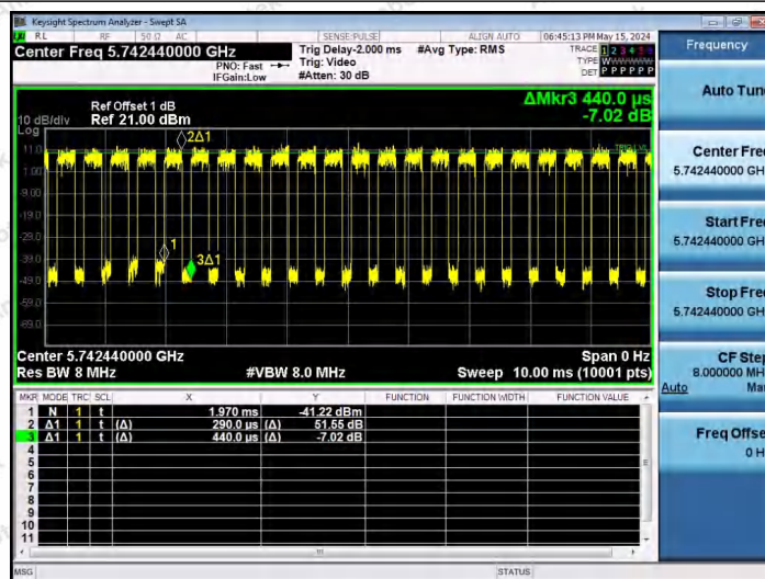
NTNV-11AX20SISO-Ant1-5745-106Tone-RU53
