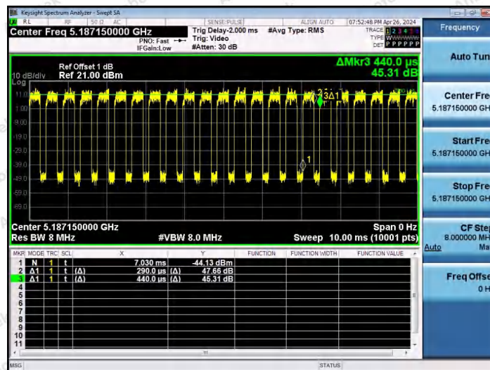
NTNV-11AX20SISO-Ant1-5180-106Tone-RU54
