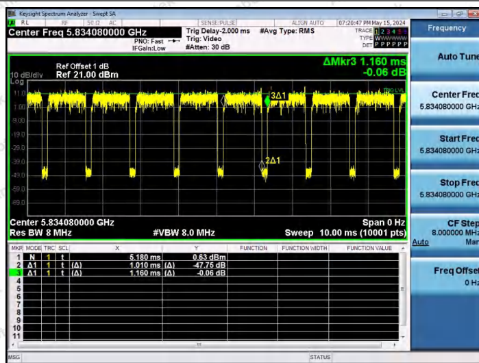
NTNV-11AX20SISO-Ant1-5825-26Tone-RU8
