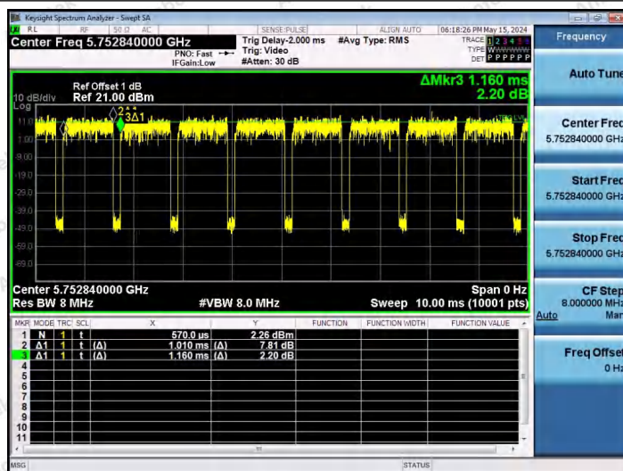
NTNV-11AX20SISO-Ant1-5745-26Tone-RU8
