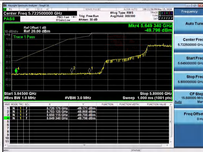
11AX80SISO-Ant1-5775-484Tone-RU66-PASS
