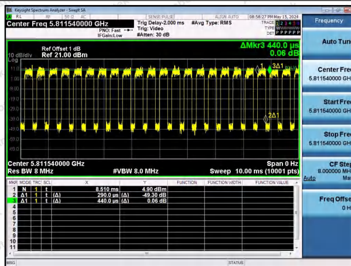
NTNV-11AX80SISO-Ant1-5775-106Tone-RU60
