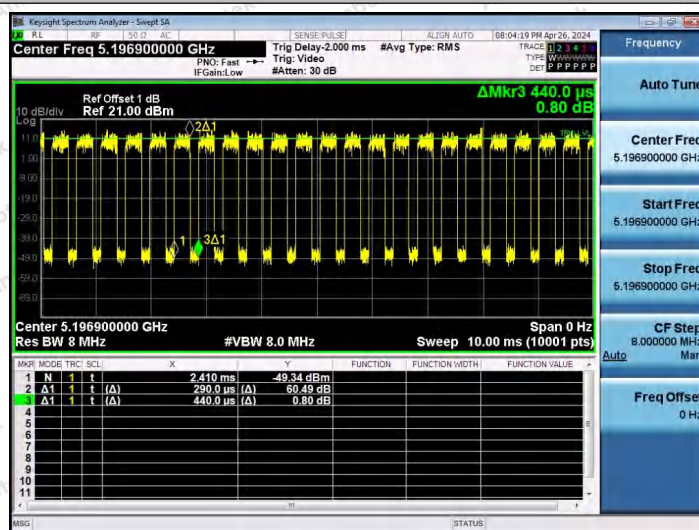
NTNV-11AX20SISO-Ant1-5200-106Tone-RU53
