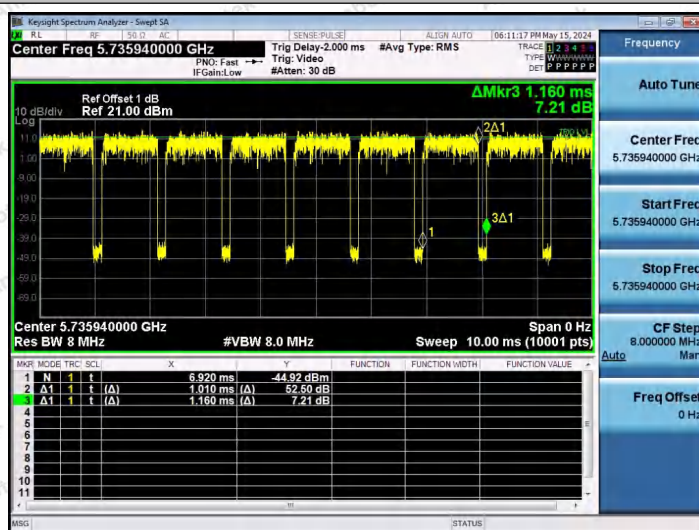
NTNV-11AX20SISO-Ant1-5745-26Tone-RU0
