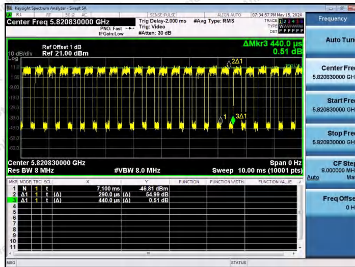
NTNV-11AX20SISO-Ant1-5825-106Tone-RU53
