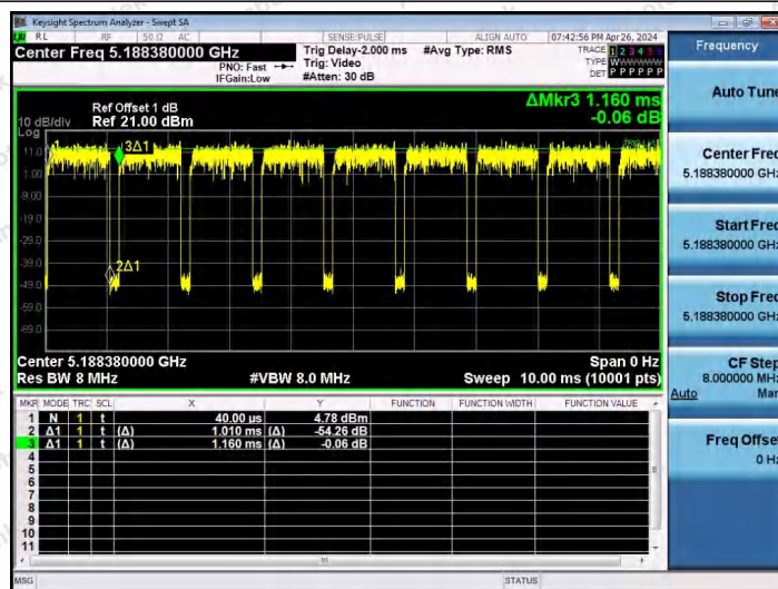
NTNV-11AX20SISO-Ant1-5180-26Tone-RU8
