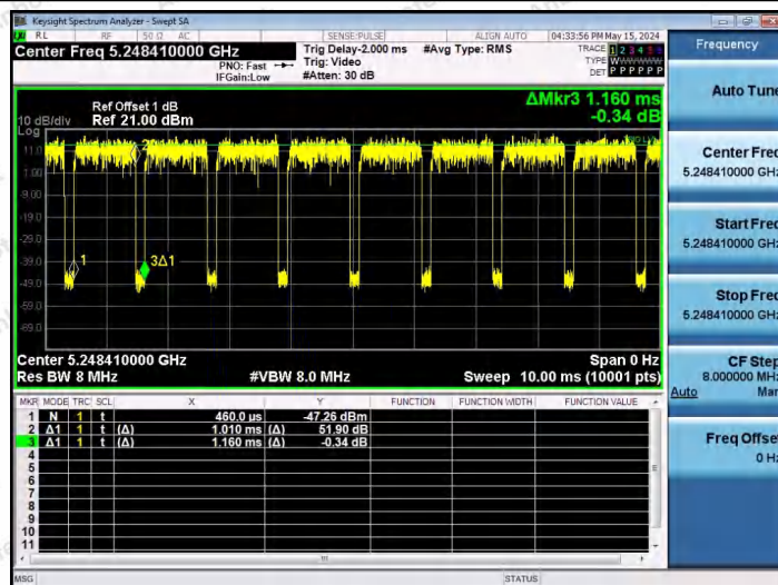
NTNV-11AX20SISO-Ant1-5240-26Tone-RU8
