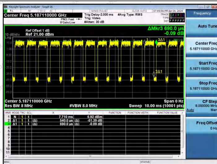
NTNV-11AX20SISO-Ant1-5180-52Tone-RU40
