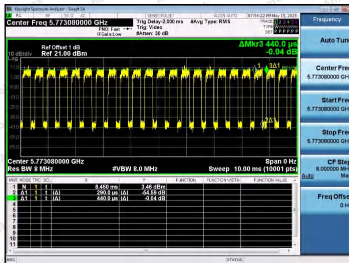
NTNV-11AX40SISO-Ant1-5755-106Tone-RU56
