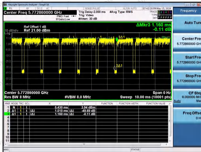
NTNV-11AX40SISO-Ant1-5755-26Tone-RU17
