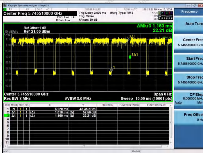
NTNV-11AX20SISO-Ant1-5745-26Tone-RU4
