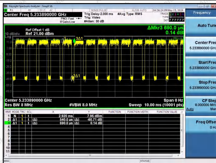
NTNV-11AX20SISO-Ant1-5240-52Tone-RU37
