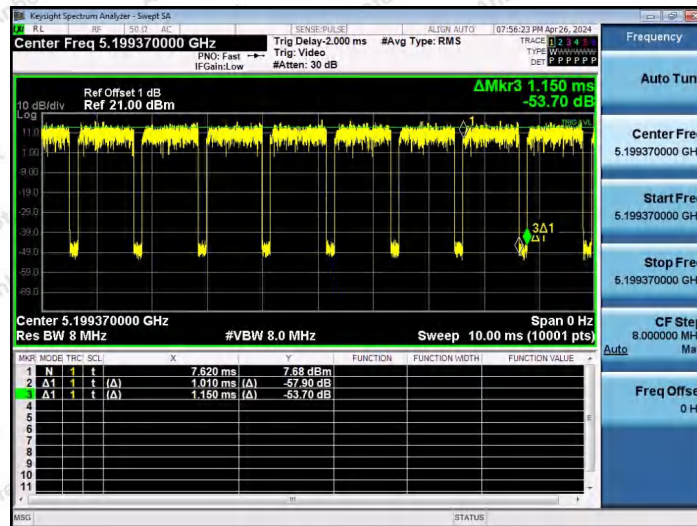
NTNV-11AX20SISO-Ant1-5200-26Tone-RU4
