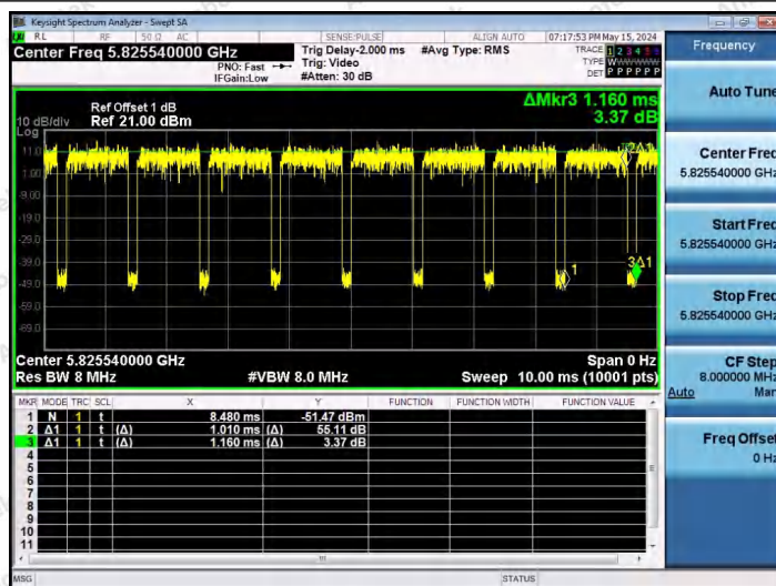
NTNV-11AX20SISO-Ant1-5825-26Tone-RU4
