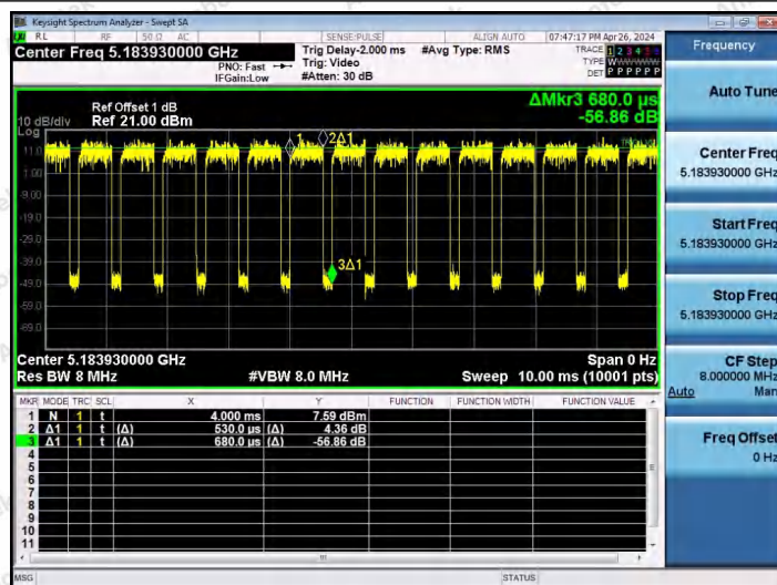
NTNV-11AX20SISO-Ant1-5180-52Tone-RU39
