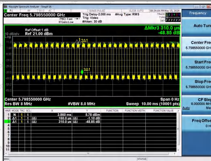
NTNV-11AX40SISO-Ant1-5795-242Tone-RU62
