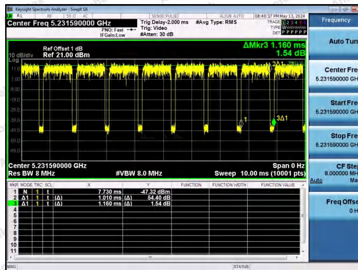
NTNV-11AX20SISO-Ant1-5240-26Tone-RU0
