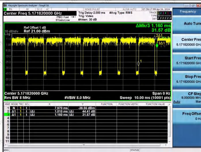
NTNV-11AX20SISO-Ant1-5180-26Tone-RU0
