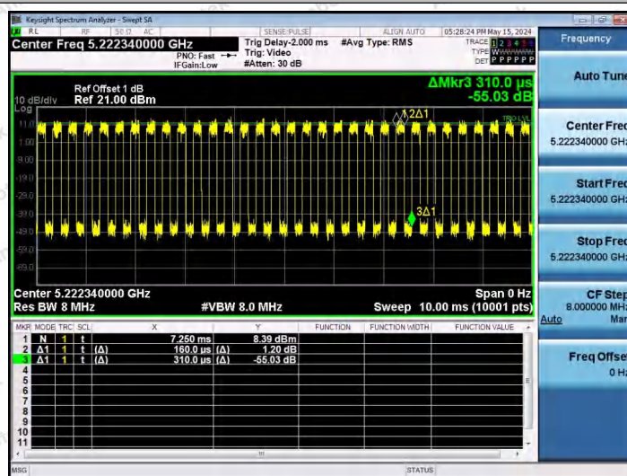
NTNV-11AX40SISO-Ant1-5230-242Tone-RU61
