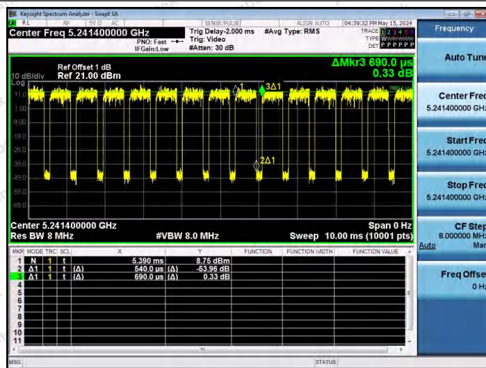
NTNV-11AX20SISO-Ant1-5240-52Tone-RU39
