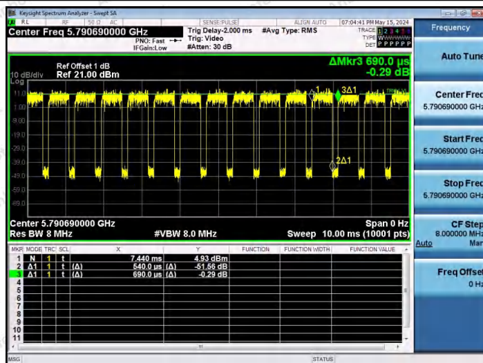
NTNV-11AX20SISO-Ant1-5785-52Tone-RU40
