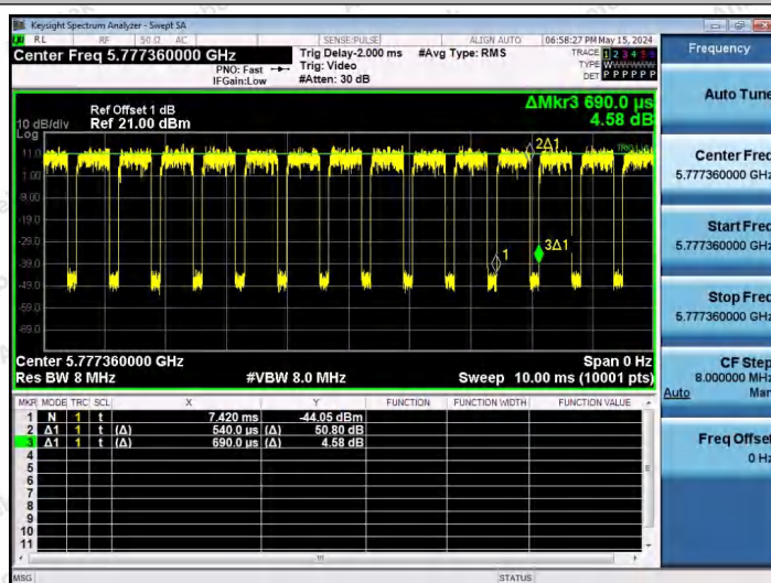
NTNV-11AX20SISO-Ant1-5785-52Tone-RU37
