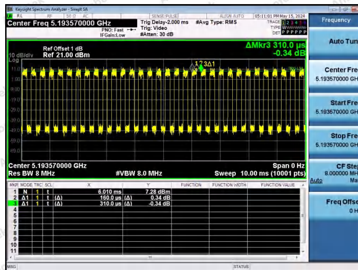
NTNV-11AX40SISO-Ant1-5190-242Tone-RU62
