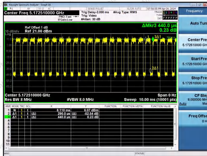
NTNV-11AX20SISO-Ant1-5180-106Tone-RU53
