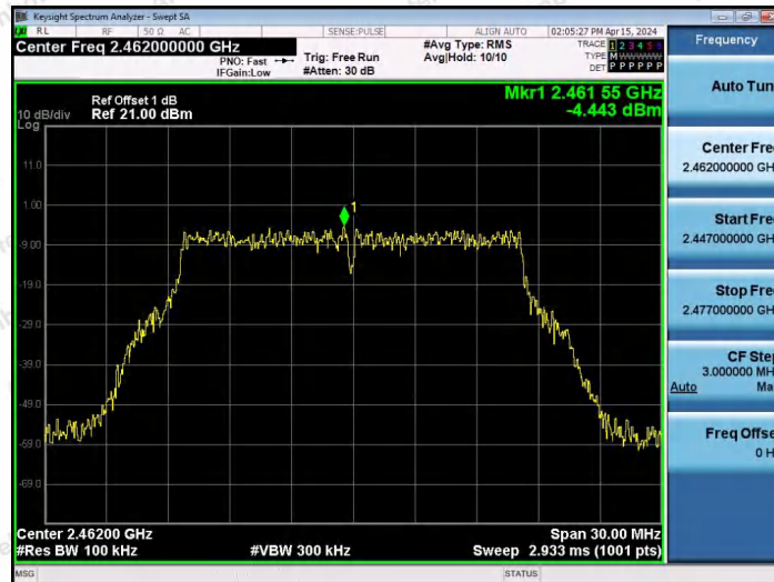
11G-Ant1-2462-0~Reference-PASS
