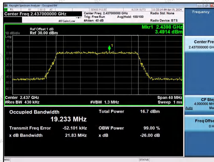
11AX20SISO-Ant1-2437
