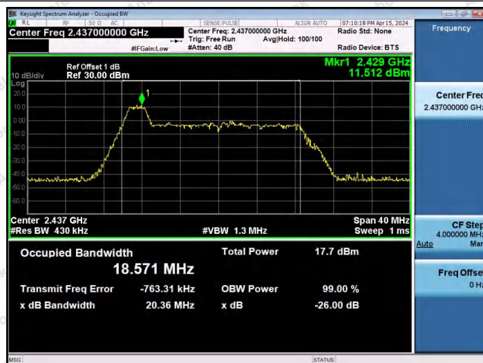
11AX20SISO-Ant1-2437-26Tone-RU0
