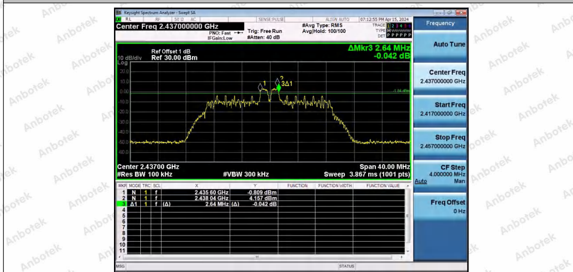
11AX20SISO-Ant1-2437-26Tone-RU0-PASS
