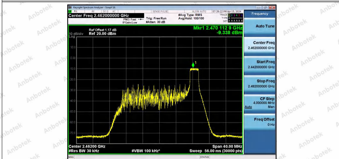
11AX20SISO-Ant1-2462-26Tone-RU8-PASS
