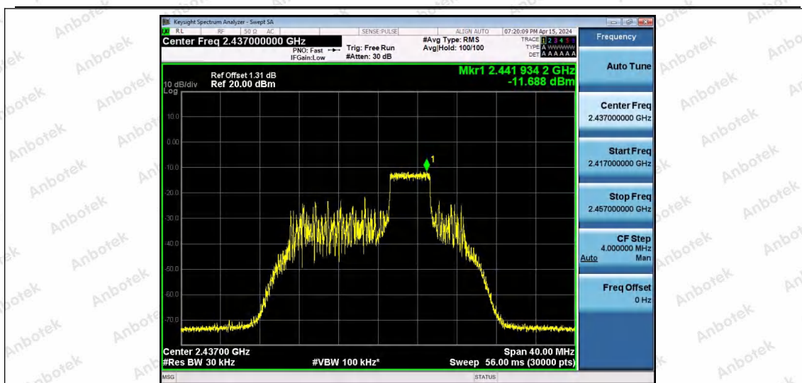
11AX20SISO-Ant1-2437-52Tone-RU39-PASS
