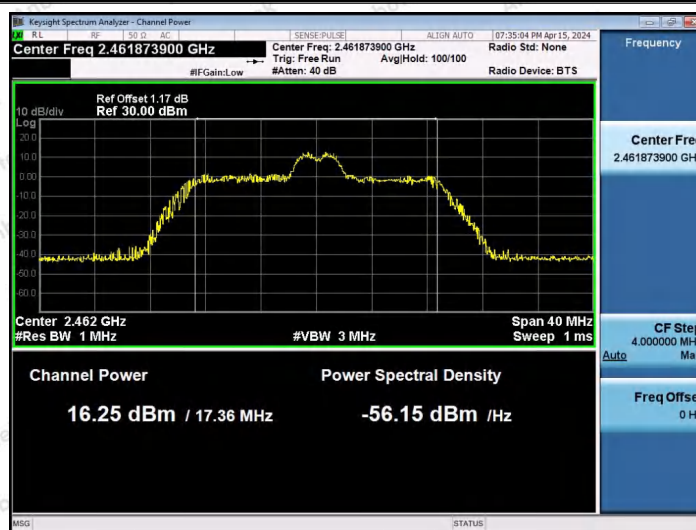
11AX20SISO-Ant1-2462-26Tone-RU4-PASS
