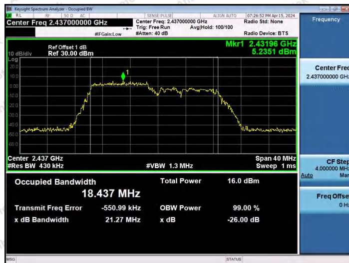
11AX20SISO-Ant1-2437-52Tone-RU40
