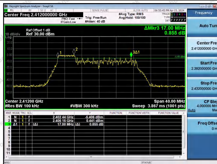
11AX20SISO-Ant1-2412-52Tone-RU37-PASS
