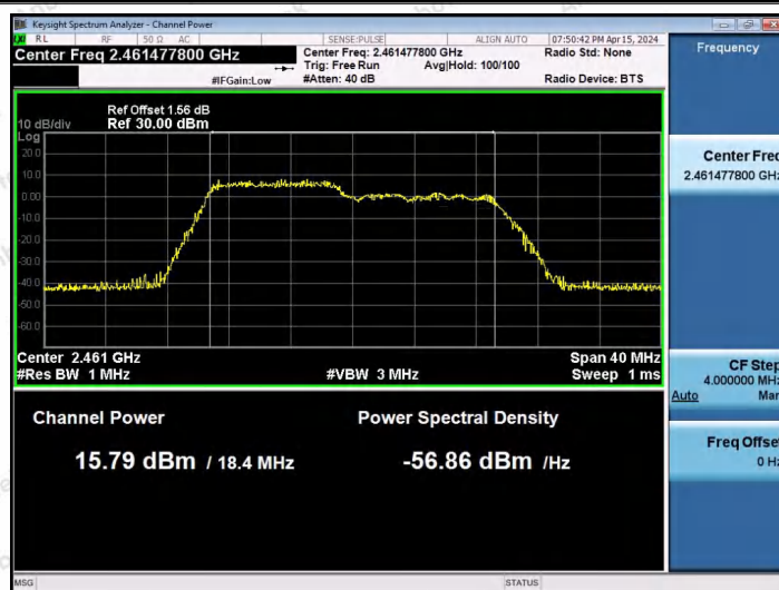
11AX20SISO-Ant1-2462-106Tone-RU53-PASS
