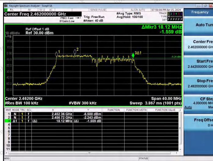
11AX20SISO-Ant1-2462-106Tone-RU53-PASS
