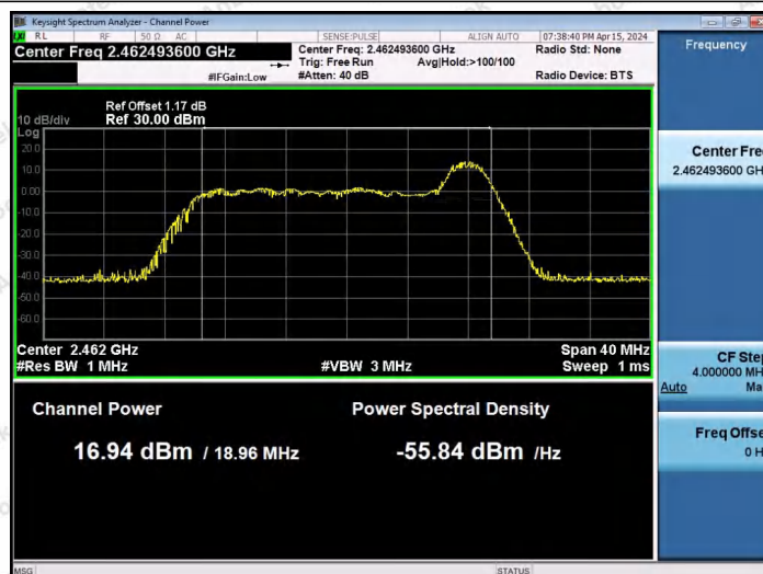
11AX20SISO-Ant1-2462-26Tone-RU8-PASS
