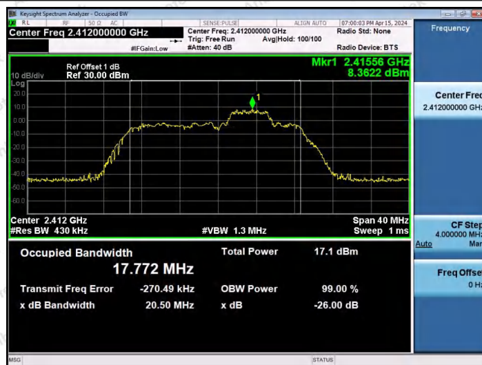
11AX20SISO-Ant1-2412-52Tone-RU37
