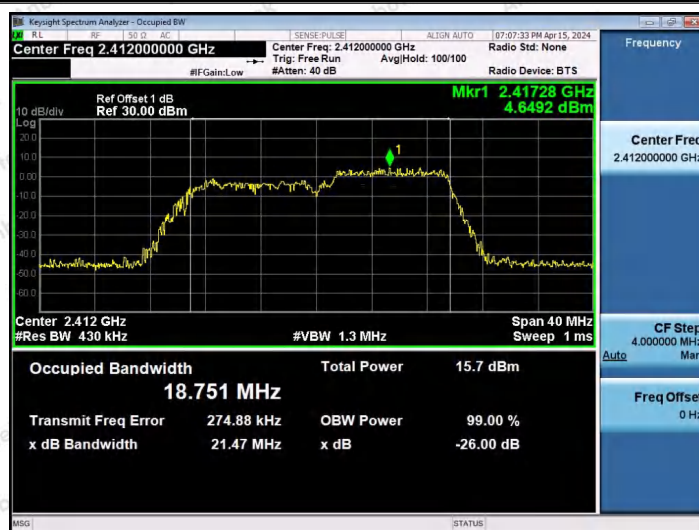
11AX20SISO-Ant1-2412-106Tone-RU54
