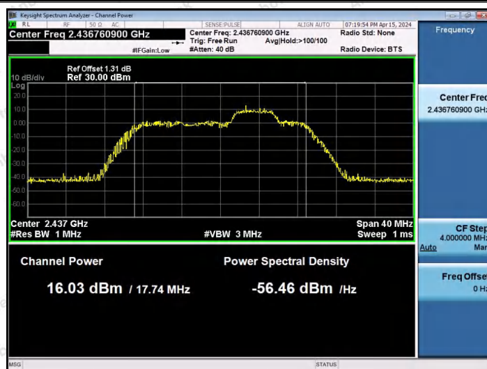
11AX20SISO-Ant1-2437-52Tone-RU39-PASS
