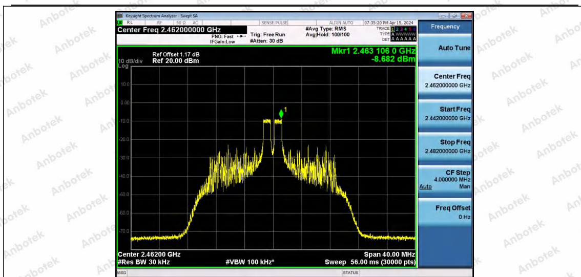
11AX20SISO-Ant1-2462-26Tone-RU4-PASS
