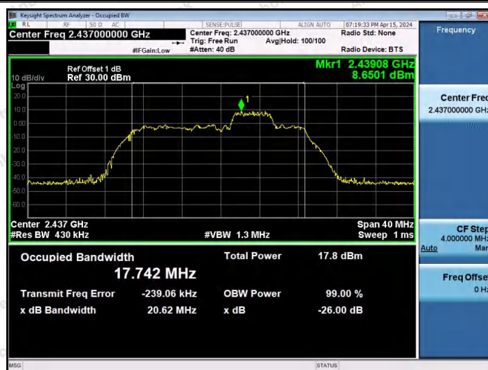
11AX20SISO-Ant1-2437-52Tone-RU39
