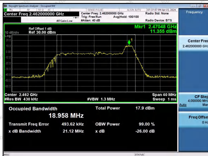
11AX20SISO-Ant1-2462-26Tone-RU8
