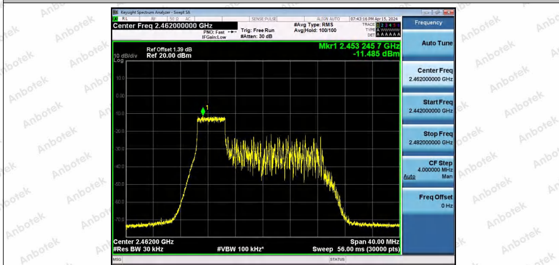
11AX20SISO-Ant1-2462-26Tone-RU8-PASS
