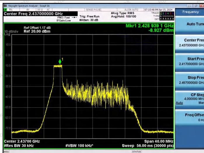
11AX20SISO-Ant1-2437-26Tone-RU0-PASS
