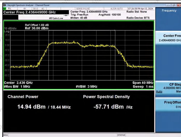
11AX20SISO-Ant1-2437-52Tone-RU40-PASS
