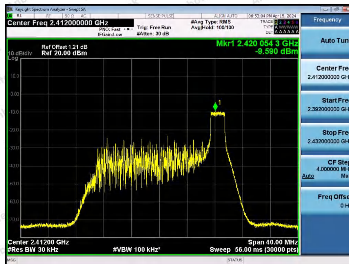
11AX20SISO-Ant1-2412-26Tone-RU8-PASS
