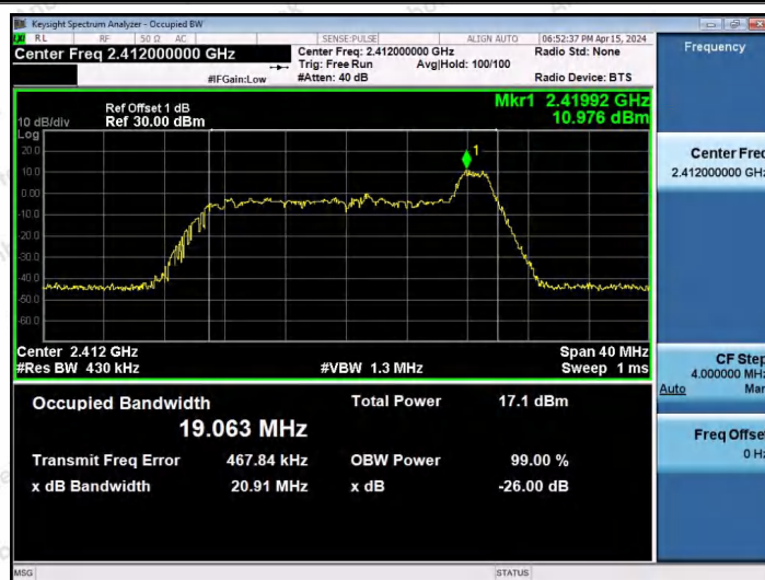
11AX20SISO-Ant1-2412-26Tone-RU8
