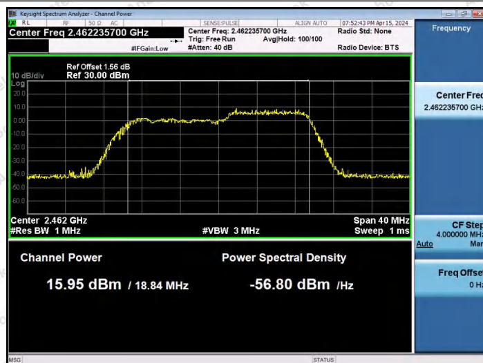
11AX20SISO-Ant1-2462-106Tone-RU54-PASS
