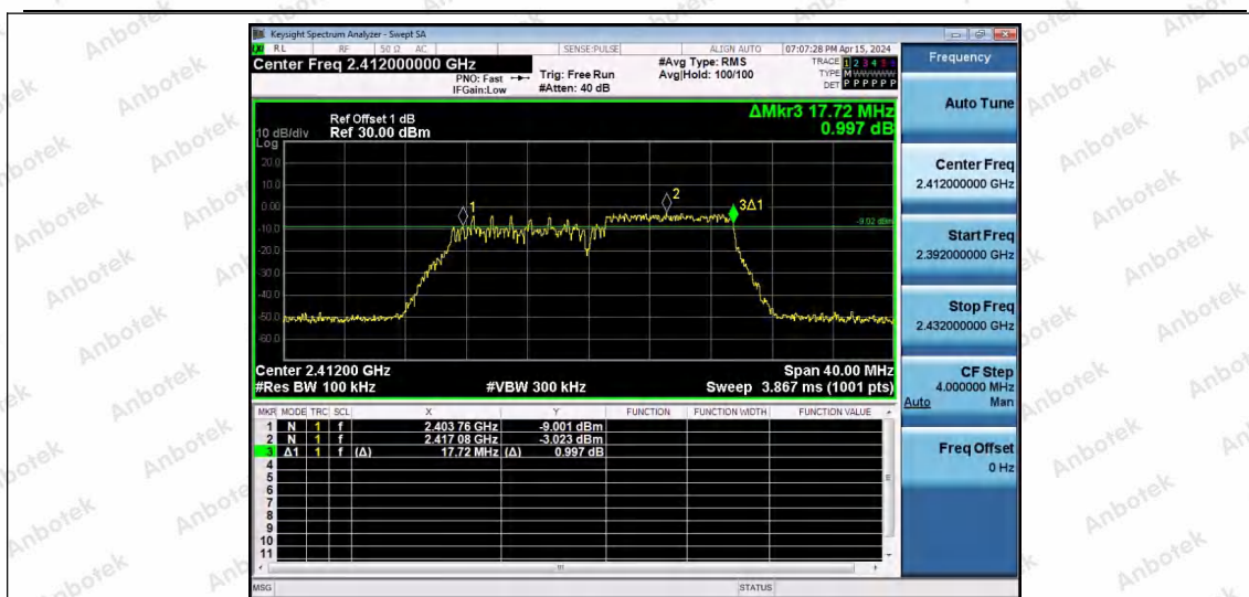
11AX20SISO-Ant1-2412-106Tone-RU54-PASS
