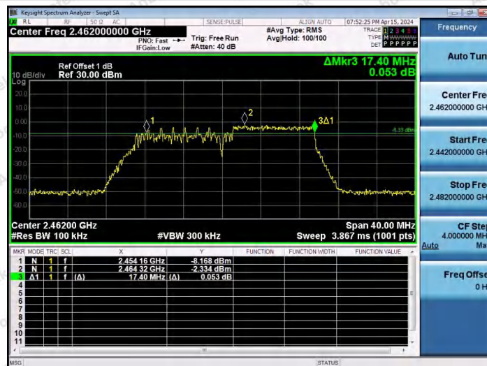
11AX20SISO-Ant1-2462-106Tone-RU54-PASS
