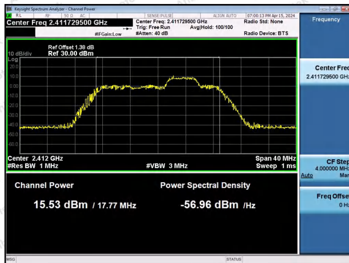
11AX20SISO-Ant1-2412-52Tone-RU37-PASS
