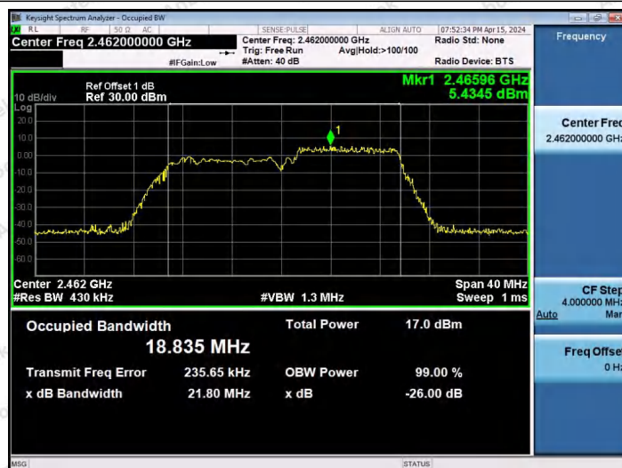
11AX20SISO-Ant1-2462-106Tone-RU54
