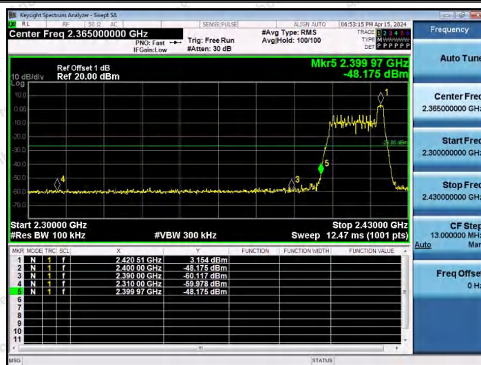
11AX20SISO-Ant1-2412-26Tone-RU8-PASS
