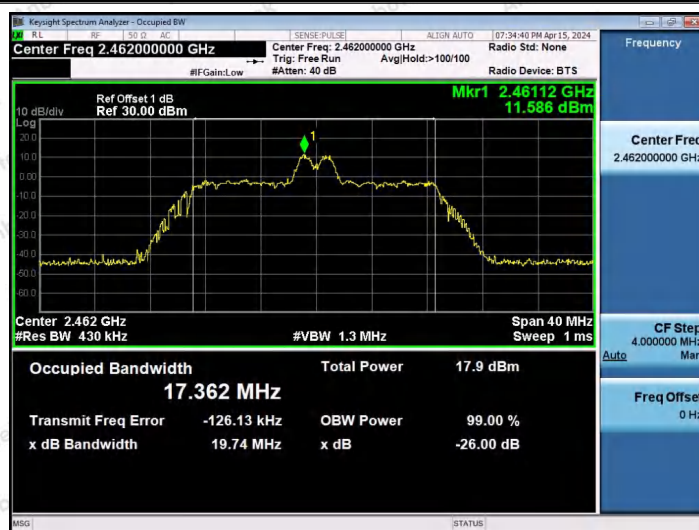
11AX20SISO-Ant1-2462-26Tone-RU4
