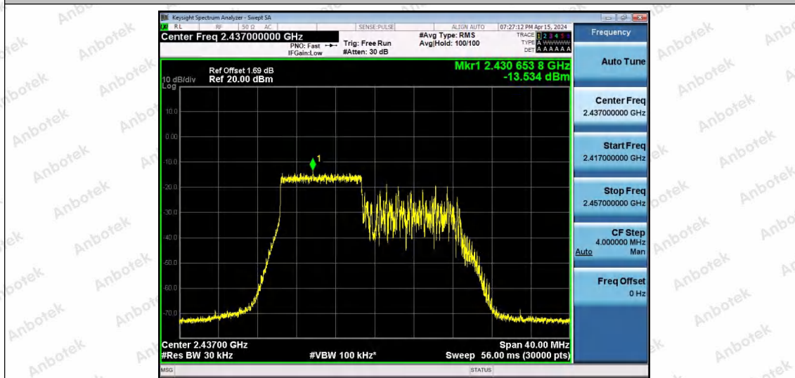
11AX20SISO-Ant1-2437-52Tone-RU40-PASS
