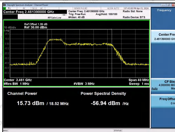
11AX20SISO-Ant1-2462-26Tone-RU8-PASS
