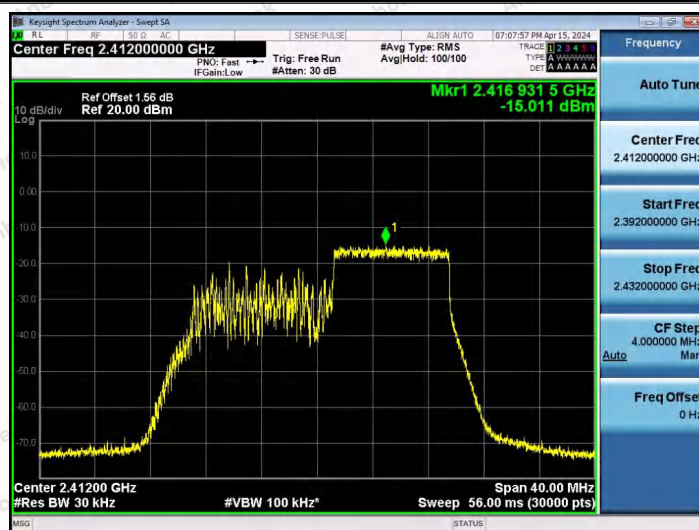
11AX20SISO-Ant1-2412-106Tone-RU54-PASS
