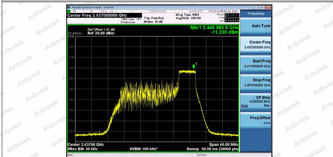
11AX20SISO-Ant1-2437-52Tone-RU40-PASS
