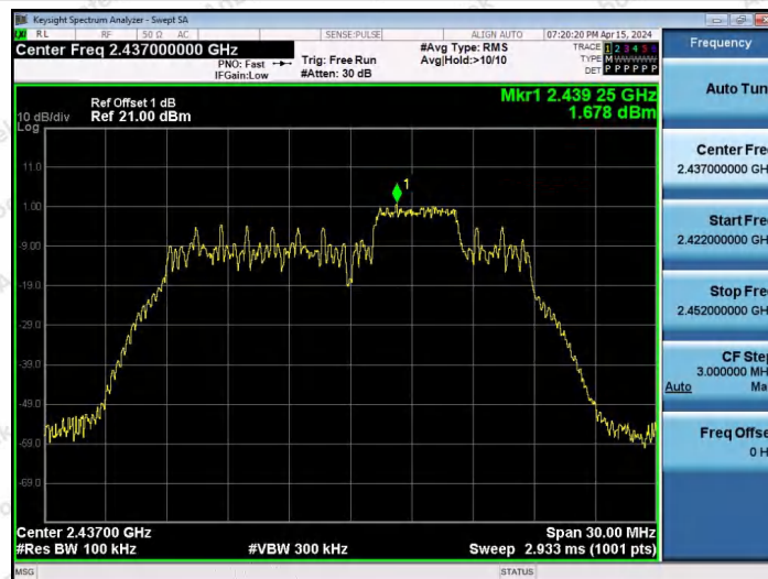
11AX20ISO-Ant1-2437-52Tone-RU39-0~Reference-PASS
