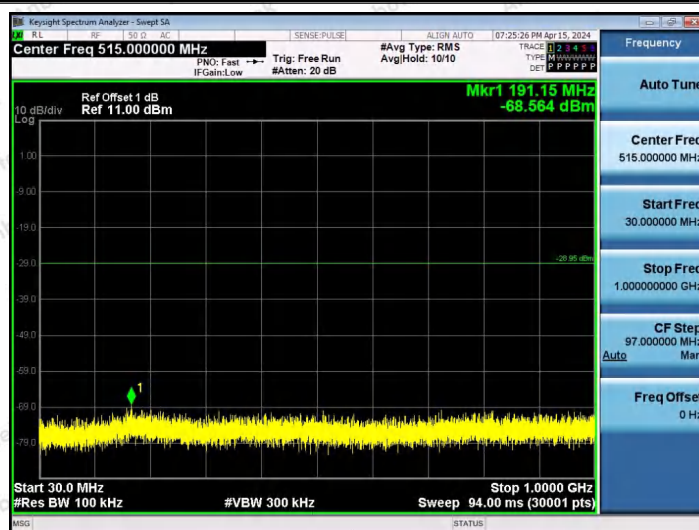
11AX20SISO-Ant1-2437-52Tone-RU40-30~1000-PASS
