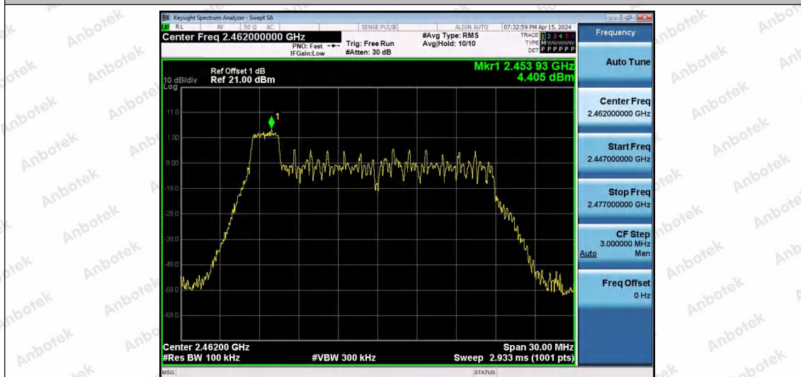
11AX20SISO-Ant1-2462-26Tone-RU0-0~Reference-PASS
