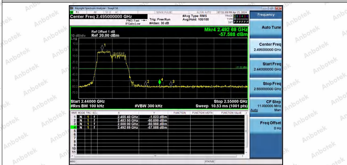
11AX20SISO-Ant1-2462-52Tone-RU40-PASS
