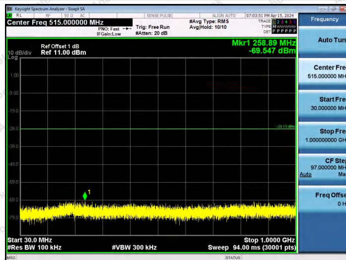
11AX20SISO-Ant1-2412-52Tone-RU40-30~1000-PASS
