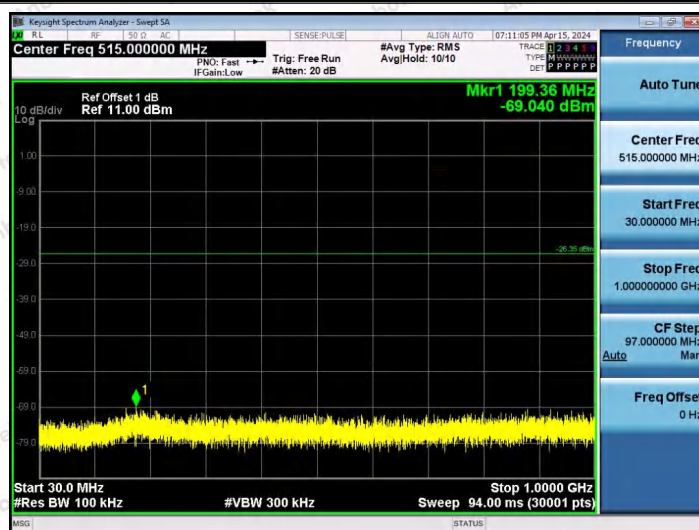
11AX20SISO-Ant1-2437-26Tone-RU0-30~1000-PASS
