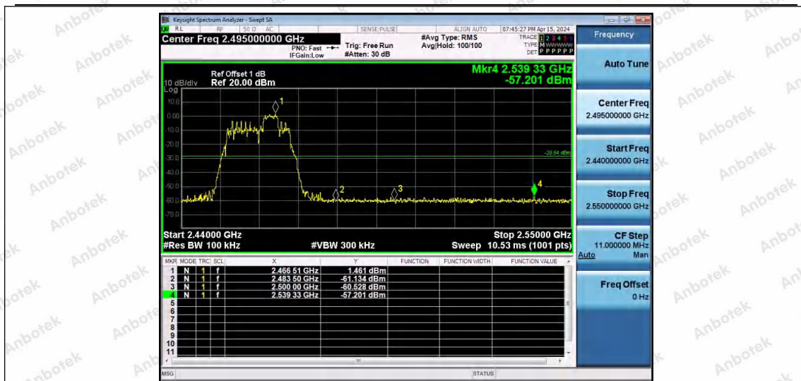
11AX20SISO-Ant1-2462-52Tone-RU39-PASS
