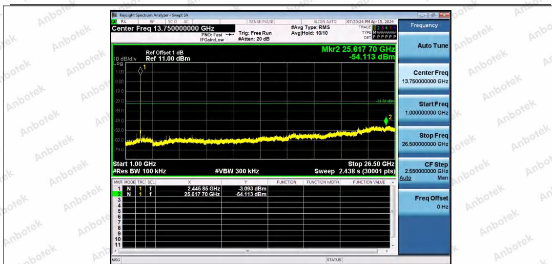
11AX20SISO-Ant1-2437-106Tone-RU54-1000~26500-PASS
