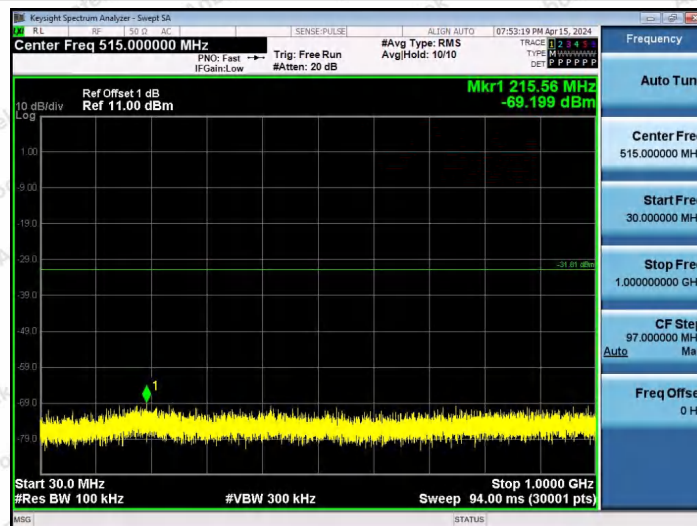
11AX20SISO-Ant1-2462-106Tone-RU54-30~1000-PASS
