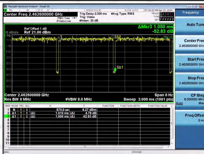
NTNV-11AX20SISO-Ant1-2462-26Tone-RU4
