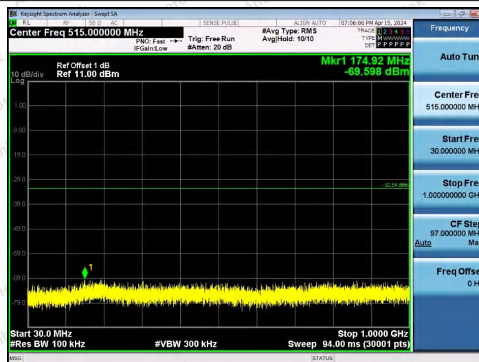
11AX20SISO-Ant1-2412-52Tone-RU40-30~1000-PASS
