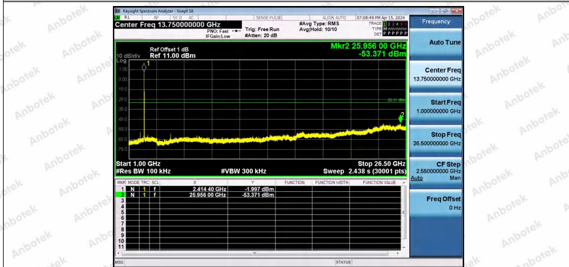
11AX20SISO-Ant1-2412-106Tone-RU54-1000~26500-PASS
