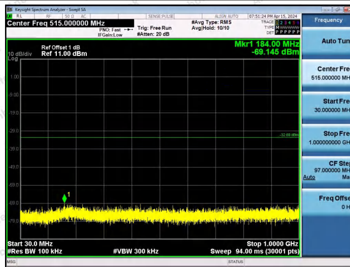
11AX20SISO-Ant1-2462-106Tone-RU53-30~1000-PASS
