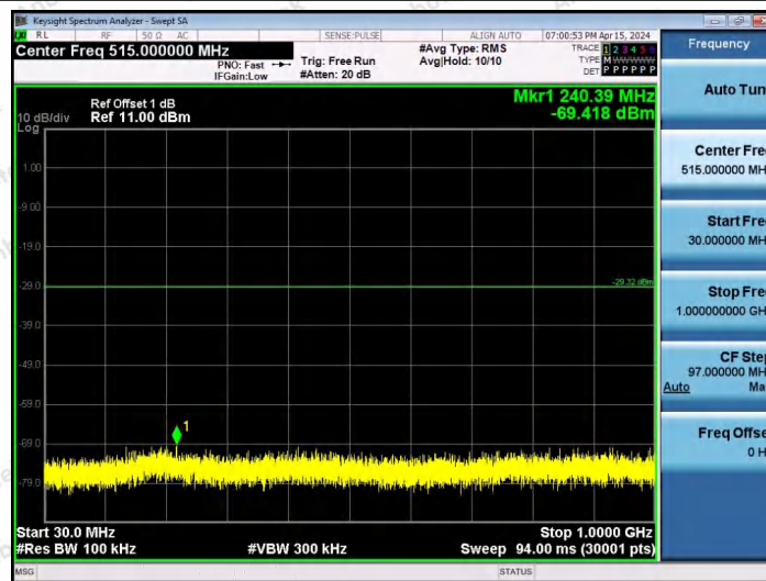
11AX20SISO-Ant1-2412-52Tone-RU39-30~1000-PASS
