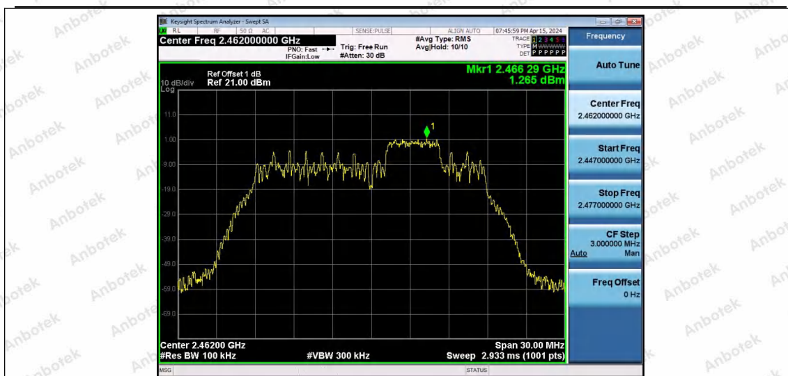
11AX20ISO-Ant1-2462-52Tone-RU39-0~Reference-PASS
