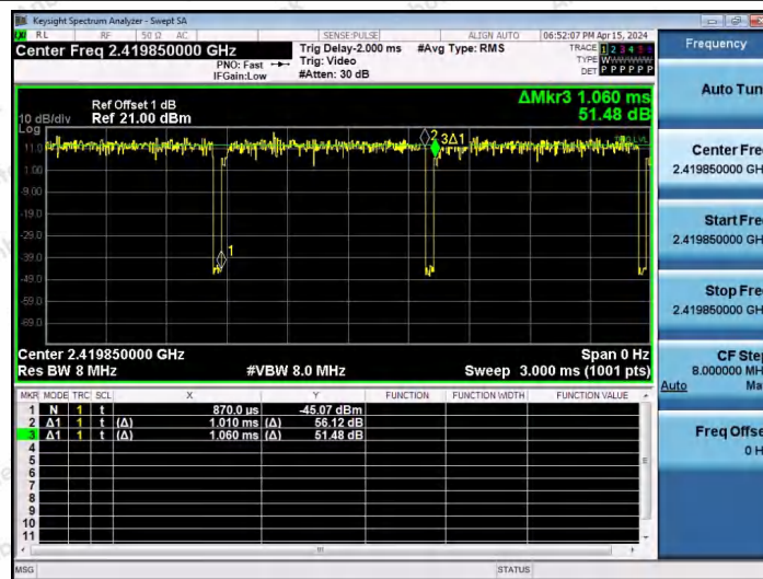
NTNV-11AX20SISO-Ant1-2412-26Tone-RU8
