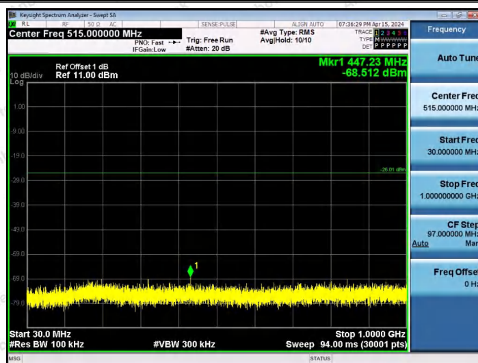
11AX20SISO-Ant1-2462-26Tone-RU4-30~1000-PASS
