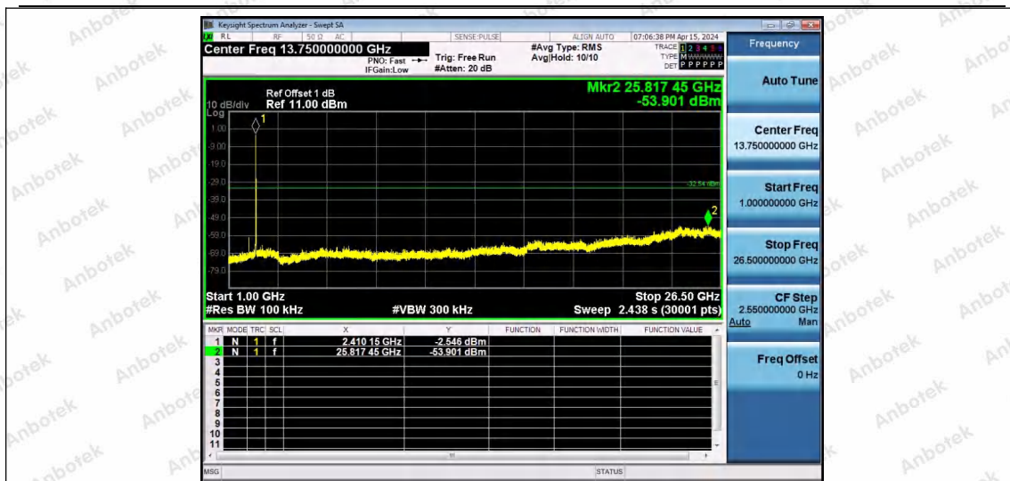
11AX20SISO-Ant1-2412-106Tone-RU53-1000~26500-PASS
