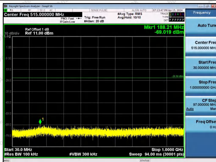
11AX20SISO-Ant1-2437-26Tone-RU4-30~1000-PASS
