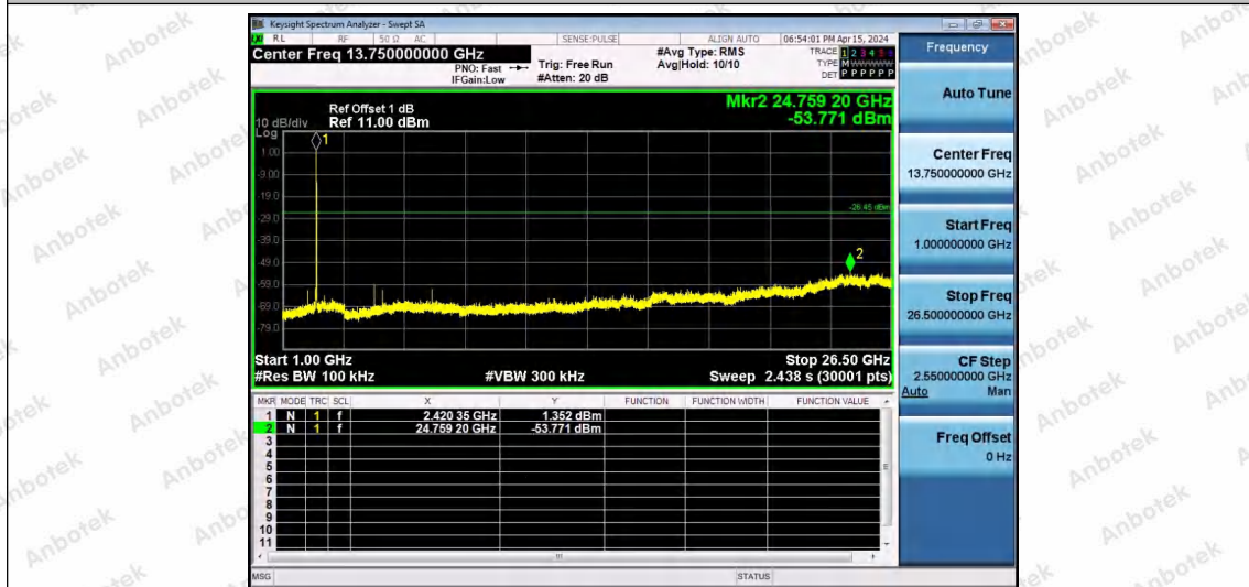
11AX20SISO-Ant1-2412-26Tone-RU8-1000~26500-PASS
