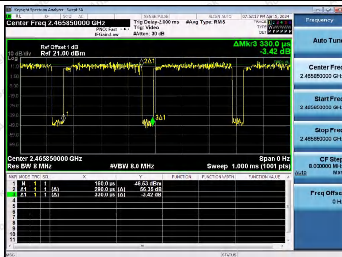
NTNV-11AX20SISO-Ant1-2462-106Tone-RU54
