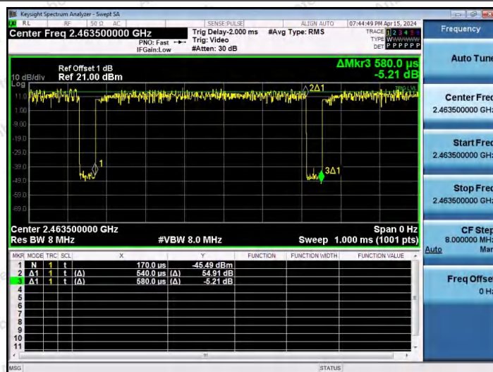
NTNV-11AX20SISO-Ant1-2462-52Tone-RU39
