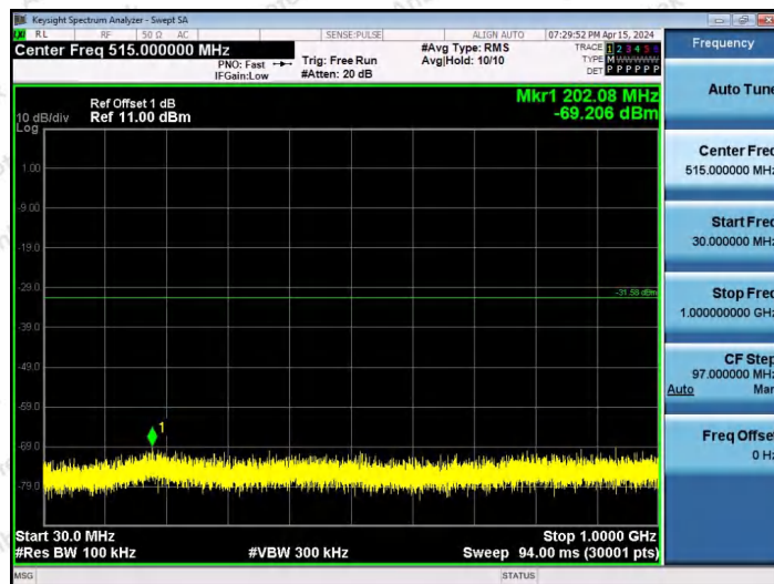
11AX20SISO-Ant1-2437-106Tone-RU53-30~1000-PASS
