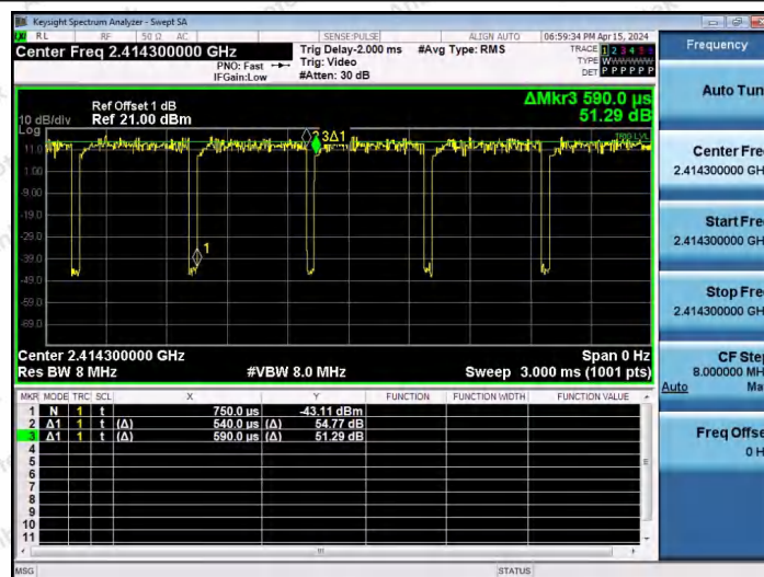
NTNV-11AX20SISO-Ant1-2412-52Tone-RU37
