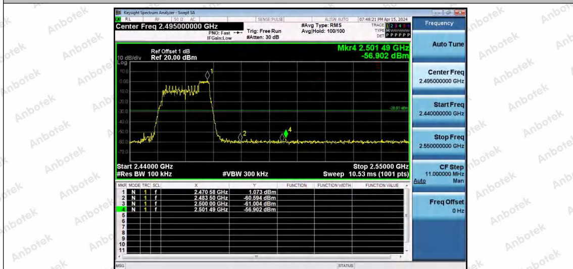
11AX20SISO-Ant1-2462-52Tone-RU40-PASS
