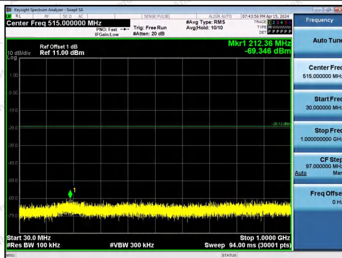
11AX20SISO-Ant1-2462-26Tone-RU8-30~1000-PASS
