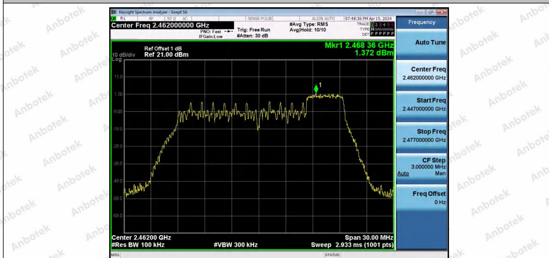
11AX20ISO-Ant1-2462-52Tone-RU40-0~Reference-PASS
