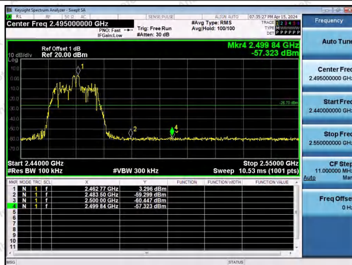
11AX20SISO-Ant1-2462-26Tone-RU0-PASS
