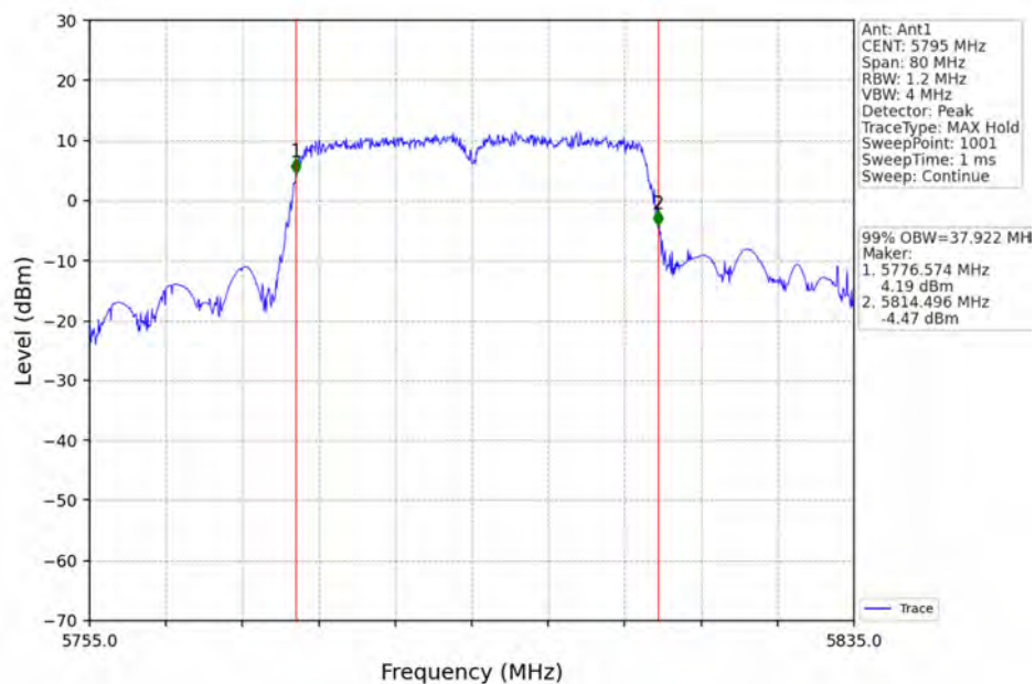
802.11ac(VHT40)_HCH_5795MHz_Ant1_NTNV
