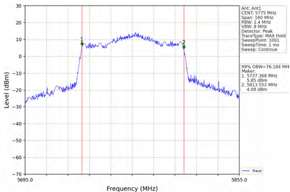
802.11ac(VHT80)_MCH_5775MHz_Ant1_NTNV
