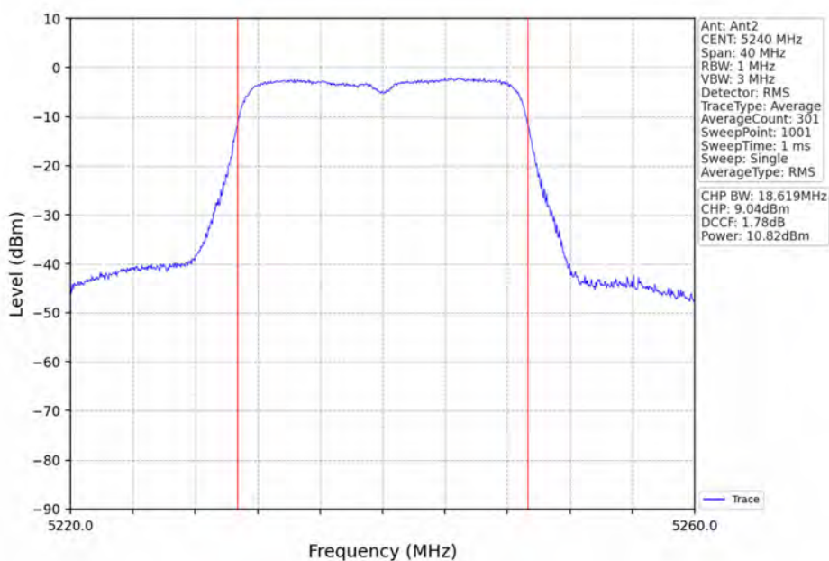
802.11n(HT20)_HCH_5240MHz_Ant2_NTNV
