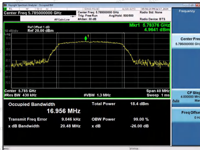
11A-Ant1-5785
