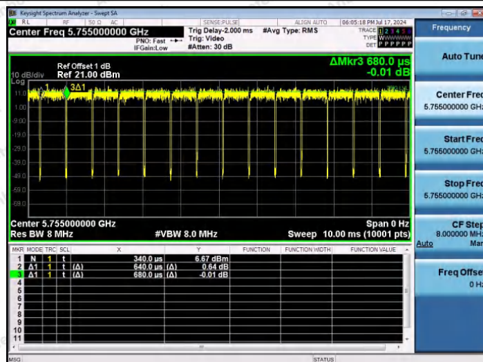
NTNV-11N40SISO-Ant1-5755
