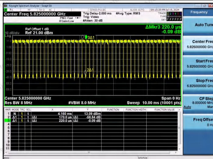
NTNV-11AX20SISO-Ant1-5825
