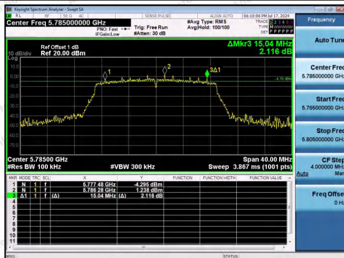
11AC20SISO-Ant1-5785-PASS
