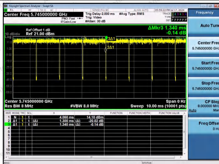
NTNV-11N20SISO-Ant1-5745
