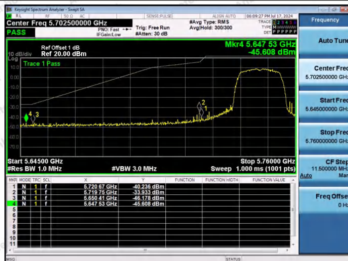
11AC20SISO-Ant1-5745-PASS
