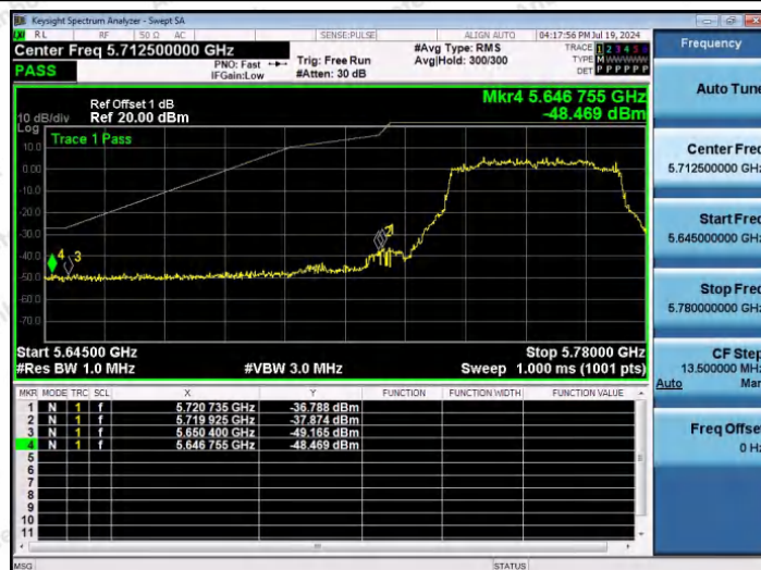
11AX40SISO-Ant1-5755-PASS
