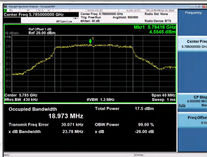
11AX20SISO-Ant1-5785
