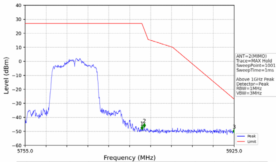
802.11ac(VHT40)_HCH_5795MHz_Ant2_NTNV
