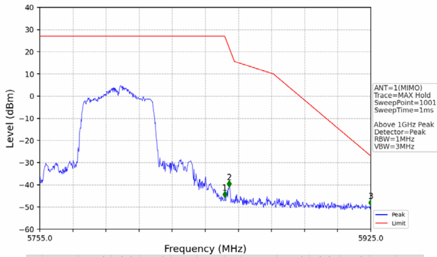
802.11ac(VHT40)_HCH_5795MHz_Ant1_NTNV
