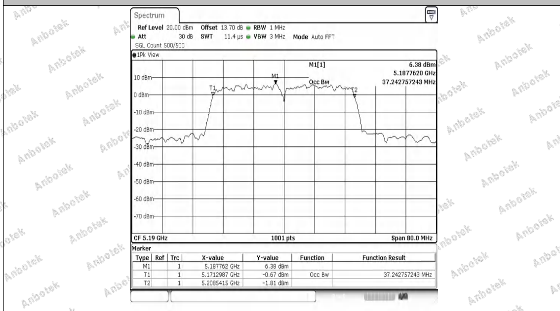
11AC40MIMO-Ant2-5190
