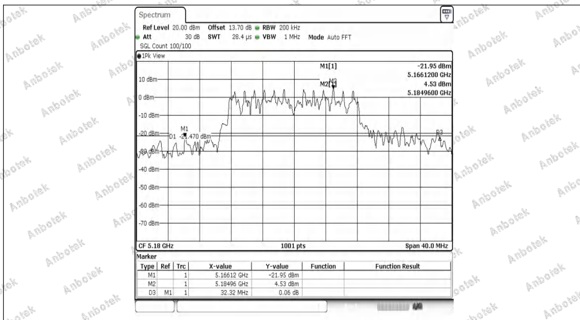
11AC20MIMO-Ant1-5180
