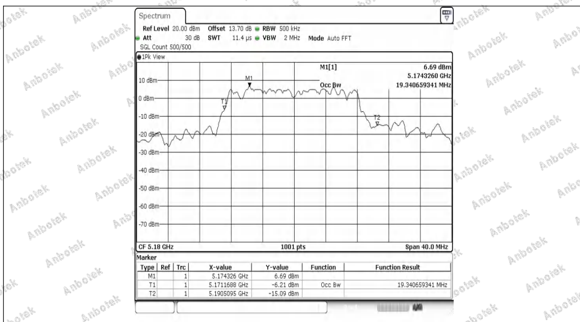
11AC20MIMO-Ant1-5180
