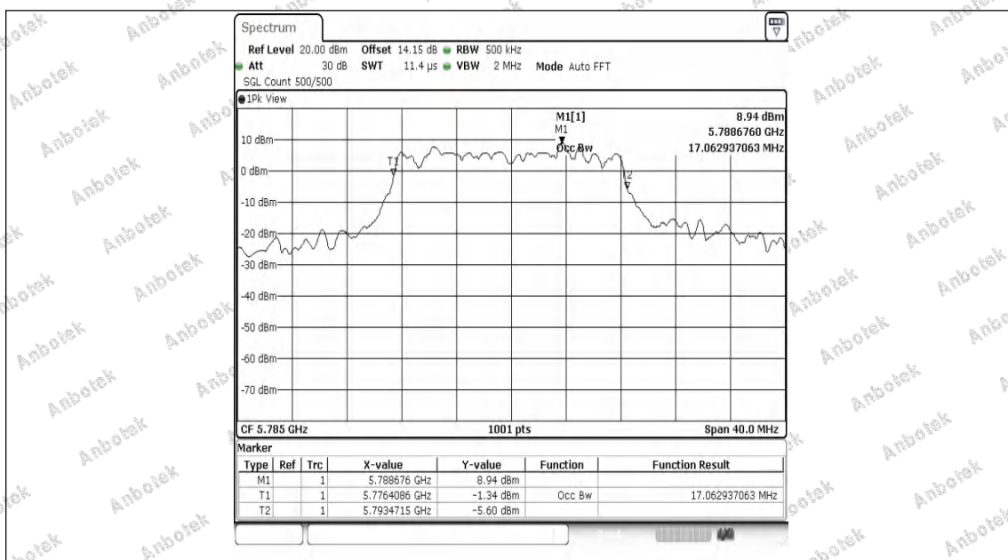
11AC20MIMO-Ant1-5785
