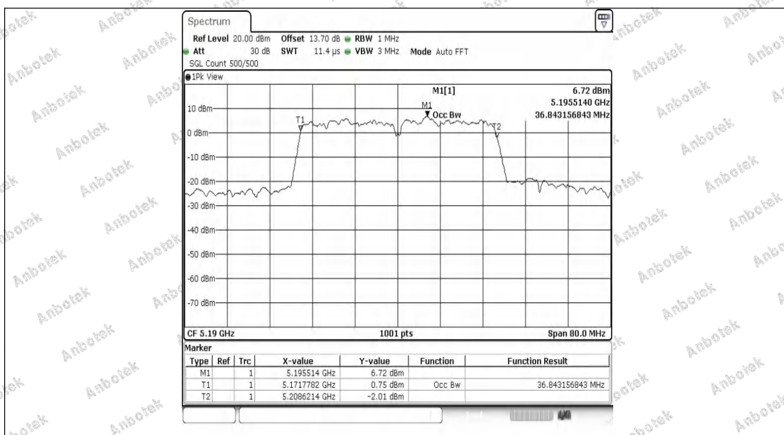
11AC40MIMO-Ant1-5190
