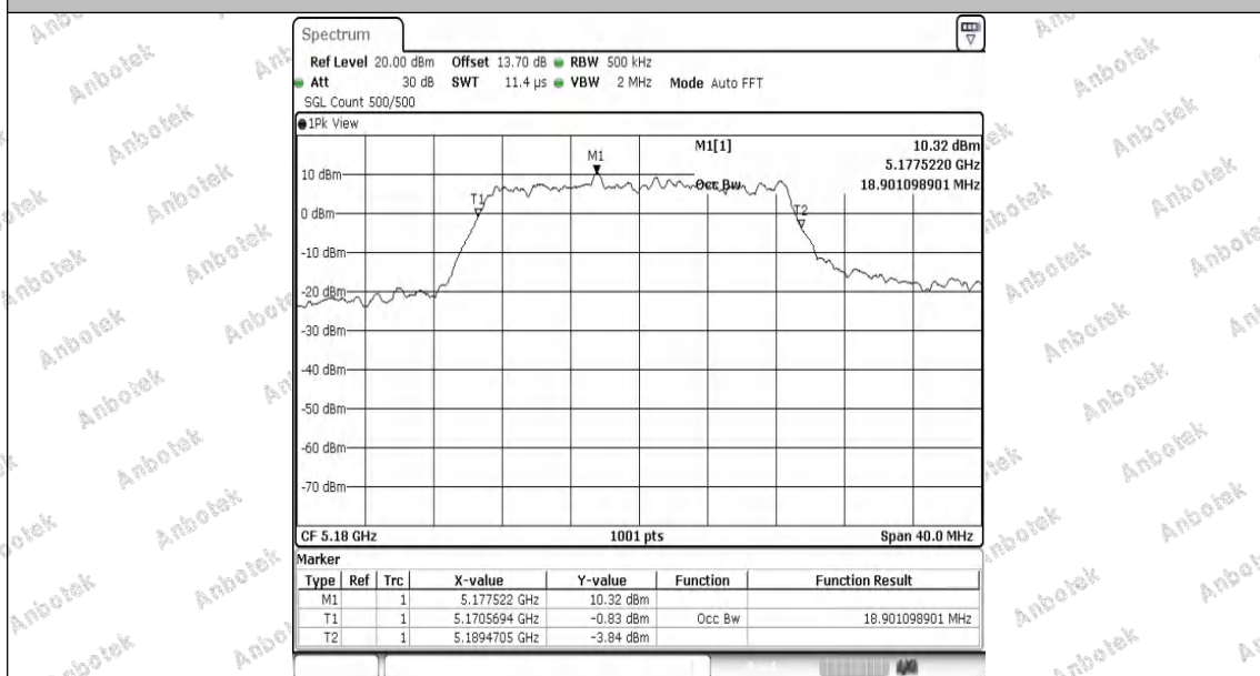
11AC20MIMO-Ant1-5180
