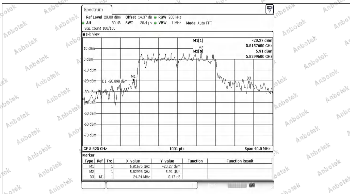
11AC20MIMO-Ant1-5825
