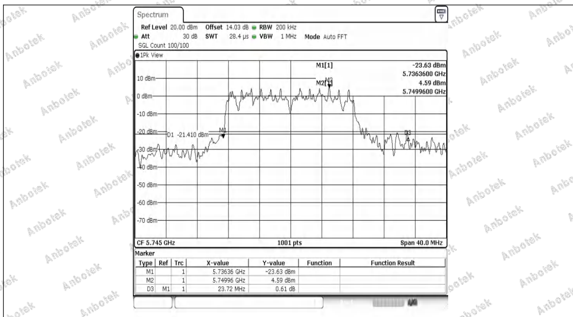
11AC20MIMO-Ant1-5745
