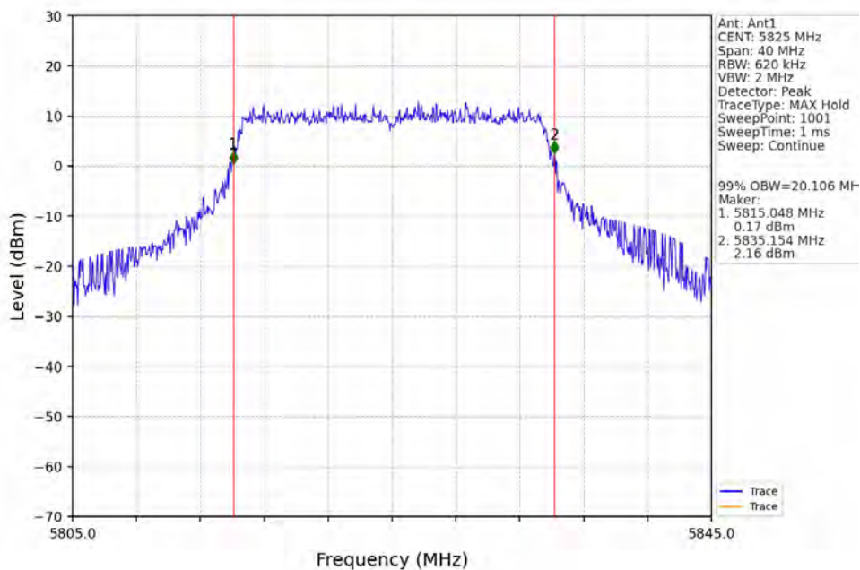
802.11ax(HEW20)_HCH_5825MHz_SU / _Ant1_NTNV
