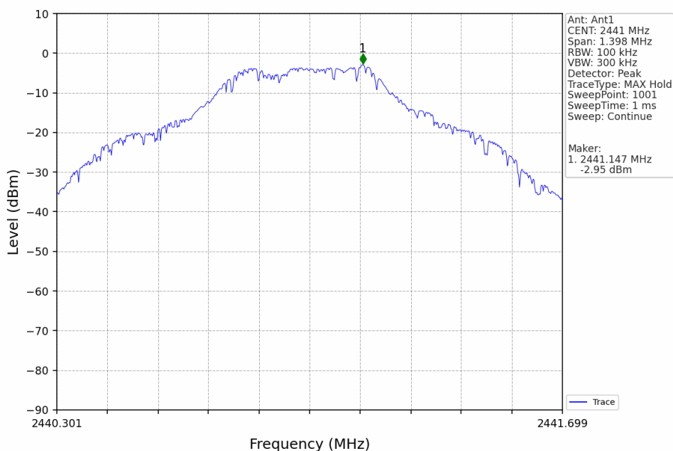
GFSK_DH5_MCH_2441MHz_Ant1_NTN
