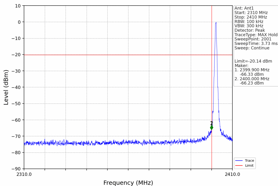
GFSK_DH5_LCH_2402MHz_Ant1_NTNV
