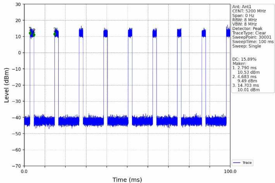
802.11n(HT20)_MCH_5200MHz_Ant1_NTNV
