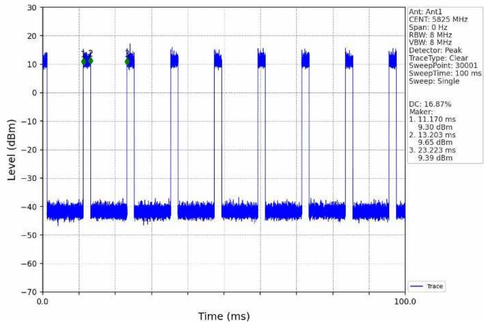
802.11a_HCH_5825MHz_Ant1_NTNV
