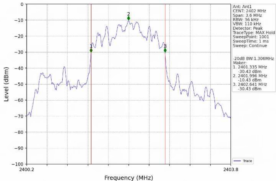
Pi/4DQPSK_2DH5_LCH_2402MHz_Ant1_NTNV
