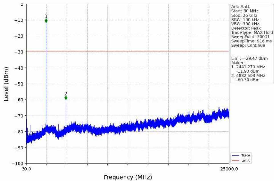
Pi/4DQPSK_2DH5_MCH_2441MHz_Ant1_NTNV
