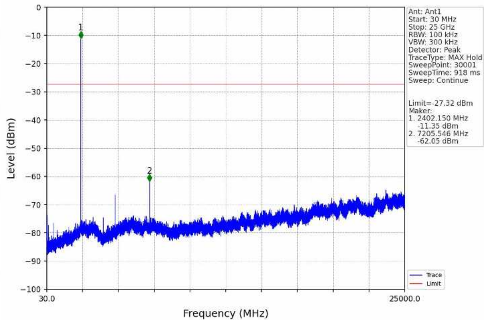
8DPSK_3DH5_LCH_2402MHz_Ant1_NTNV
