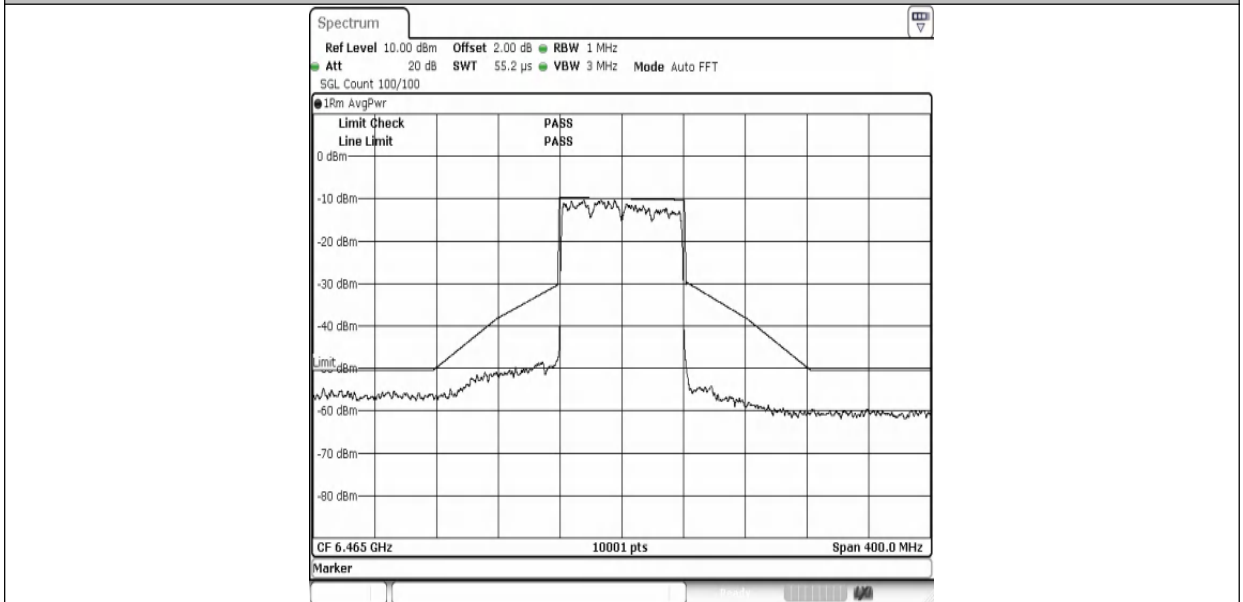
NTNV-11AX80MIMO-Ant1-6465-PASS
