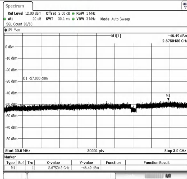
11AX80MIMO-Ant1-6145-30~3000-PASS
