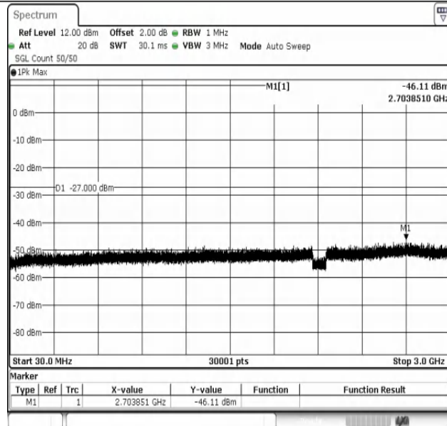
11AX80MIMO-Ant1-6385-30~3000-PASS
