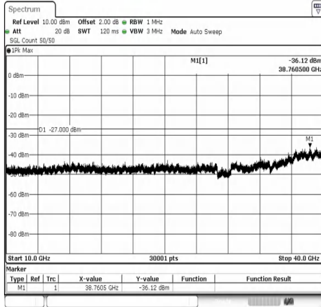
11AX80MIMO-Ant1-6385-10000~40000-PASS
