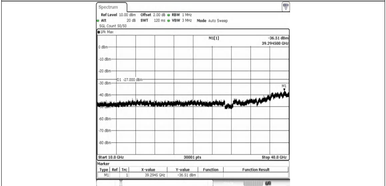
11AX80MIMO-Ant2-6145-10000~40000-PASS
