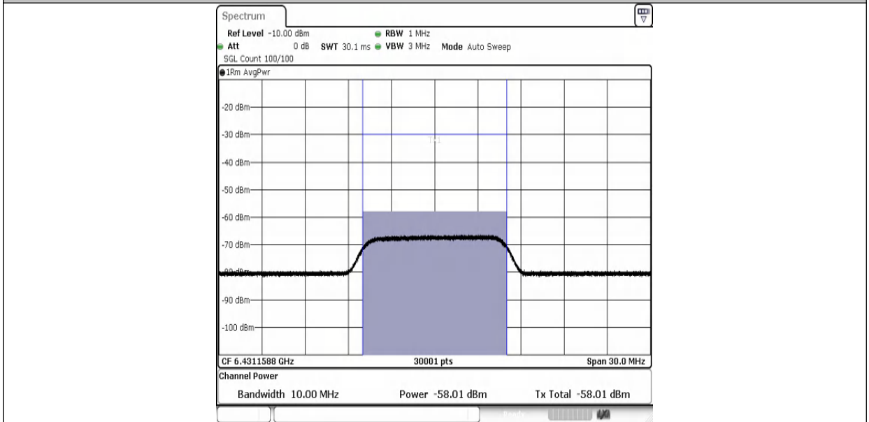
11AX80MIMO-Ant1-6465-6431.1588-PASS
