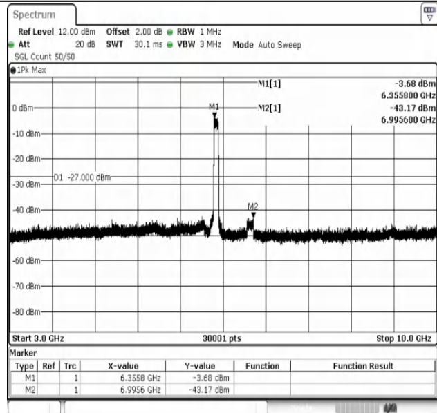
11AX80MIMO-Ant1-6385-3000~10000-PASS
