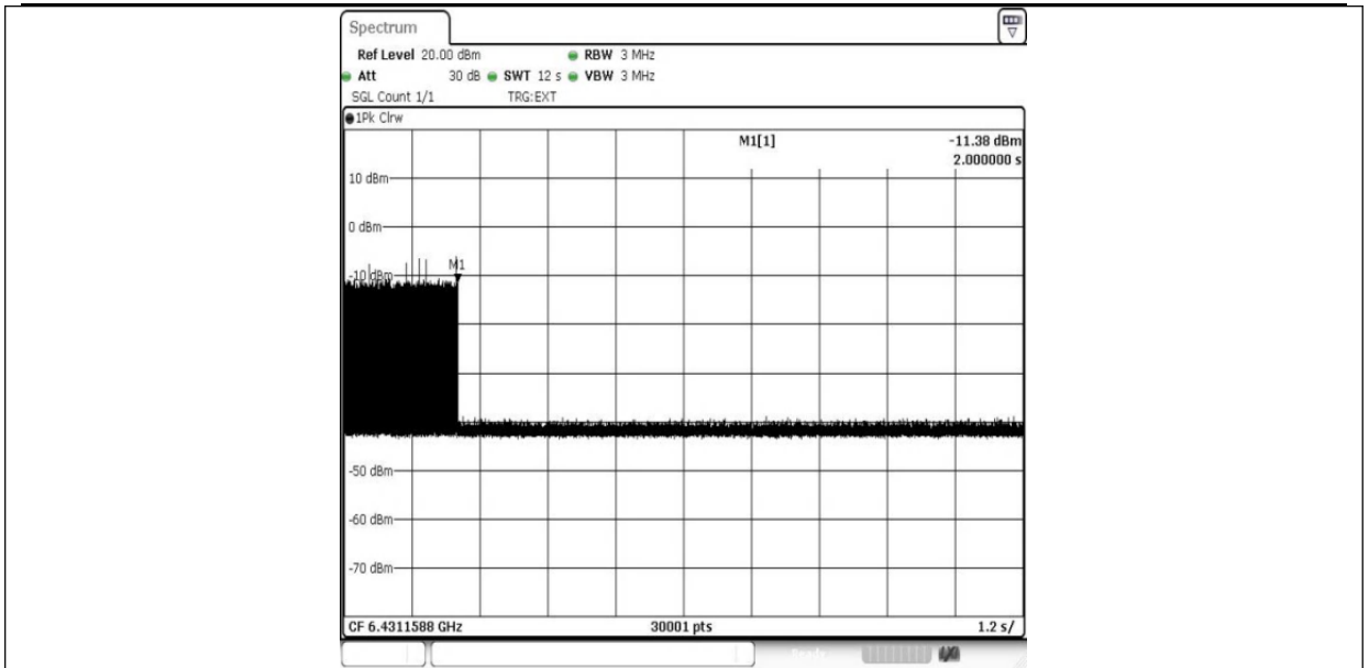
11AX80MIMO-Ant1-6465-6431.1588-PASS
