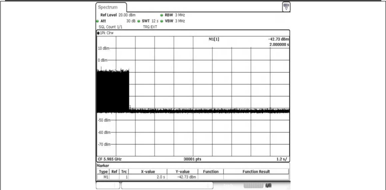
11AX80MIMO-Ant1-5985-5985-PASS
