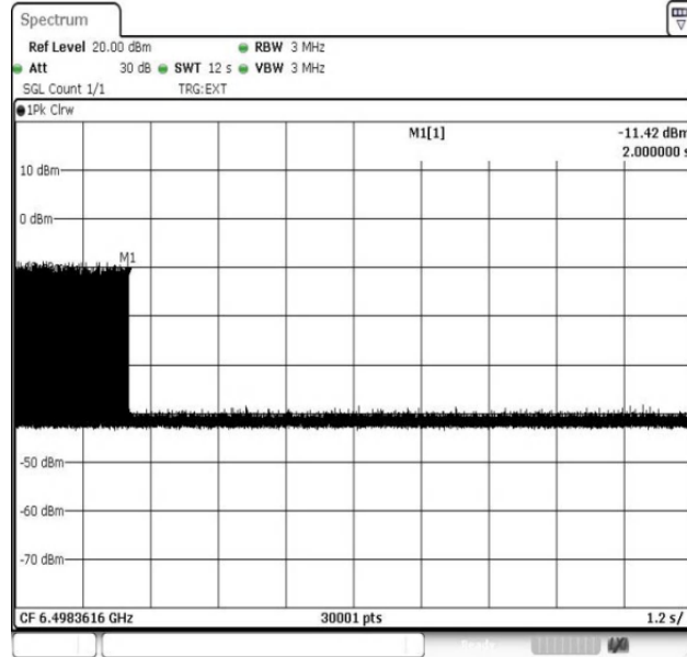
11AX80MIMO-Ant1-6465-6498.3616-PASS
