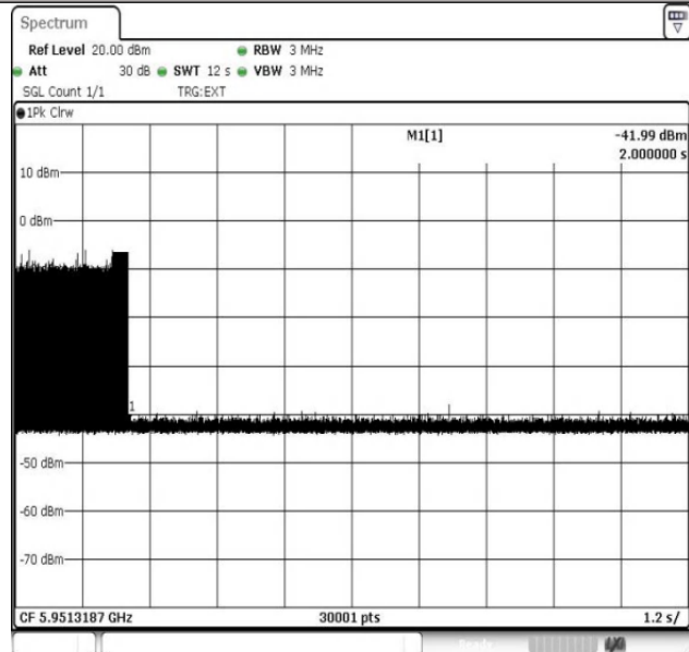
11AX80MIMO-Ant1-5985-5951.3187-PASS
