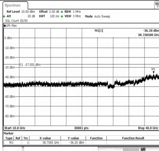
11AX80MIMO-Ant1-6465-10000~40000-PASS
