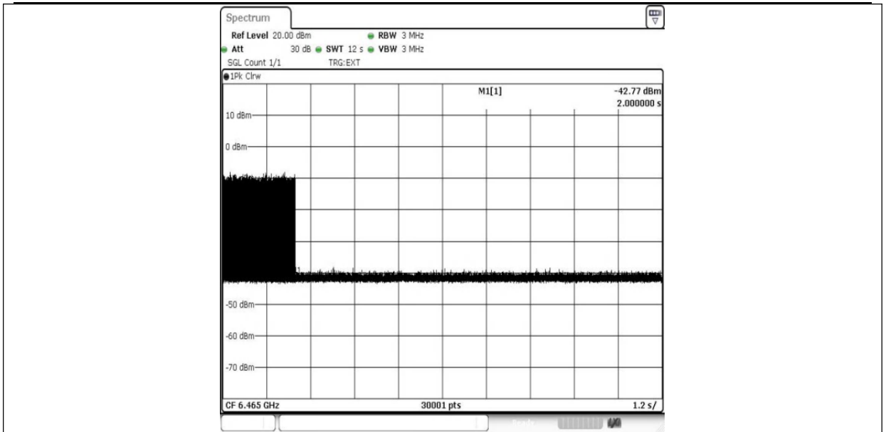
11AX80MIMO-Ant1-6465-6465-PASS
