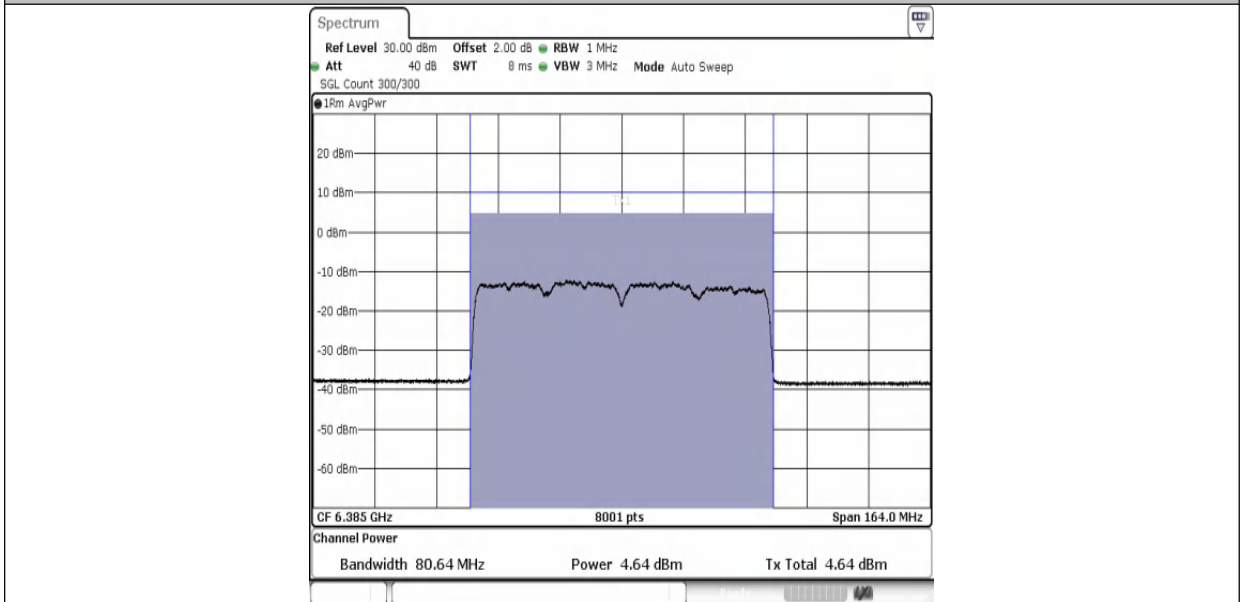
11AX80MIMO-Ant1-6385-PASS
