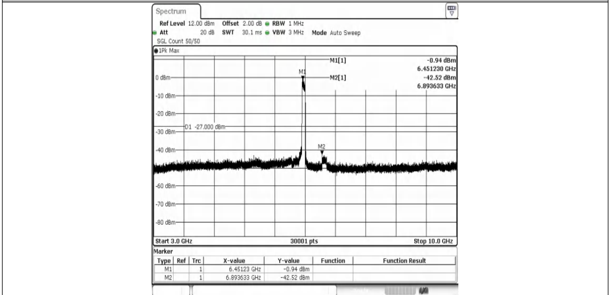
11AX80MIMO-Ant1-6465-3000~10000-PASS
