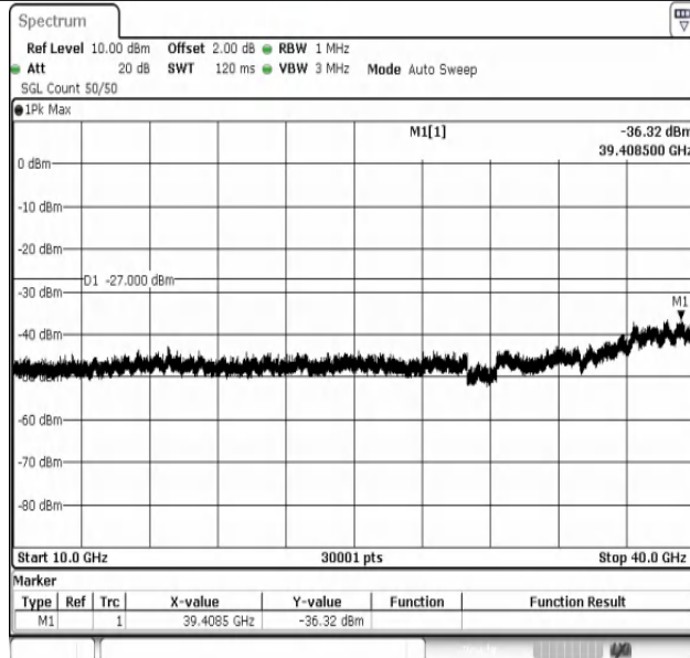
11AX80MIMO-Ant2-6385-10000~40000-PASS
