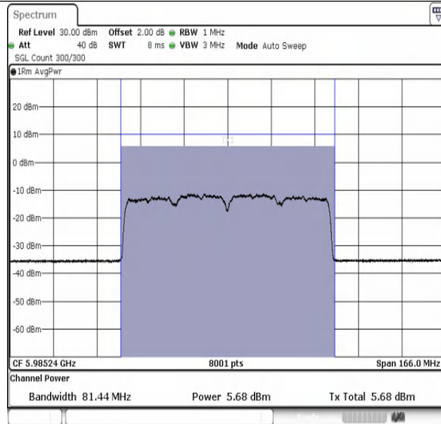
11AX80MIMO-Ant1-5985-PASS
