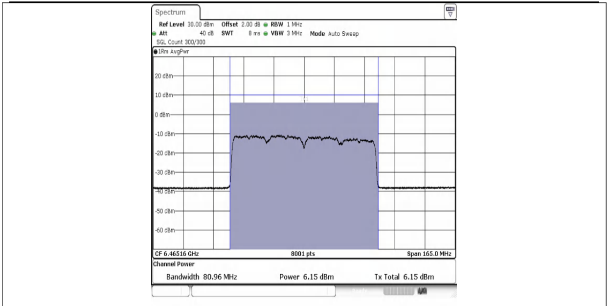
11AX80MIMO-Ant1-6465-PASS
