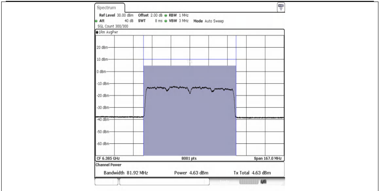
11AX80MIMO-Ant1-6385-PASS
