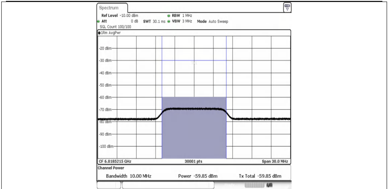
11AX80MIMO-Ant1-5985-6018.5215-PASS
