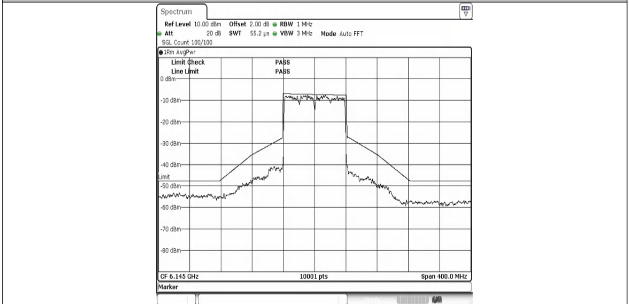
NTNV-11AX80MIMO-Ant1-6145-PASS
