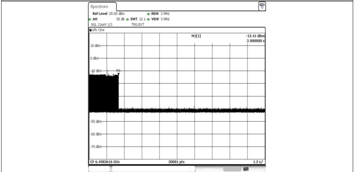
11AX80MIMO-Ant1-6465-6498.3616-PASS
