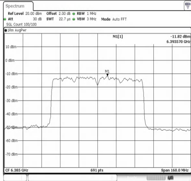
11AX80MIMO-Ant1-6385-PASS
