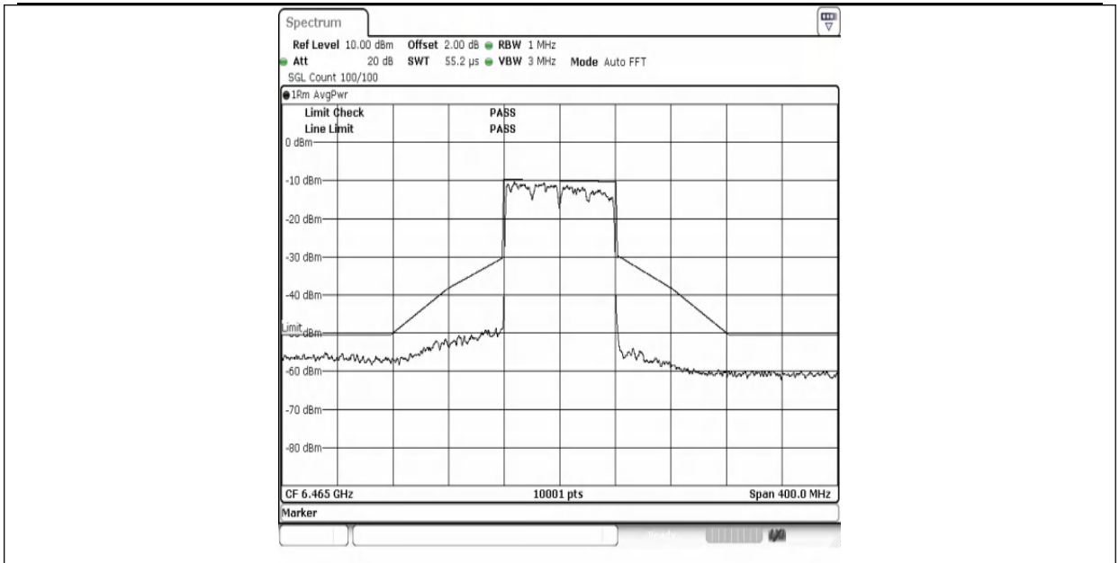
NTNV-11AX80MIMO-Ant1-6465-PASS
