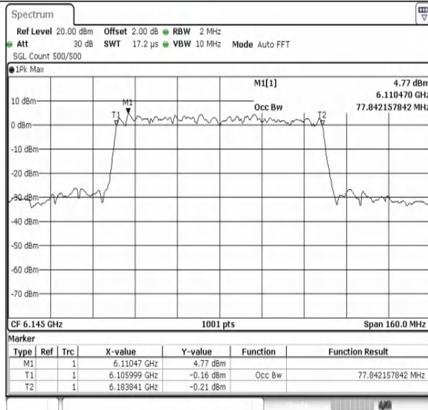
11AX80MIMO-Ant1-6145-PASS
