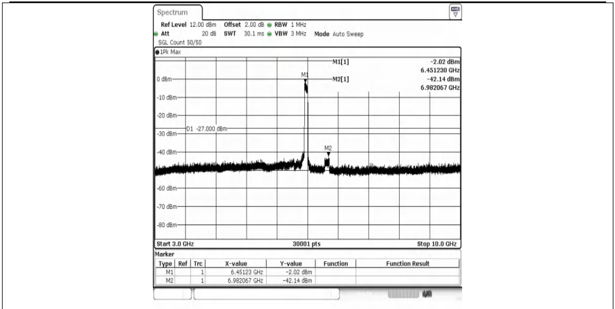
11AX80MIMO-Ant1-6465-3000~10000-PASS
