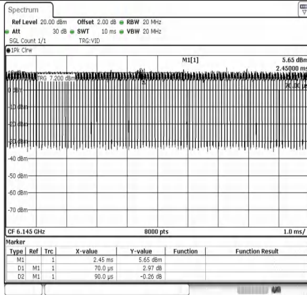
NTNV-11AX80MIMO-Ant1-6145
