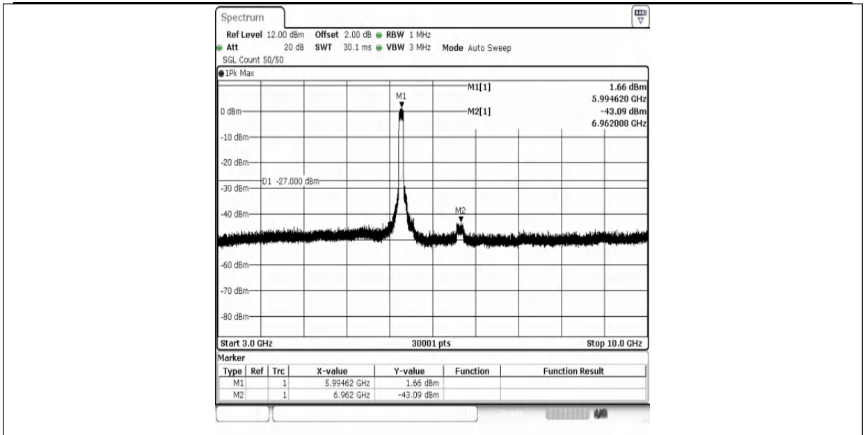
11AX80MIMO-Ant1-5985-3000~10000-PASS
