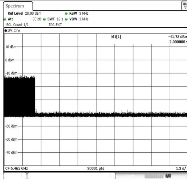
11AX80MIMO-Ant1-6465-6465-PASS
