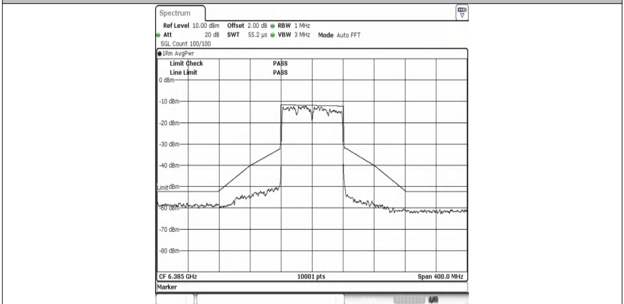
NTNV-11AX80MIMO-Ant1-6385-PASS
