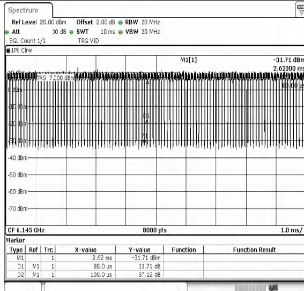
NTNV-11AX80MIMO-Ant2-6145
