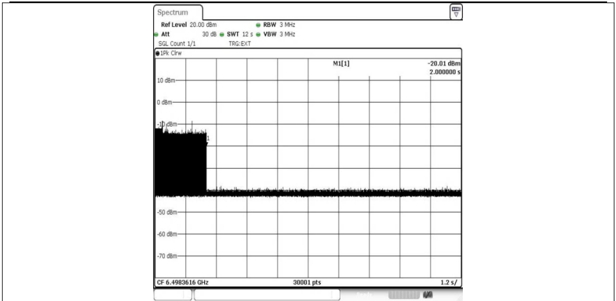
11AX80MIMO-Ant1-6465-6498.3616-PASS
