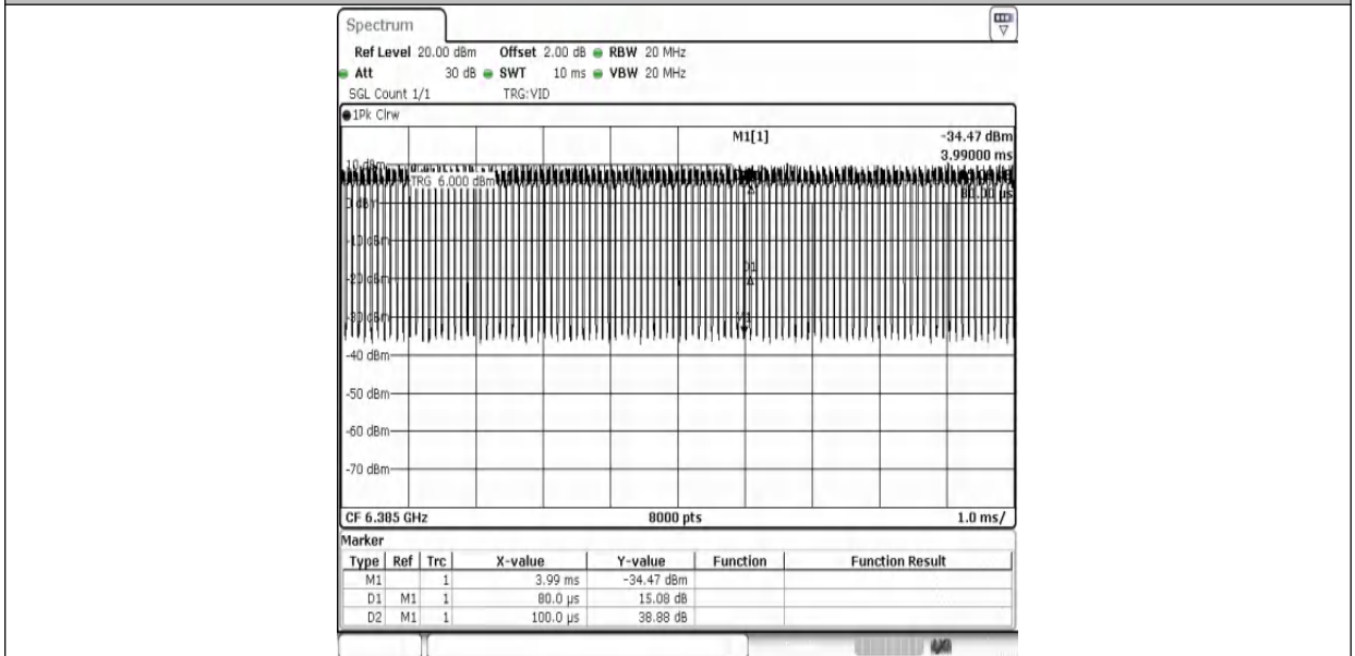
NTNV-11AX80MIMO-Ant2-6385
