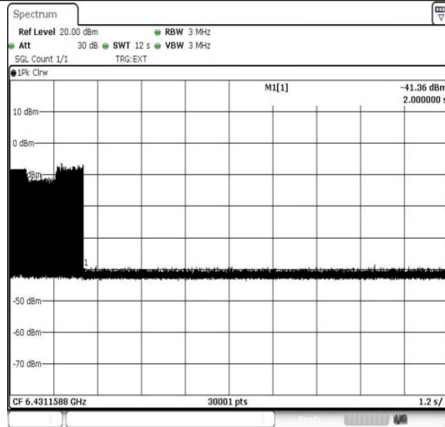
11AX80MIMO-Ant1-6465-6431.1588-PASS
