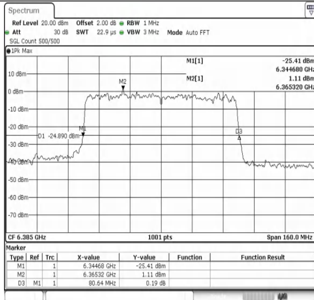
11AX80MIMO-Ant1-6385
