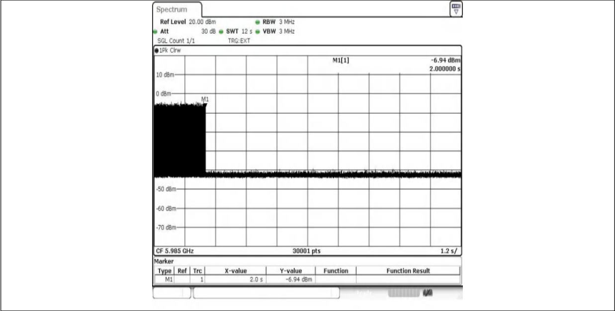
11AX80MIMO-Ant1-5985-5985-PASS
