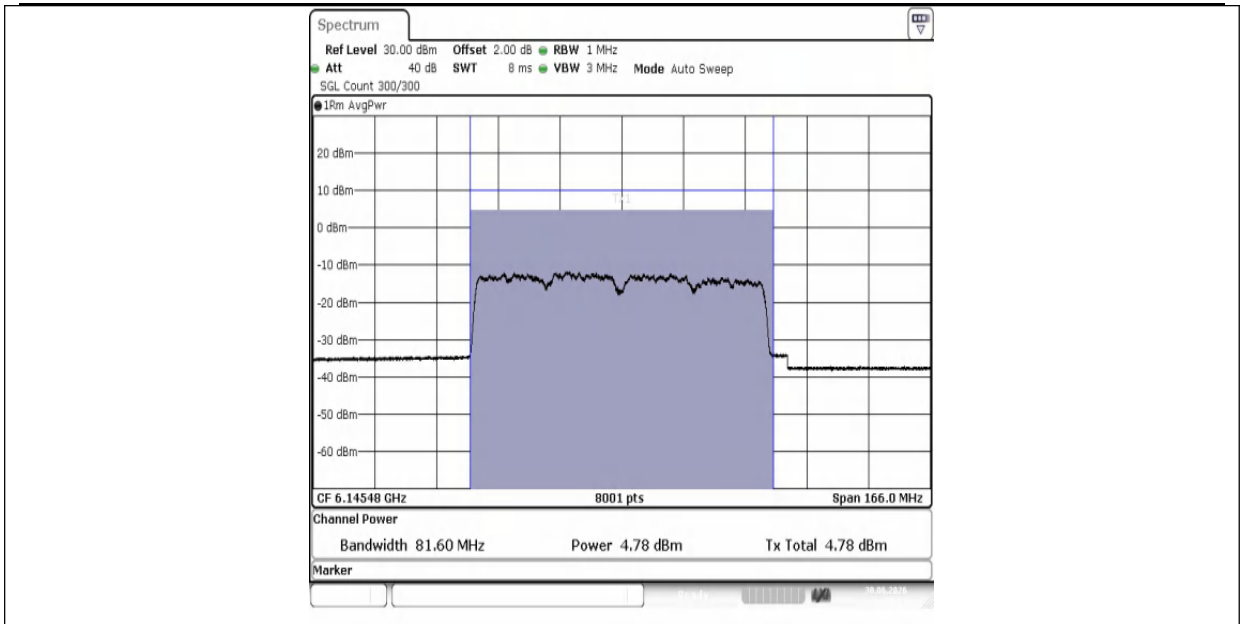
11AX80MIMO-Ant1-6145-PASS
