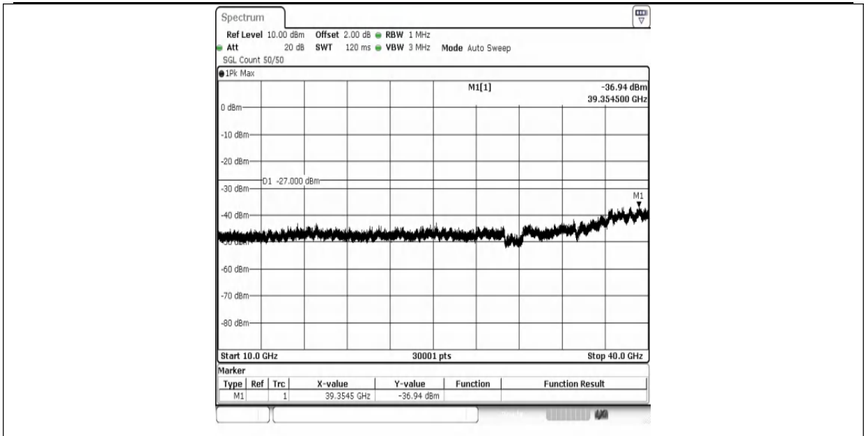
11AX80MIMO-Ant1-6145-10000~40000-PASS
