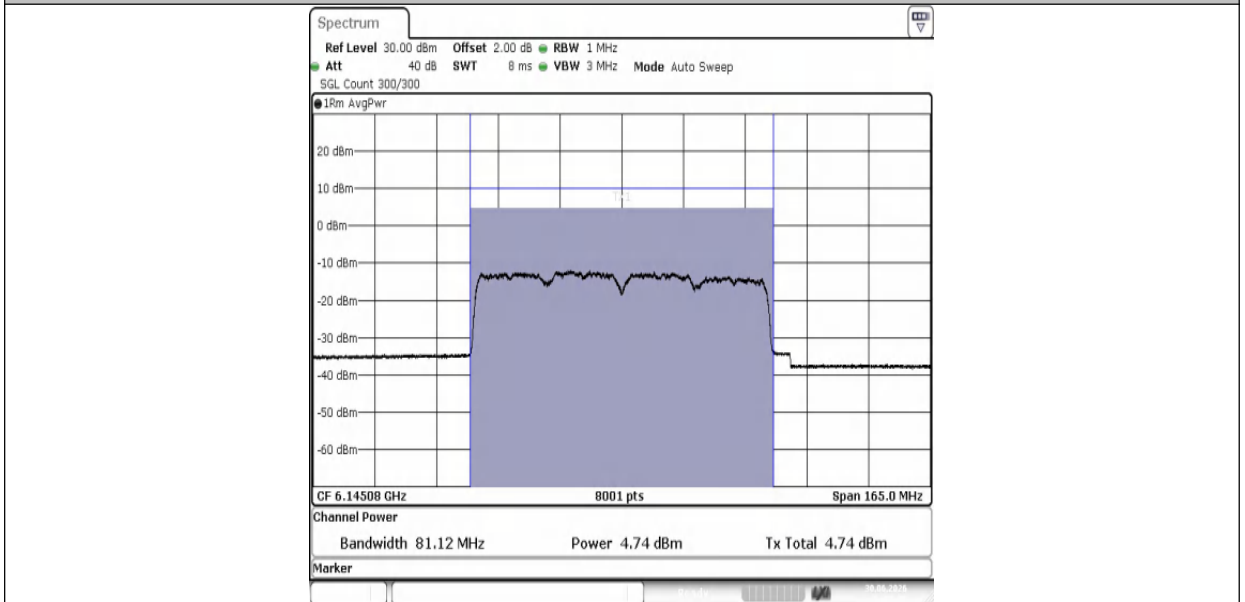
11AX80MIMO-Ant1-6145-PASS
