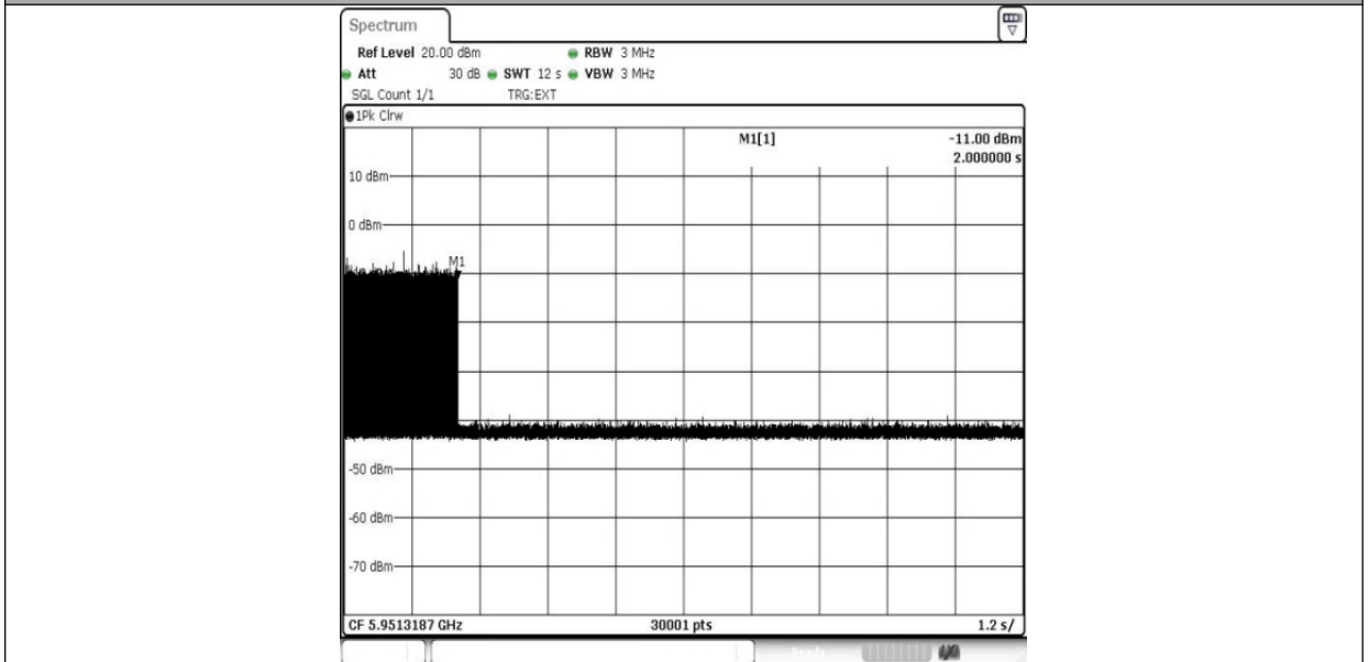
11AX80MIMO-Ant1-5985-5951.3187-PASS
