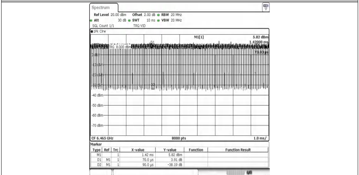
NTNV-11AX80MIMO-Ant1-6465
