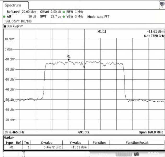
11AX80MIMO-Ant1-6465-PASS
