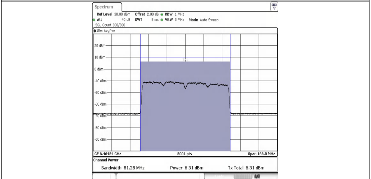
11AX80MIMO-Ant1-6465-PASS
