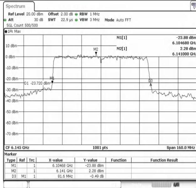
11AX80MIMO-Ant1-6145
