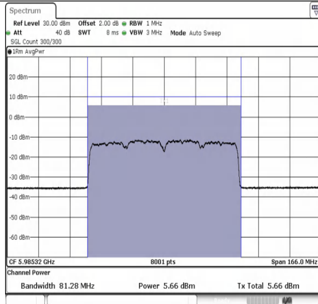
11AX80MIMO-Ant2-5985-PASS
