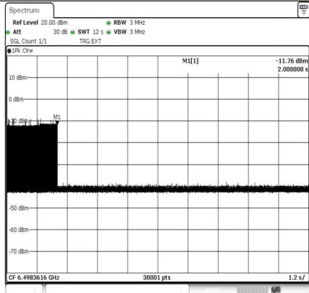
11AX80MIMO-Ant1-6465-6498.3616-PASS
