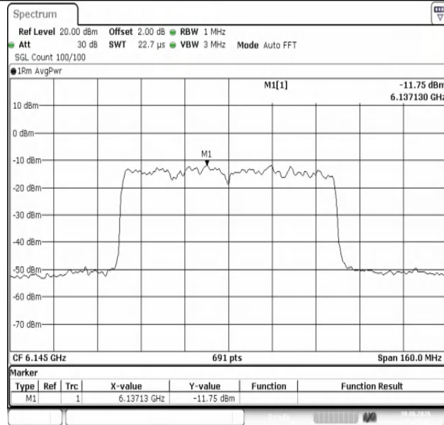
11AX80MIMO-Ant1-6145-PASS
