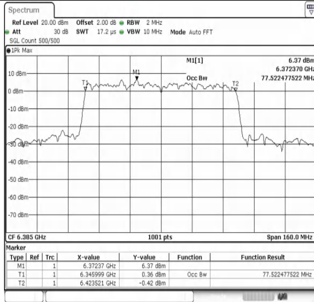
11AX80MIMO-Ant1-6385-PASS
