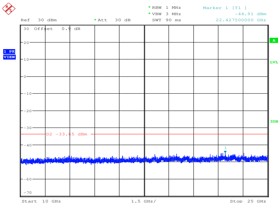
RF Conducted Spurious Emissions 11N40SISO 2437 Ant1
