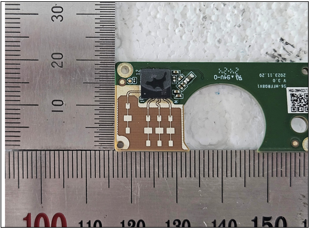
Antenna & Chipset
