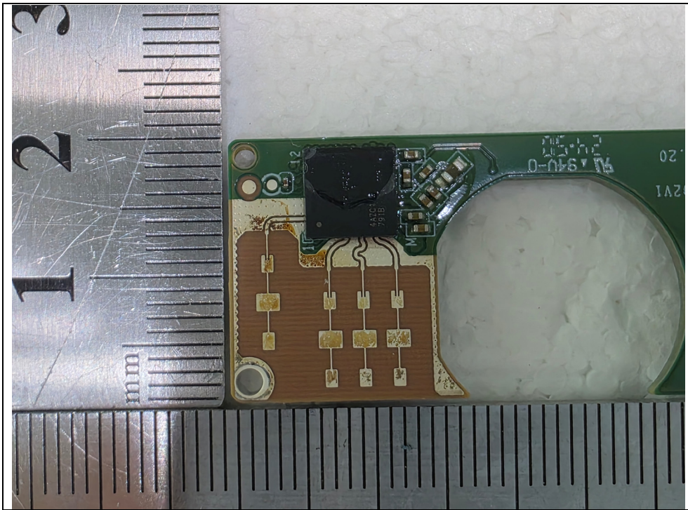
Antenna & Chipset
