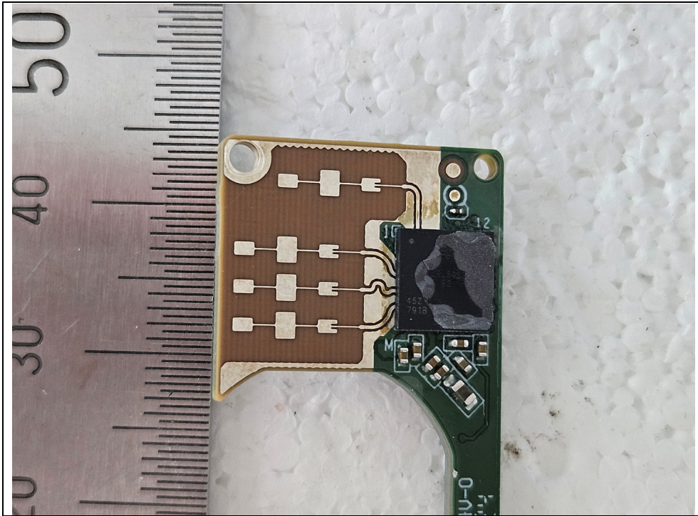
Antenna & Chipset
