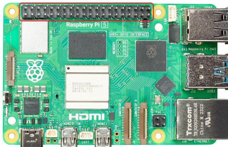
Figure 3 - 40 Pin GPIO Header J8
