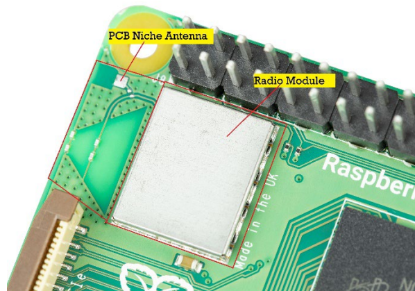
Figure 1 - Radio Circuitry
