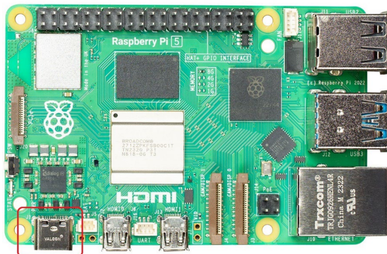
Figure 2 - USB-C Power Connector J1
