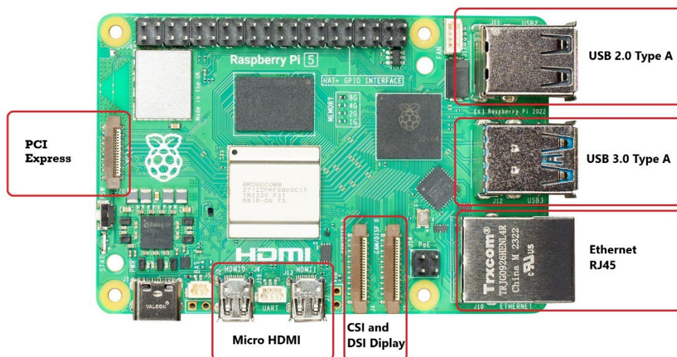
Figure 5 - Peripheral Connections
