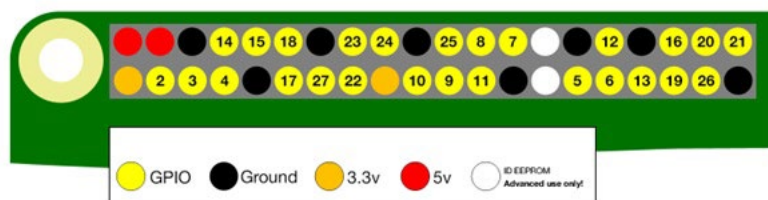
Figure 4 - 40 Pin GPIO Power Supply Example
