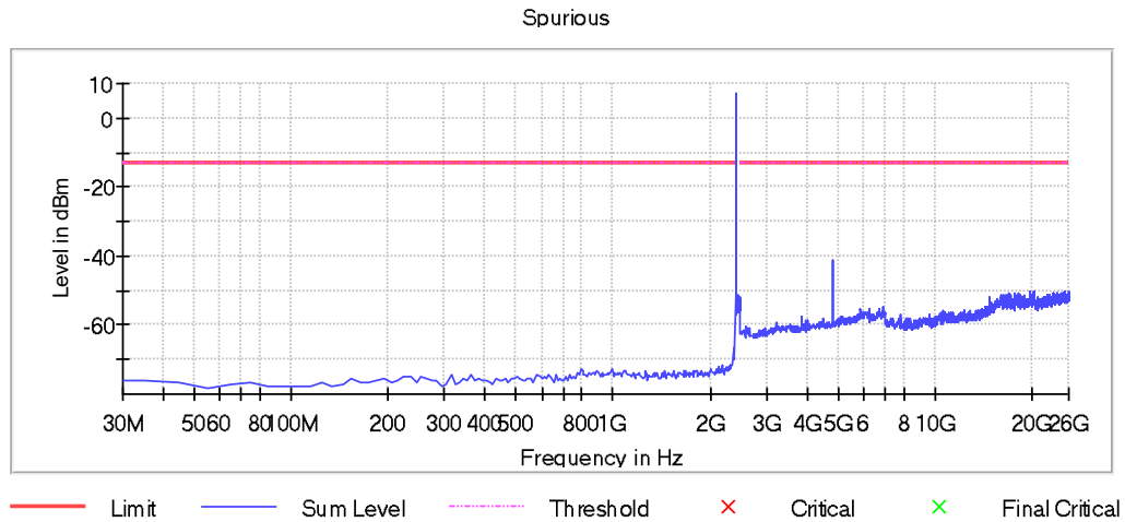
Plot 14: CSE, OP 1, low channel, 30 MHz – 26 GHz
