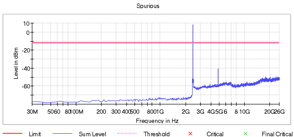
Plot 15: CSE, OP 1, mid channel, 30 MHz – 26 GHz
