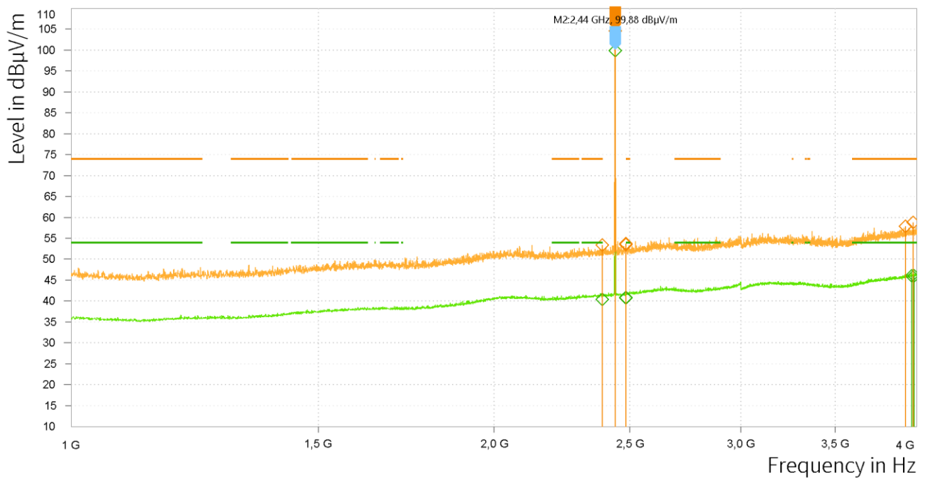
Plot 24: RSE 1 GHz – 4 GHz, OP 1, mid channel, horizontal / vertical polarisation
