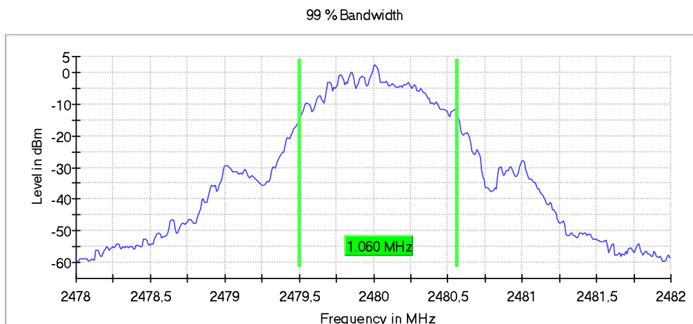
Plot 6: 99% Occupied Bandwidth, OP 1, high channel
