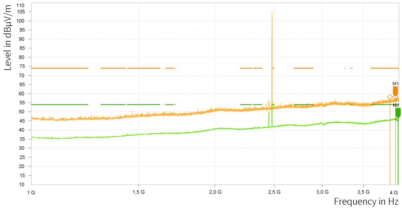
Plot 25: RSE 1 GHz – 4 GHz, OP 1, high channel, horizontal / vertical polarisation
