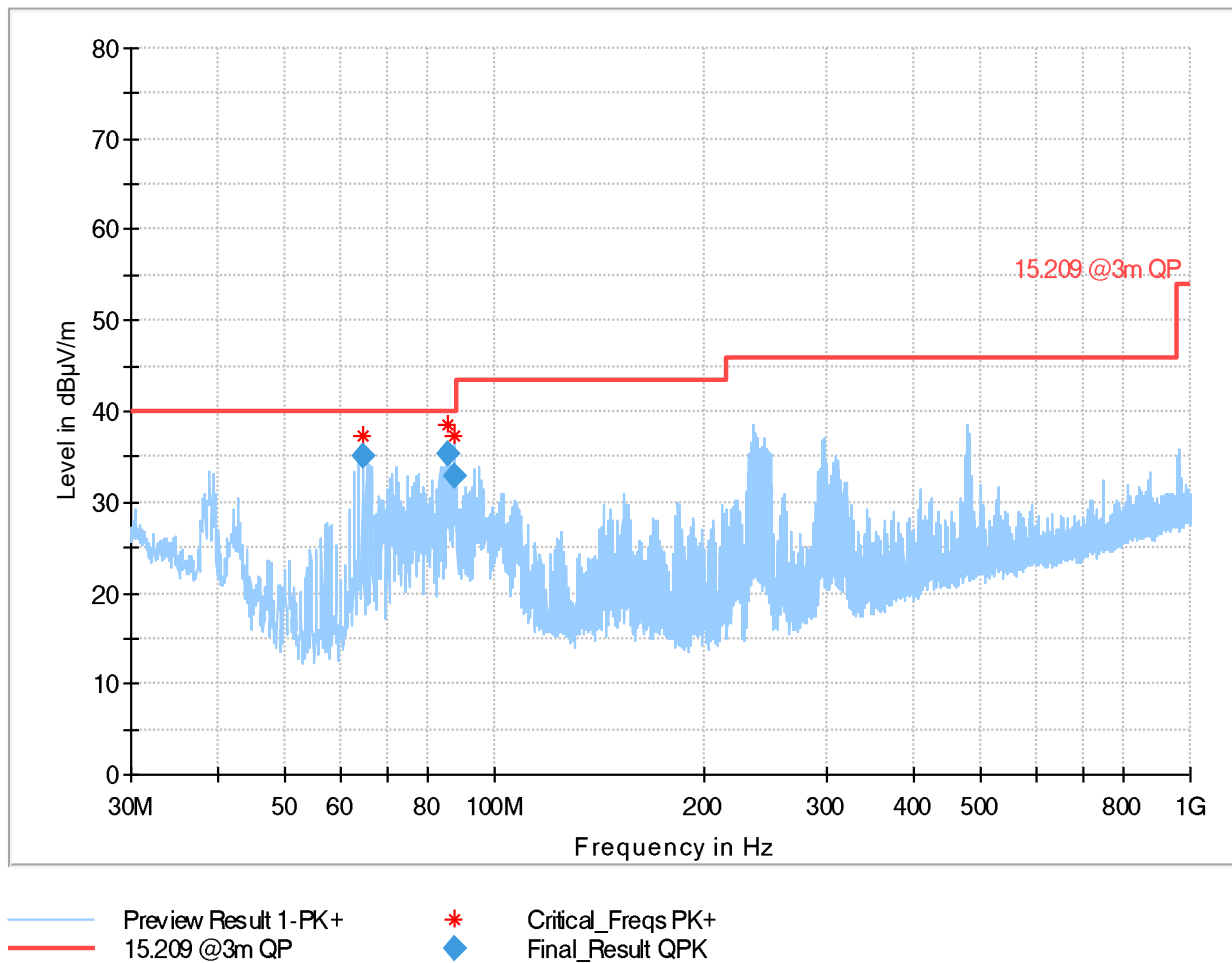
Plot 20: RSE 30 MHz – 1 GHz, OP 1, low channel, horizontal / vertical polarisation
