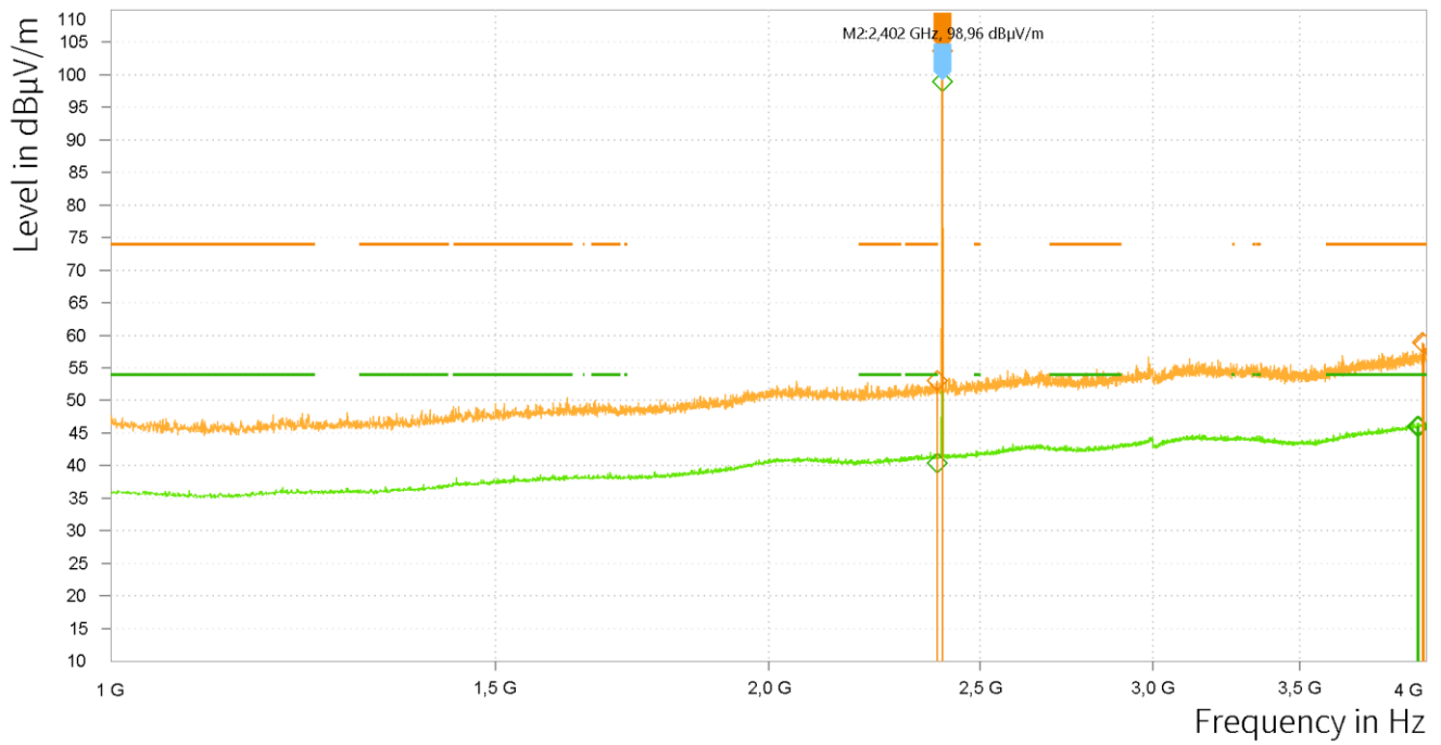
Plot 23: RSE 1 GHz – 4 GHz, OP 1, low channel, horizontal / vertical polarisation
