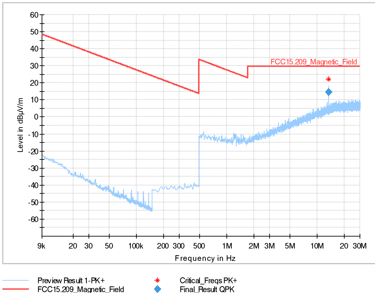
Plot 18: RSE 9 kHz – 30 MHz, OP 1, mid channel, loop antenna
