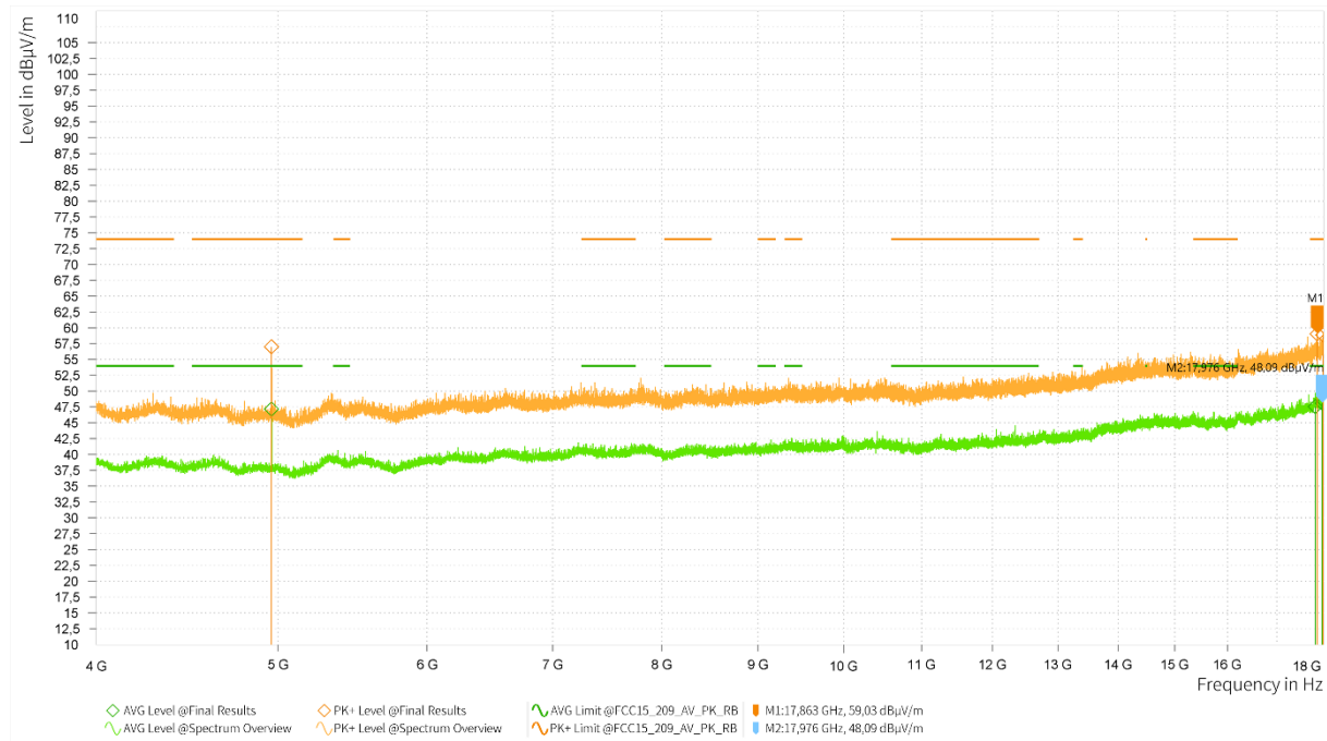
Plot 28: RSE 4 GHz – 18 GHz, OP 1, high channel, horizontal / vertical polarisation
