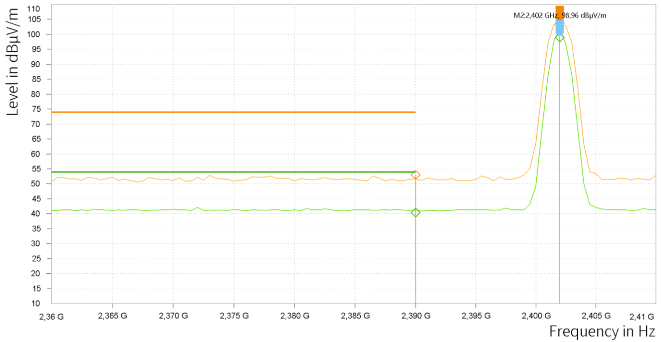
Plot 12: BEC, OP 1, low channel
