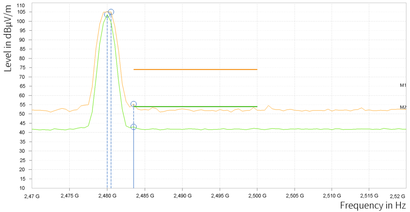
Plot 13: BEC, OP 1, high channel
