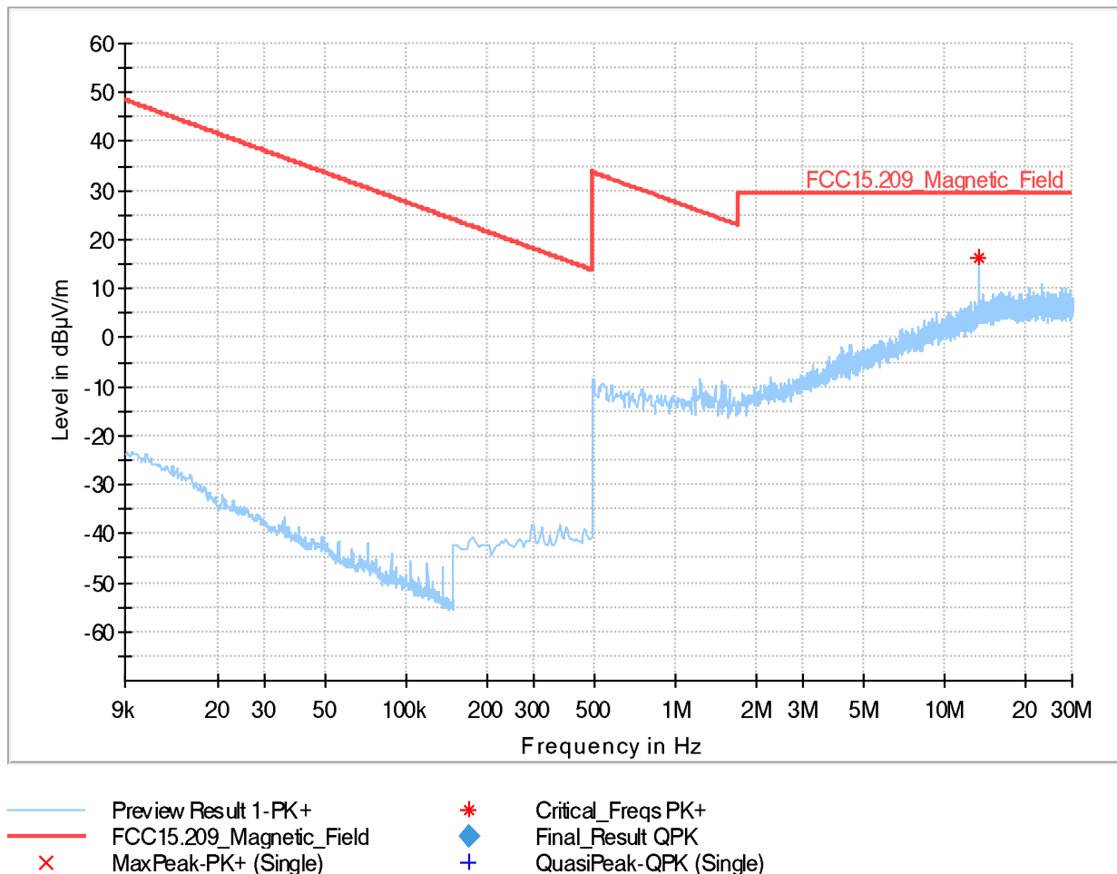
Plot 19: RSE 9 kHz – 30 MHz, OP 1, high channel, loop antenna
