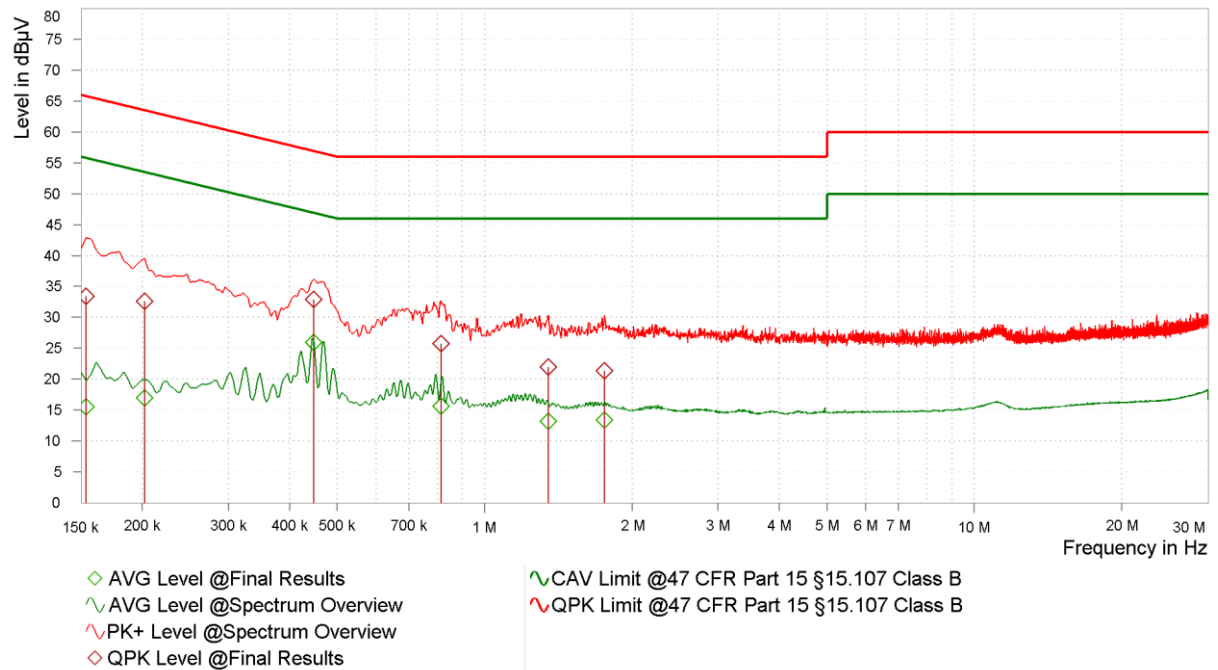
Plot no. 33: conducted emissions, neutral N
