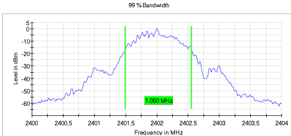
Plot 4: 99% Occupied Bandwidth, OP 1, low channel
