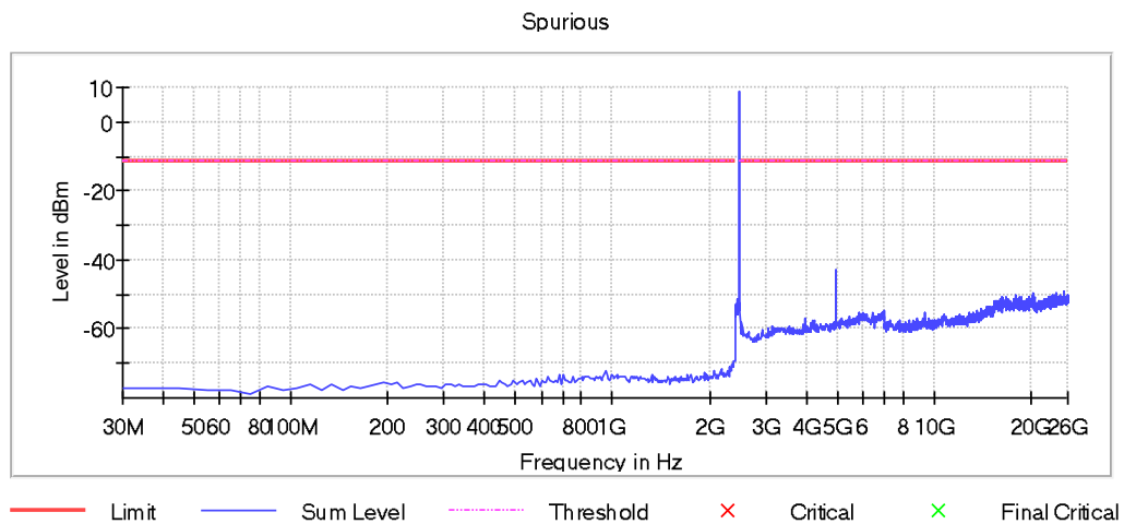
Plot 16: CSE, OP 1, high channel, 30 MHz – 26 GHza
