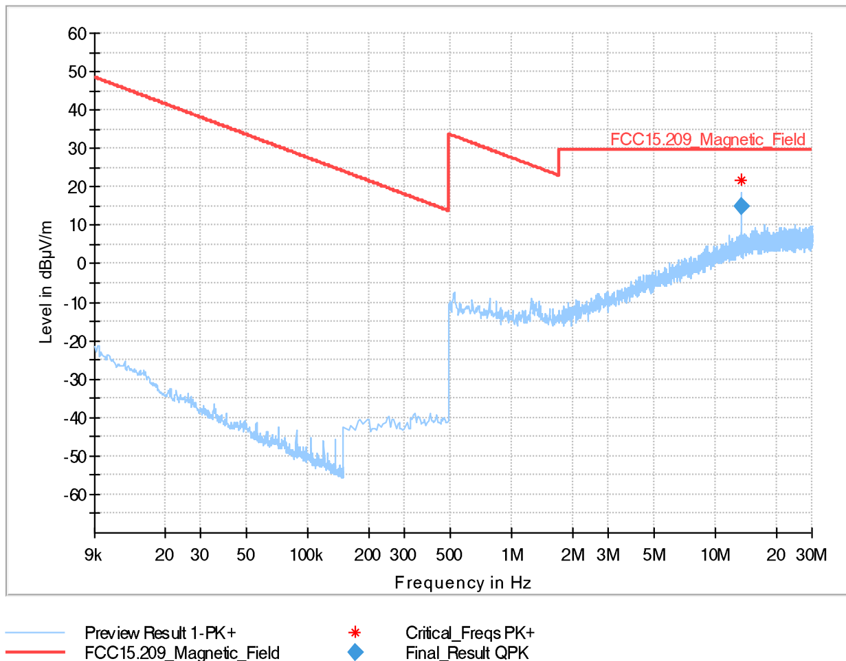
Plot 17: RSE 9 kHz – 30 MHz, OP 1, low channel, loop antenna
