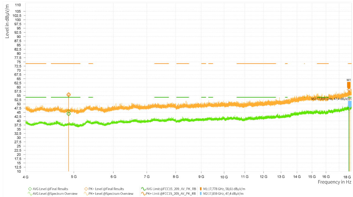
Plot 27: RSE 4 GHz – 18 GHz, OP 1, mid channel, horizontal / vertical polarisation
