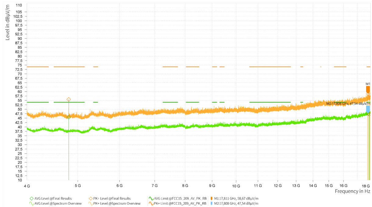
Plot 26: RSE 4 GHz – 18 GHz, OP 1, low channel, horizontal / vertical polarisation
