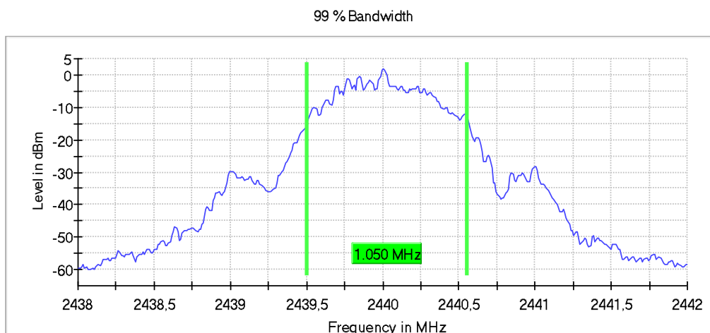
Plot 5: 99% Occupied Bandwidth, OP 1, mid channel
