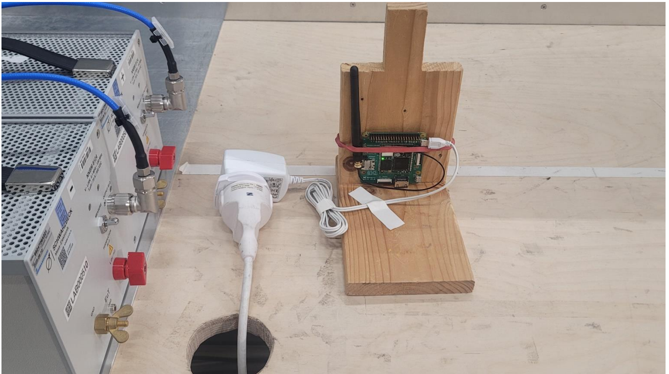
Photo No. 15: AC conducted emissions
