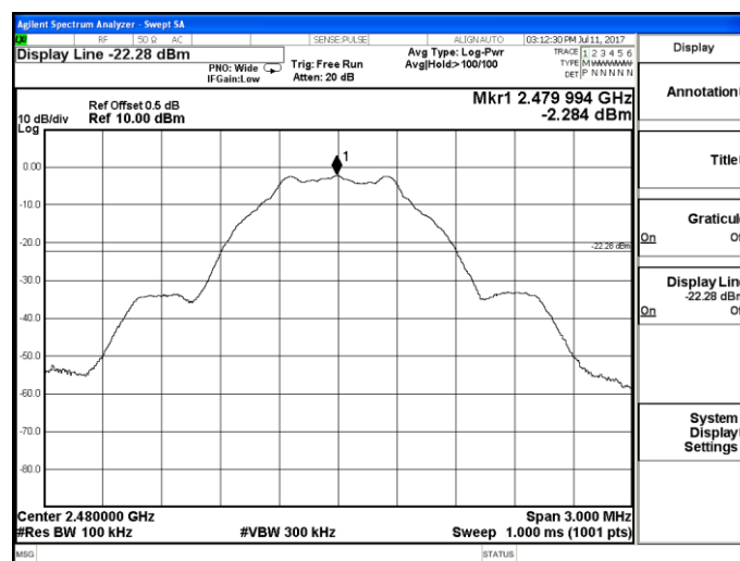
Channel 39 / 2480 MHz
