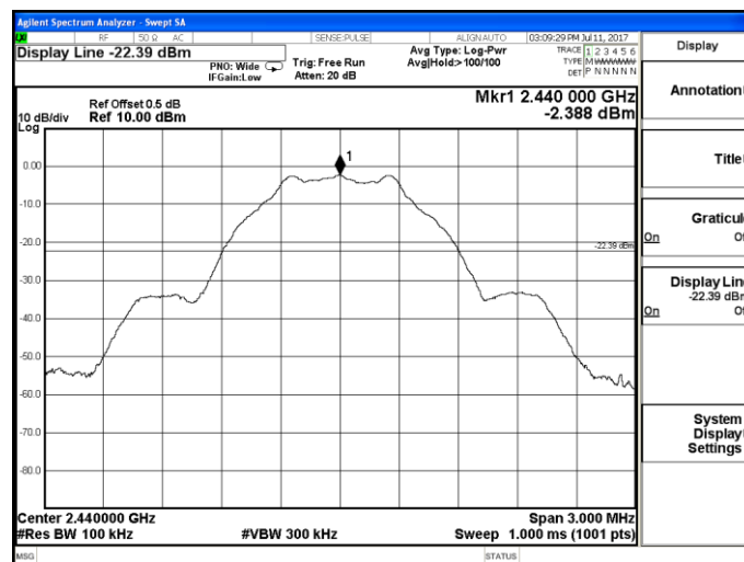
Channel 19 / 2440 MHz
