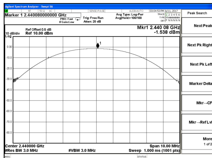
Channel 19 / 2440 MHz
