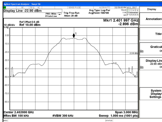
Channel 0 / 2402 MHz
