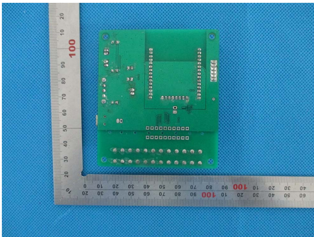
VIEW OF EUT-7 [Bottom side of evaluation board]
