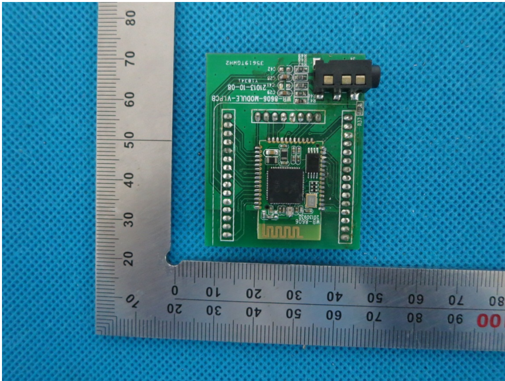
VIEW OF EUT-1 [RF Module fixed mounted on carrier board]
