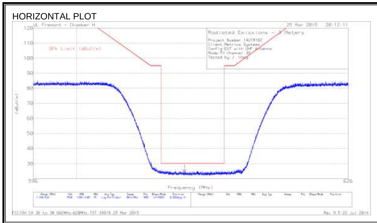
PLOT OF SPURIOUS EMISSIONS 602 TO 620 MHz (CHANNEL 39 - 623MHz)
