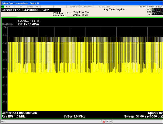
Number of Pulses in 31.6 seconds \pi/4 DQPSK_2-DH1
