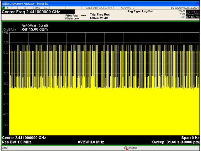
Number of Pulses in 31.6 seconds \pi/4 DQPSK_2-DH3
